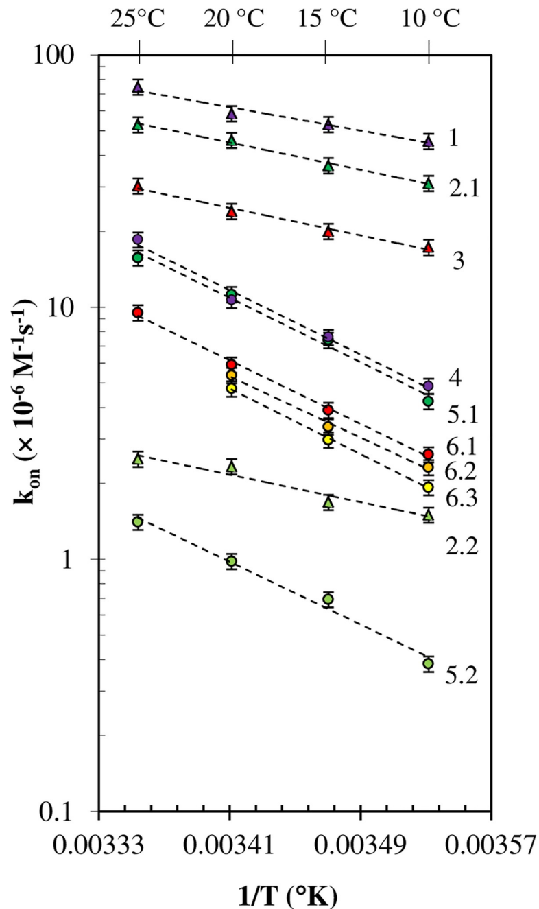
Fig 8. Arrhenius plot of the association rate constants. Temperature dependence of the B 7 association reaction at pH 8 (unless otherwise specified) for: 1 SAV-BFl (purple triangles); 2 SAV-B 7 -DNA ds *Fl (green triangles): 2.1 (k on1 ) and 2.2 (k on2 ); 3 SAV-BcO (red triangles); 4 AV-BFl (purple circles); 5 AV-B 7 -DNA ds *Fl (green circles): 5.1 (k on1 ) and 5.2 (k on2 ); 6 AV-BcO (red circles): 6.1 at pH 8, 6.2 at pH 9 (orange circles), 6.3 at pH 10 (yellow circles). The data points were plotted in semi-logarithm (ln k on vs 1/T) for clarity.
