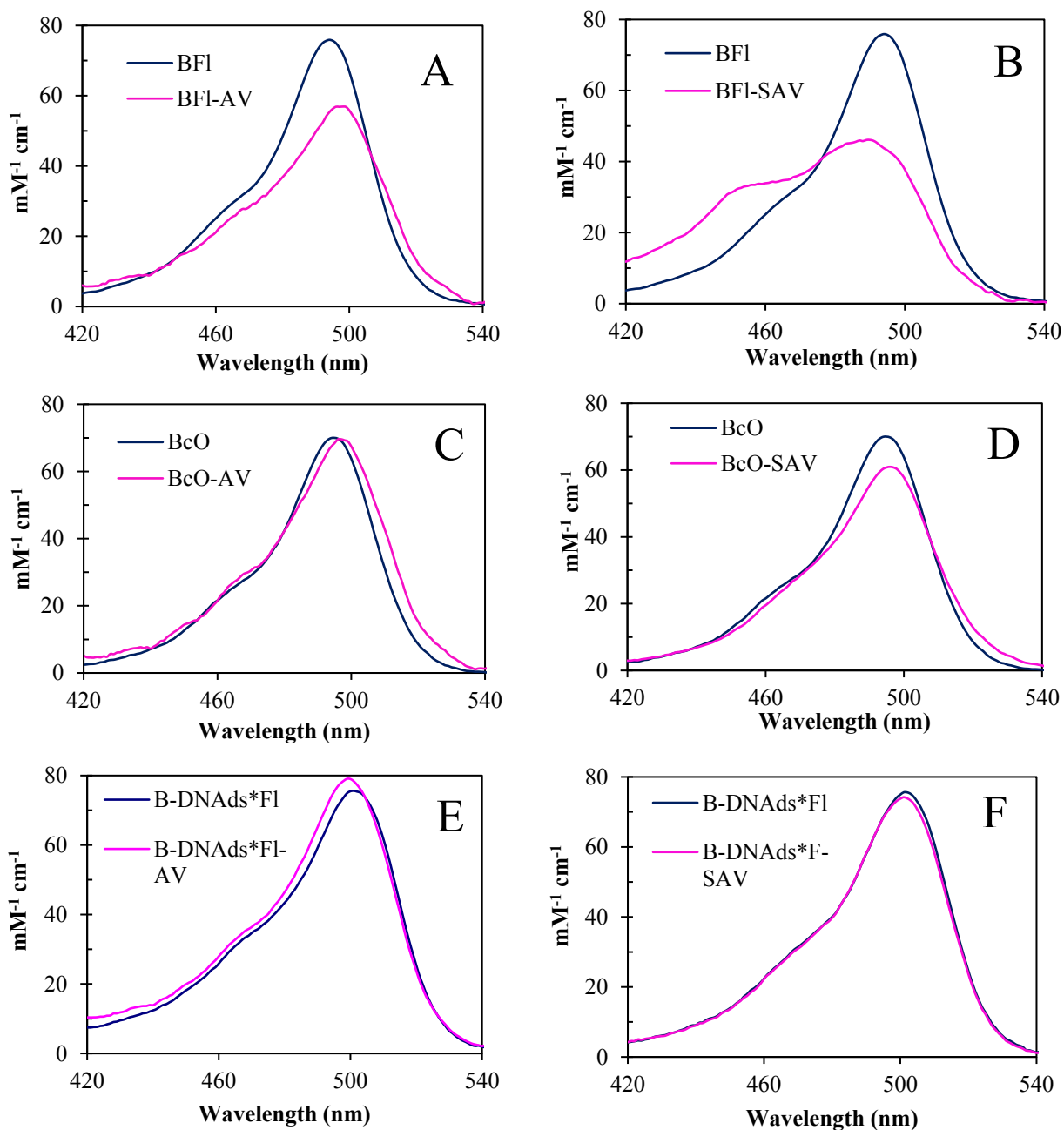
S1 Fig. Absorbance spectra of dye-labeled B 7 probes and respective complexes with AV and SAV. The absorbance spectra of the unbound BFI, BcO and B 7 -DNA 4s *FI are shown in dark blue and the respective bound complexes formed with SAV and AV in pink. The spectra are normalized to the calculated molar absorptivities. The distortion of the SAV-BFI absorbance spectrum (B panel) is caused by the presence of FI 2- and FI 1- . The labeled probes and protein concentrations were 1 μM and 10 μM, respectively.
