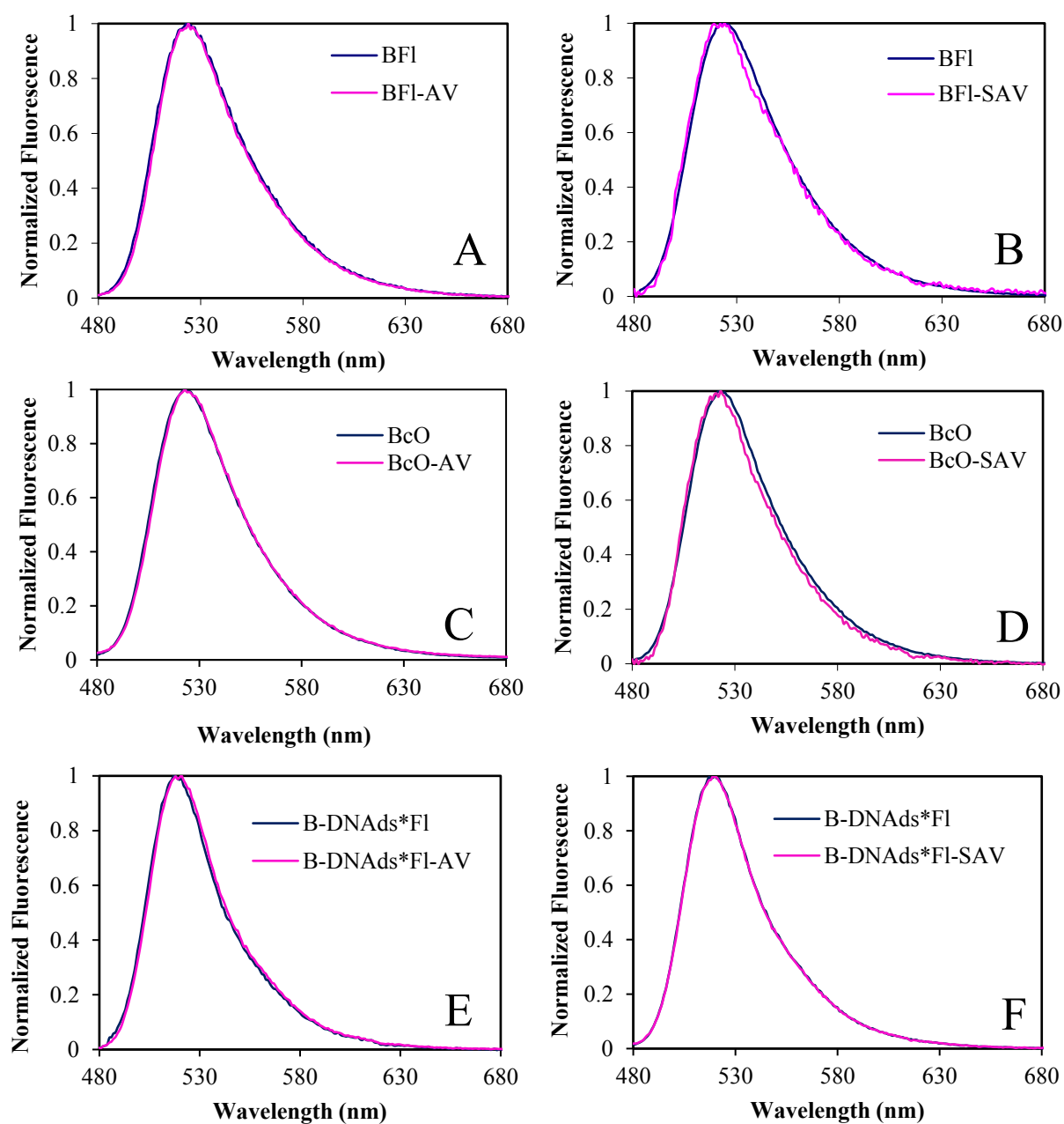
S2 Fig. Fluorescence emission spectra of dye-labeled B 7 and respective complexes with AV and SAV. The normalized spectra of the unbound BFl, BcO and B 7 -DNA ds *Fl are shown in blue and their respective bound complexes formed with SAV and AV in pink. The probe and protein concentrations were 20 nM and 1040 nM (AB 1 filling model), respectively.
