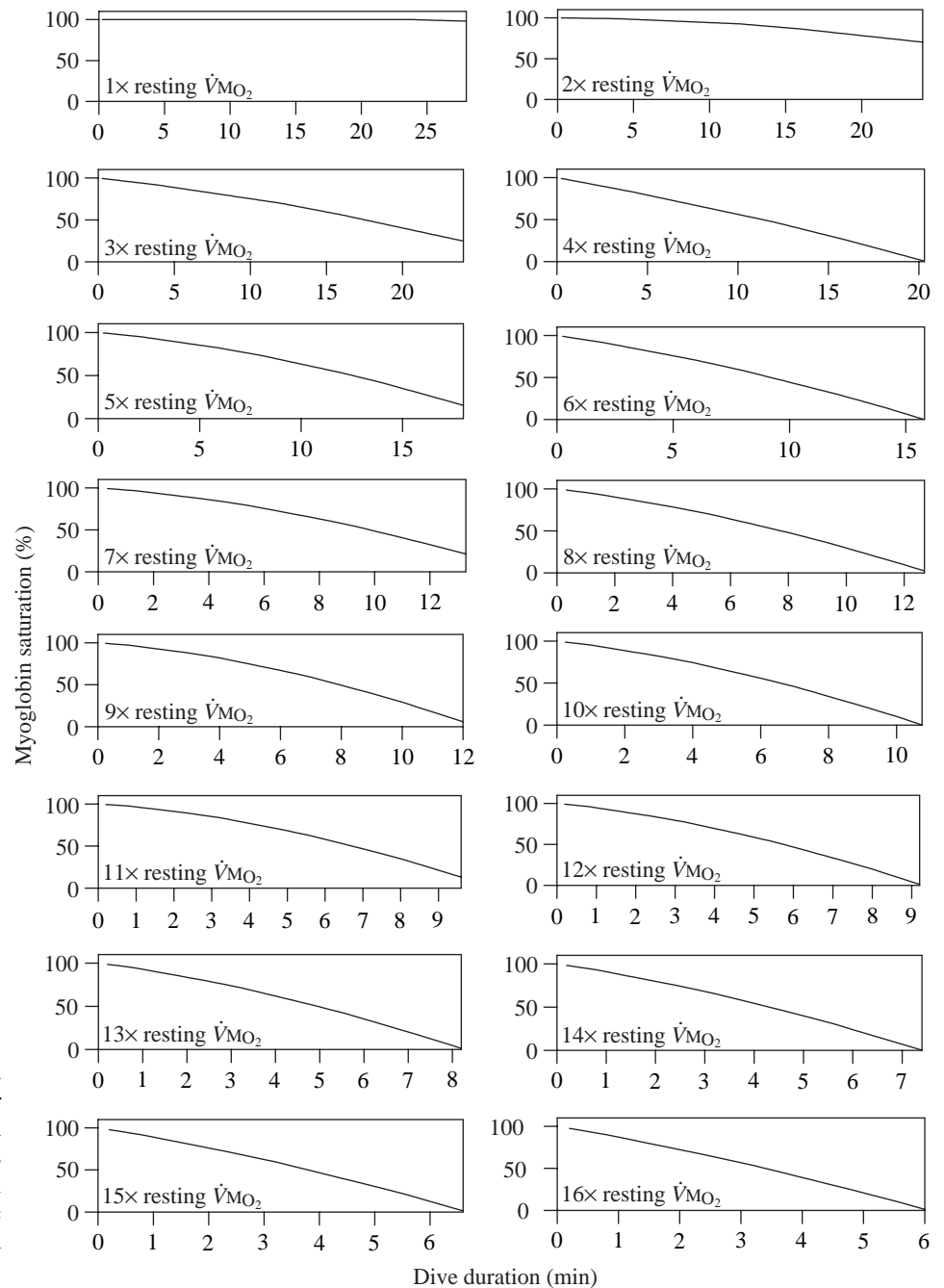
Fig. 11. Percentage oxymyoglobin saturation as a function of dive time for skeletal muscle oxygen consumption rates ( \dot{V}M_{O_2} ) ranging from 1 to 16 times the resting value. The abscissa of each plot is scaled to its respective aerobic dive limit (ADL) to give maximum resolution.
