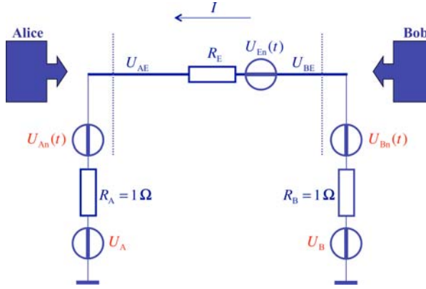
FIGURE 5. Outline of the situation encompassing correct physics represented by non-zero Johnson noise voltages of the resistors. The impacts of U_{A_n} and U_{B_n} are significant: for GAA’s absurdly limited Eve it provides non-perfect eavesdropping and a continuous change of the information leak when R_E converges to zero. Perfect eavesdropping can be achieved only after infinitely long time-averaging, which is unphysical.
