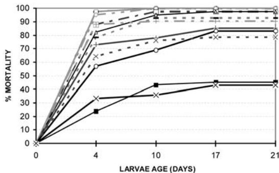
Fig. 1. Mortality of fall armyworm larvae (started as neonate larvae) confined on zoysiagrasses in no-choice laboratory experiments (14 replicates). Cultivars: —●— Cavalier, —□— Emerald, —◇— Belair, —□— Meyer, —△— K Com, —■— El Toro, —+— DALZ8501, —+— Diamond, —○— DALZ8508, —■— Crowne, —■— DALZ8516, —X— Palisades.
