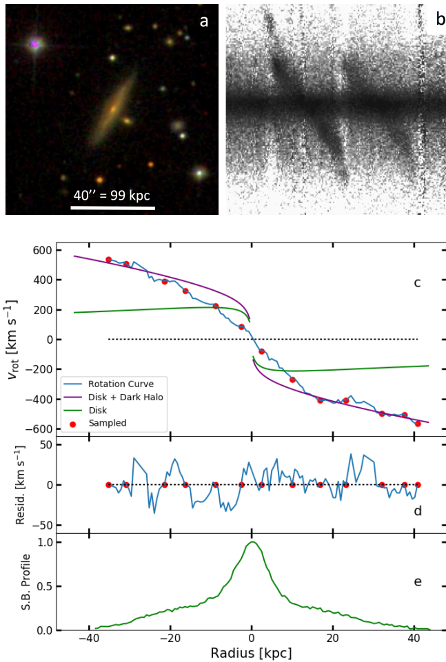
Figure 1. Fastest rotating super spiral 2MFGC 12344. a) SDSS g, r, i -band image. b) SALT RSS 2D spectrum of H\alpha and [N\ II]\ \lambda 6585 . c) Rotation curve (solid blue line, red points) with v_{\max} = 568 \pm 16\ \text{km s}^{-1} at r = 41\ \text{kpc} . The model (purple) includes a disk of stars and gas (green curve) following the observed galaxy surface brightness profile plus NFW dark-matter halo. d) Residuals to cubic spline fit, with standard deviation 16\ \text{km s}^{-1} . e) Galaxy continuum profile along the slit.
