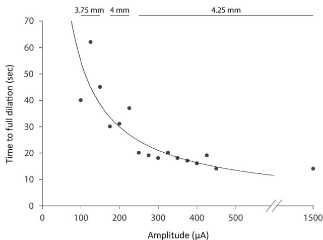
FIGURE 4. Relationship between stimulus amplitude and time to full pupil dilation. Stimulus parameters were 15 Hz, 100 \mu\text{s}/\text{phase} , and 25 to 1500 \mu\text{A} . Threshold amplitude was measured at 100 \mu\text{A} . The lines at the top of the chart indicate the pupil diameter when fully dilated, for each stimulus amplitude. Diameter at rest was 3.5 mm.
