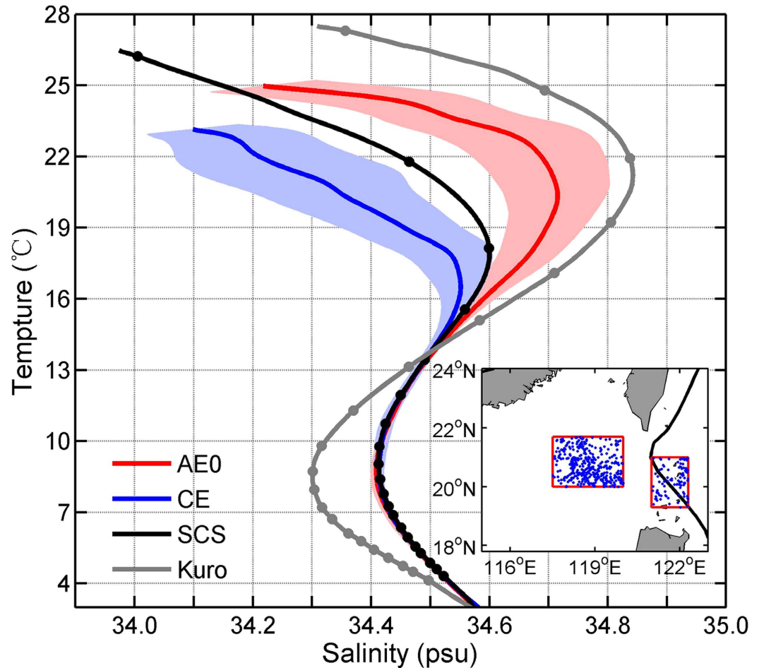
Figure 2. Mean T-S diagrams of water mass within and outside of the eddies. Red and blue lines show the results within AE0 and CE, respectively, obtained from the moored CTD observations (Supplementary Table S1). Shadings denote the standard deviations. The black and gray lines show the results of the northeastern SCS water and the Kuroshio water, respectively, computed based on historical Argo T/S profiles within the red boxes of the inset figure. The dots on the T-S diagrams indicate the depths of 50, 100, 150, 200 m, etc. Blue dots in the inset figure indicate Argo profiles' locations, and the black curve indicates the axis of the time-mean Kuroshio. Figure is plotted using MATLAB R2013a ( http://www.mathworks.com/ ). The map in the inset figure is generated by MATLAB R2013a with M_Map (a mapping package, http://www.eos.ubc.ca/~rich/map.html ).
