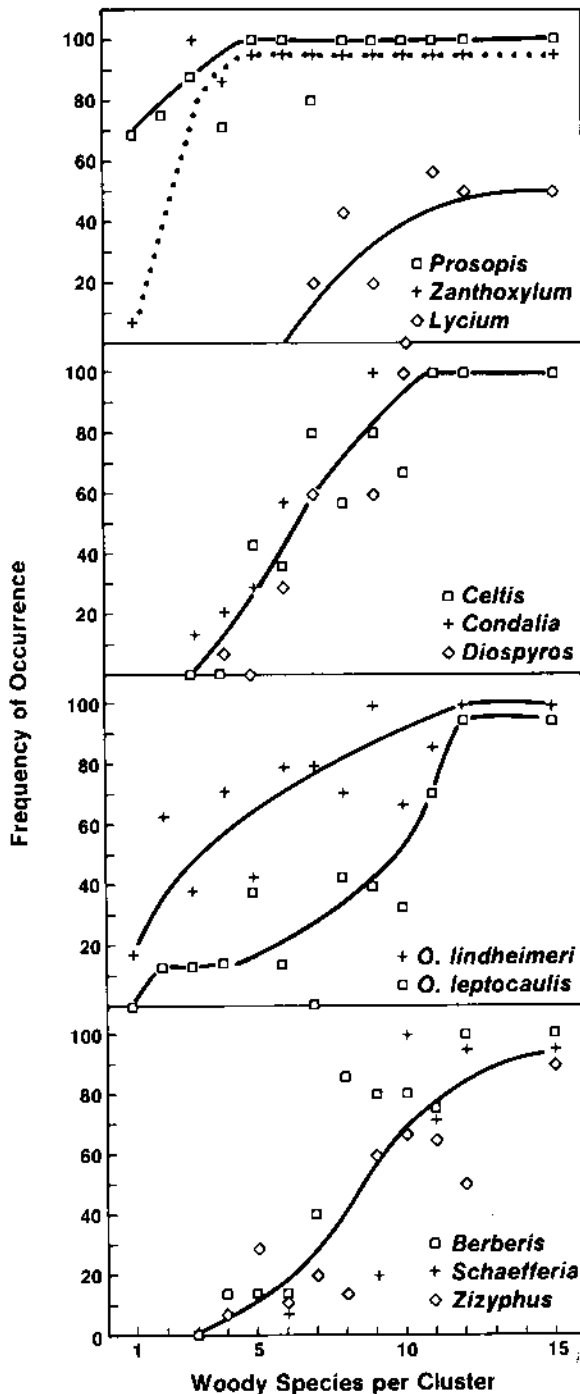
FIG. 3. Frequency of occurrence of woody species in clusters at varying stages of development. In cases where Prosopis was absent from clusters the remains of dead individuals were usually found. Curves were hand fitted.
