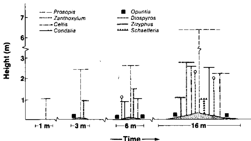
FIG. 10. Diagrammatic illustration of the chronosequential development of shrub clusters on fine loamy uplands in the Rio Grande Plains, Texas. These landscapes may be moving from the present two-phase configuration—discrete woody clusters scattered throughout the continuous grassland matrix—toward a monophasic woodland, as new clusters are initiated and existing clusters expand and coalesce.
