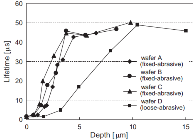
Figure 2.13 Minority carrier lifetime measured vs depth of damage layer removed from each side of the silicon wafer (plots of various polycrystalline wafers cut using SWC and DWC methods are shown) (Watanabe et al., 2010).
