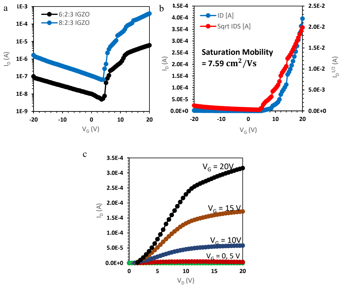
Figure 3.9 Shows (a) transfer characteristics of 6:2:3 and 8:2:3 IGZO devices, (b) mobility calculations and (c) output characteristics of the 8:2:3 IGZO device.
