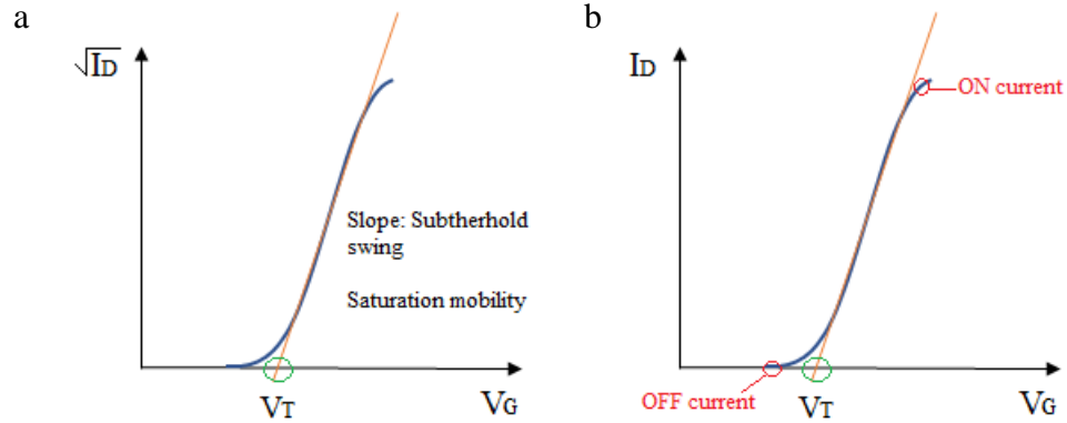
Figure 2.11 Transfer characteristics illustrating the extraction of threshold voltage, saturation transconductance from (a) square root of I_D vs V_G and ON/ OFF currents and linear transconductance from (b) I_D vs V_G .
