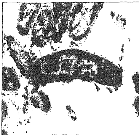
Figure 1 The Mycobacterium tuberculosis (X 90,000 by electron microscope)
