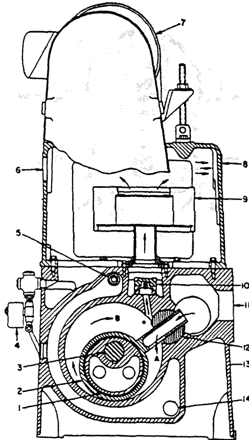
Figure 3.4 Schematic of a rotary piston pump: 1. eccentric; 2. piston; 3. shaft; 4. gas ballast; 5. colling water; 6. optional exhaust; 7. motor; 8. exhaust; 9. oil mist separator; 10. poppet valve; 11. inlet; 12. hing bar; 13 casing 14; cooling water.
