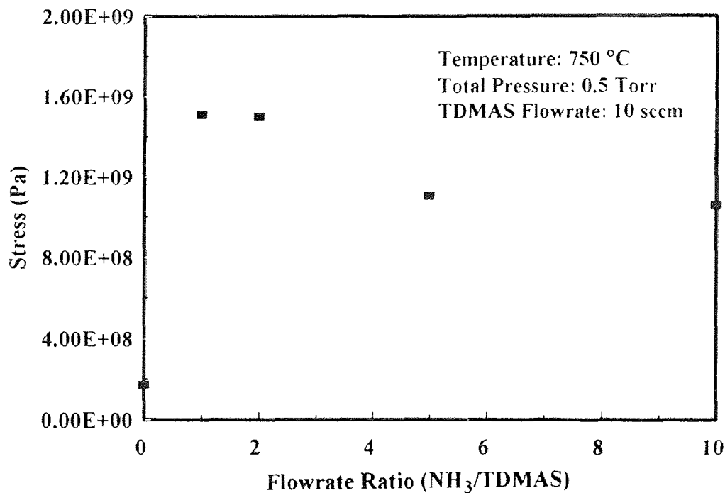
Figure 4.27 Variation of stress in silicon nitride films as a function of NH 3 /TDMAS flowrate ratio.
