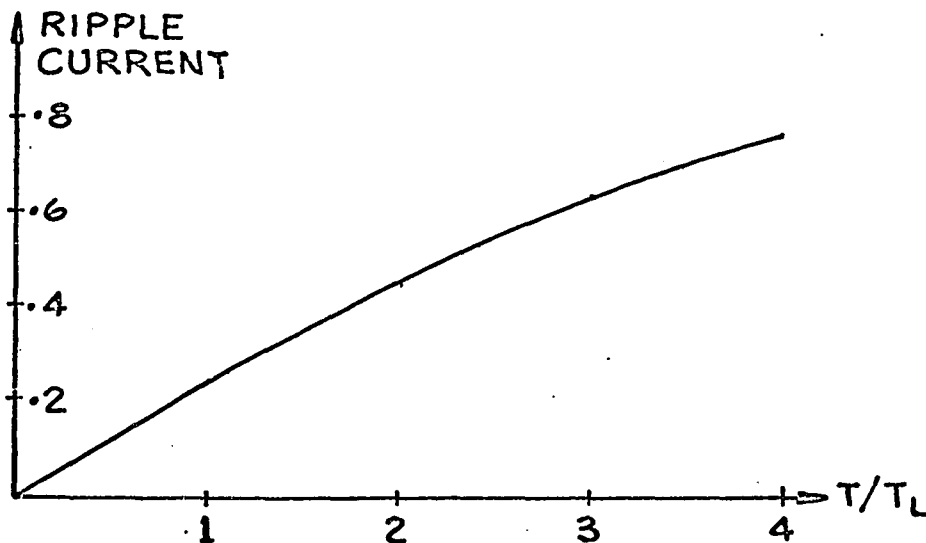
APP. 2.1 : PWM EXCITATION OF INDUCTIVE LOADS
