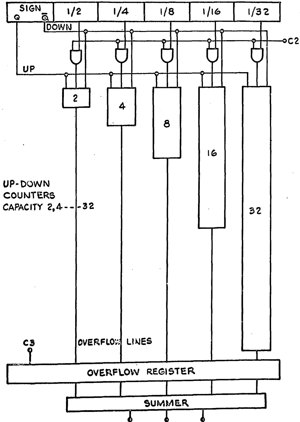
FIG.V.10: ALTERNATIVE IMPLEMENTATION OF THE RESET INTEGRATOR.
