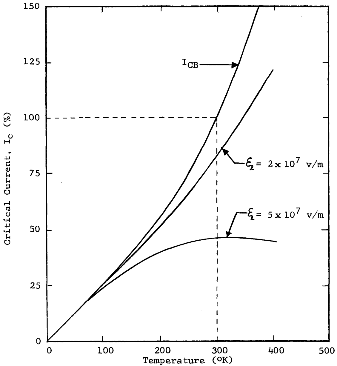
Figure 16.--The critical current to initiate pinching versus temperature for \mathcal{E}_1 negligible, \mathcal{E}_2 = 2 \times 10^7 \text{ v/m} and \mathcal{E}_2 = 5 \times 10^7 \text{ v/m} . I_{CB} calculated assuming electron and hole limiting velocities vary with temperature as electrons in germanium.
