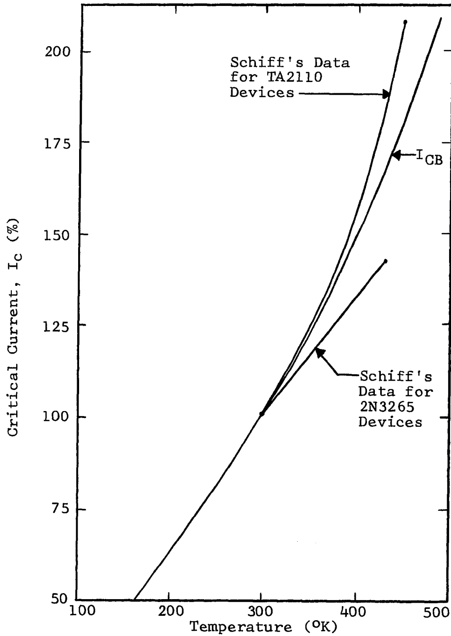
Figure 18.--Comparison of Schiff's data with the theoretical curve for I_{CB} for silicon. Data and theoretical curve adjusted to 100% at 300^{\circ}\text{K} .
