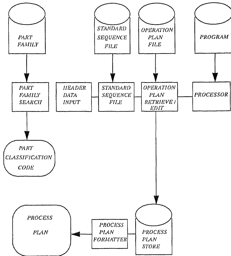
Figure 2.4: CAPP System: Flow diagram
