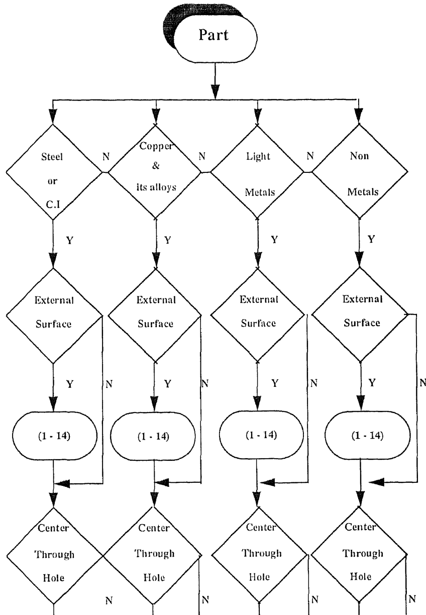
Figure 3.2: Flow diagram of operation logic
