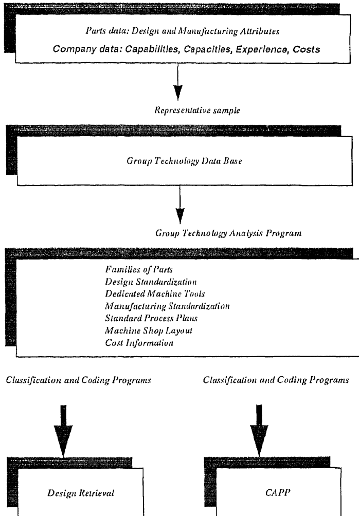
Fig. 2.5: Flow diagram of the MIPLAN system
