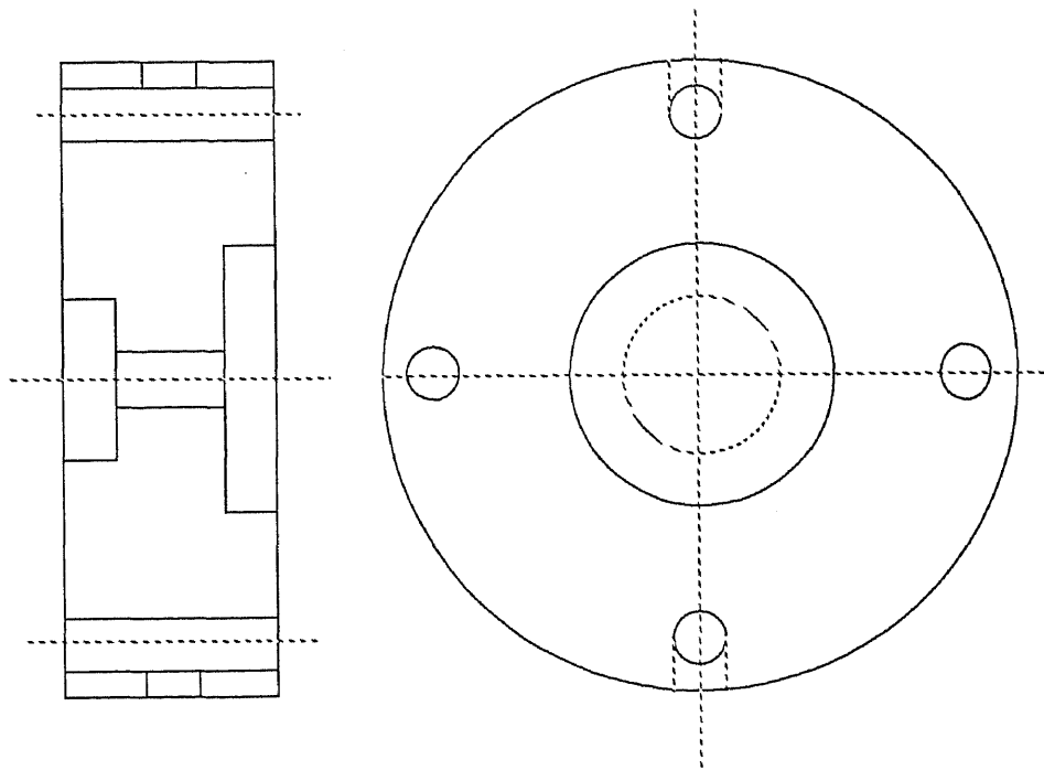
Fig. 3.3: Part for illustration: Sleeve
