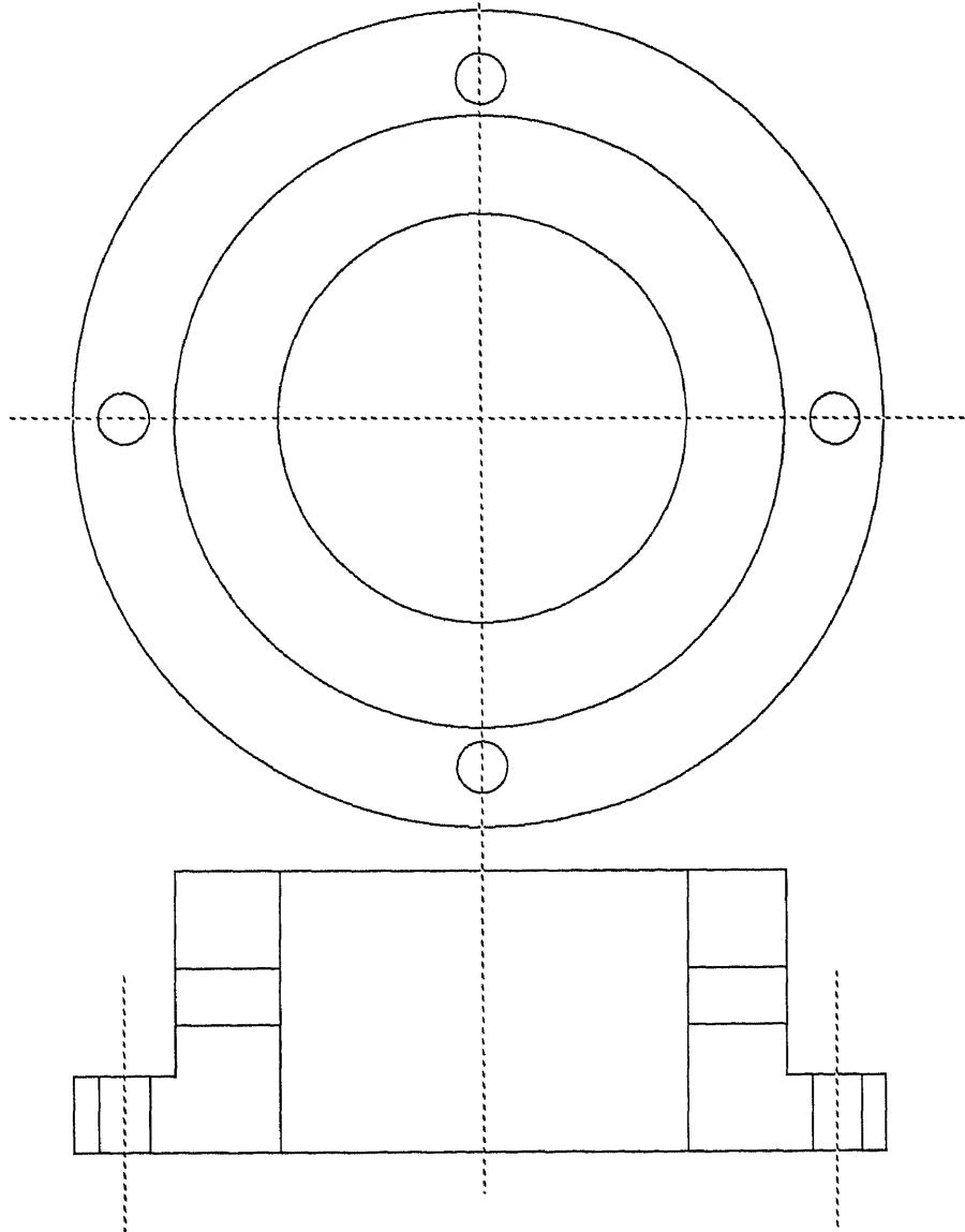
Figure 3.4: part for illustration: Bushing
