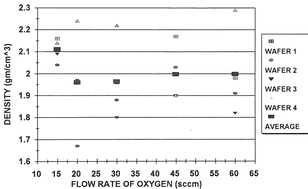
Figure 5.13 Variation of Density of the SiO 2 Deposits with Flow Rate of Oxygen
