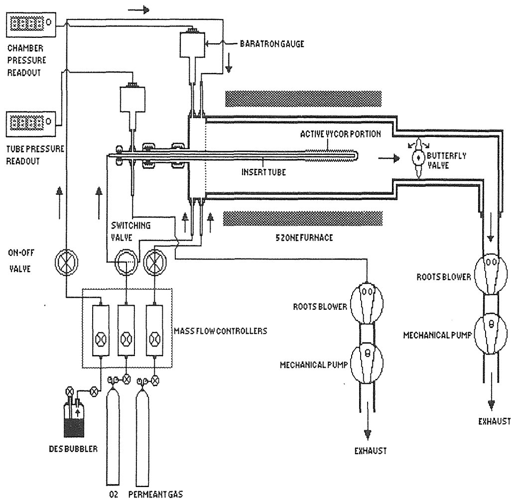
Figure 4.7 Schematic Diagram of the LPCVD Set-up for Membrane Synthesis and In-situ Permeability Measurements
