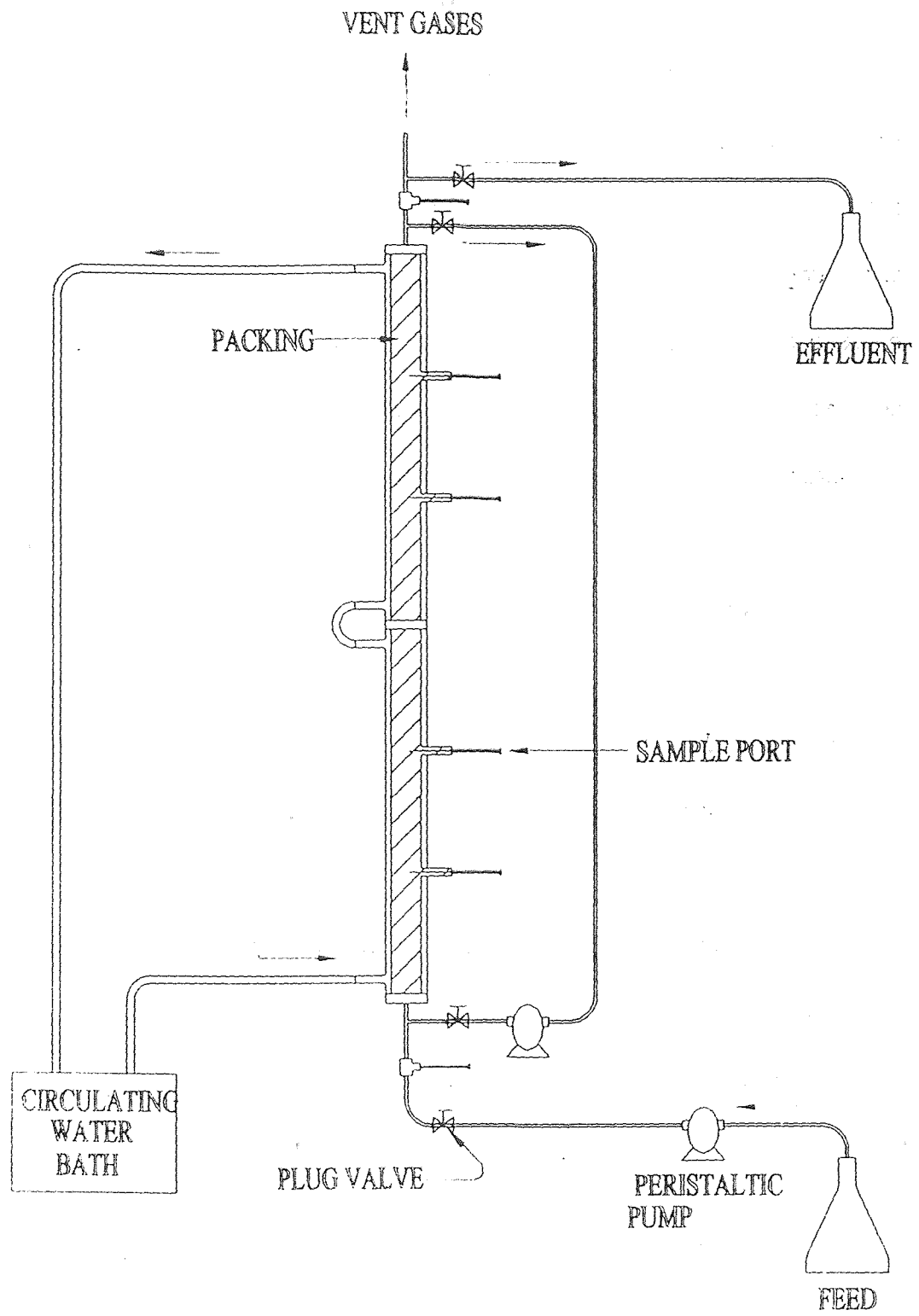
Figure 1: Reactor Set-Up
