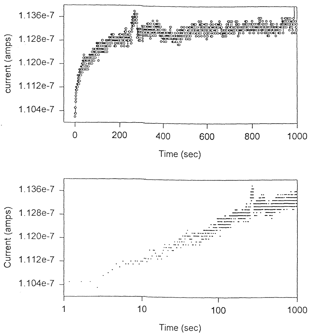
Fig. 4.2.1 Positive charging at V_g=2.1 V for a 2.8 nm oxide device
