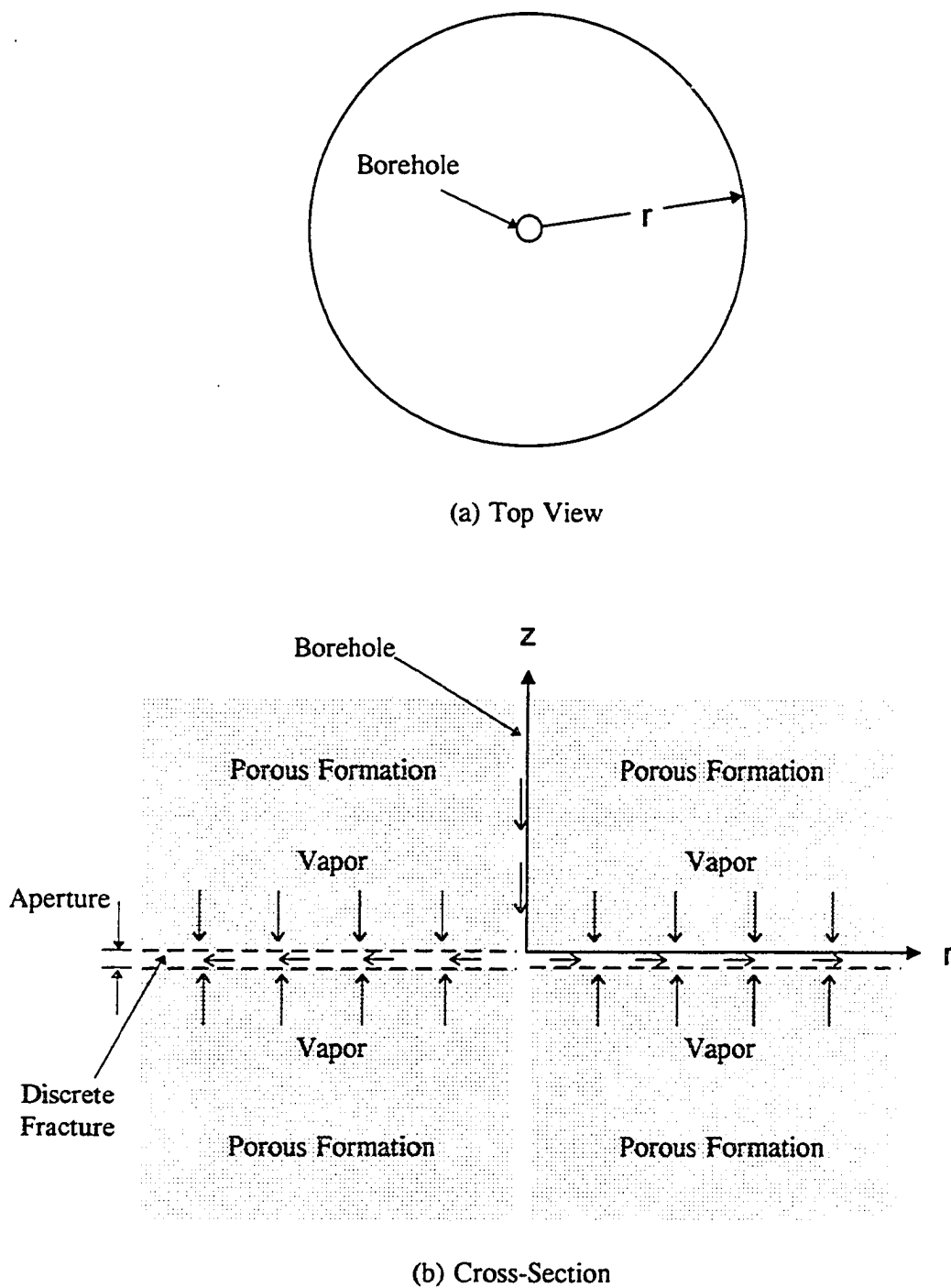
Figure 3.5 Conceptual Model of Chemical Transport for Axial Symmetrical Analysis
