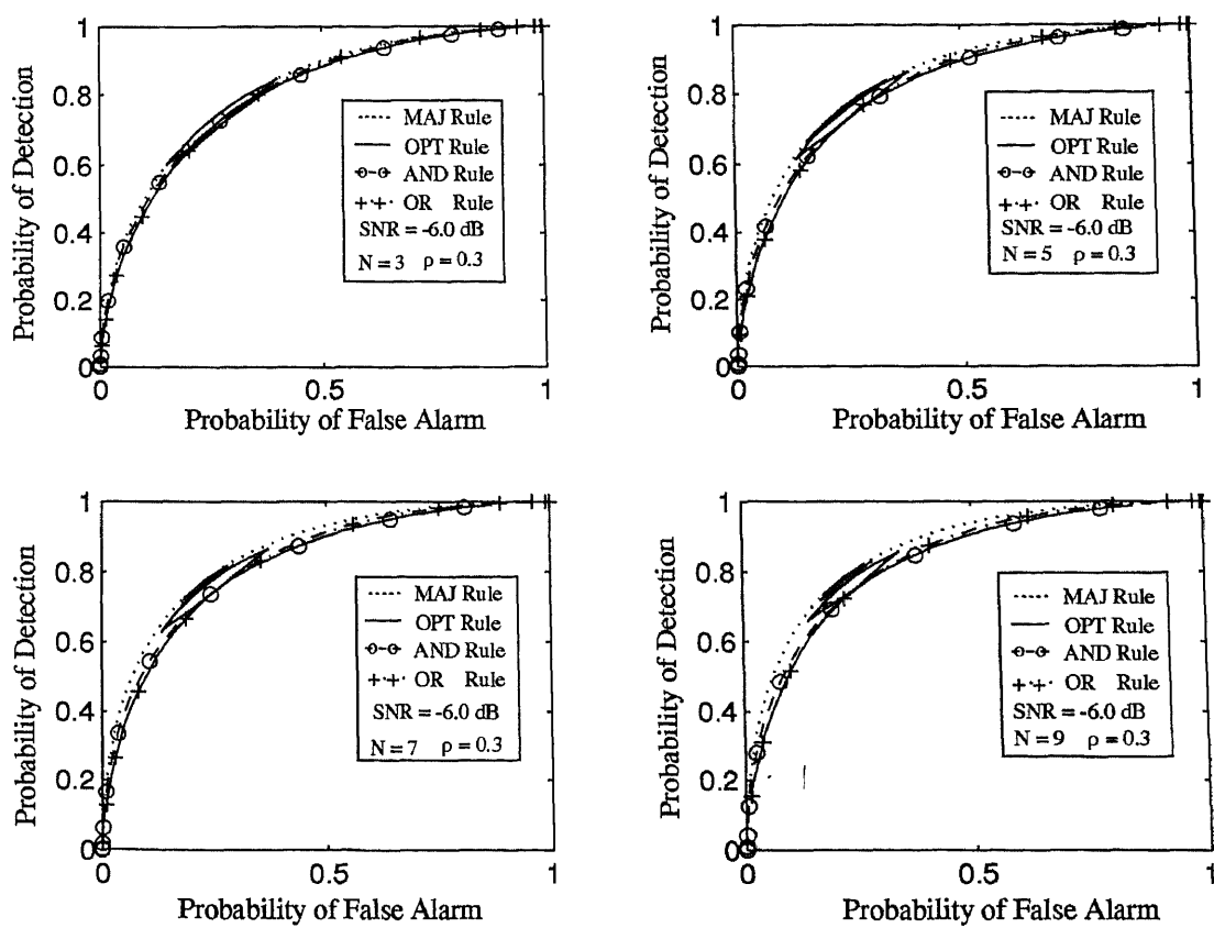
Figure 5.5 The ROC for the correlated case with different N when \text{SNR} = -6.0\text{dB} .
