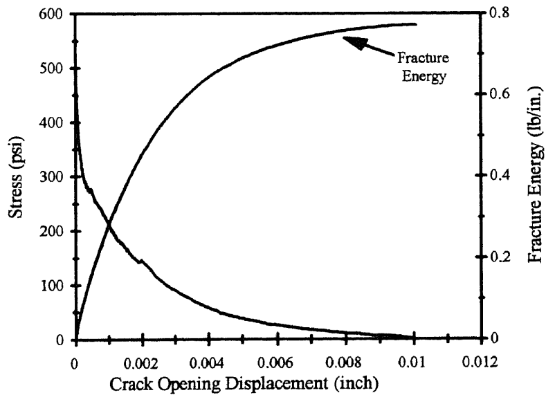
Figure B.6b Stress - Separation Curve and Fracture Energy for HSC-B (Specimen B6)
