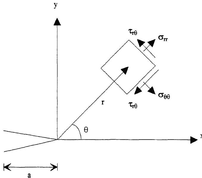
Figure 2.1 Stress State Close to the Crack Tip
