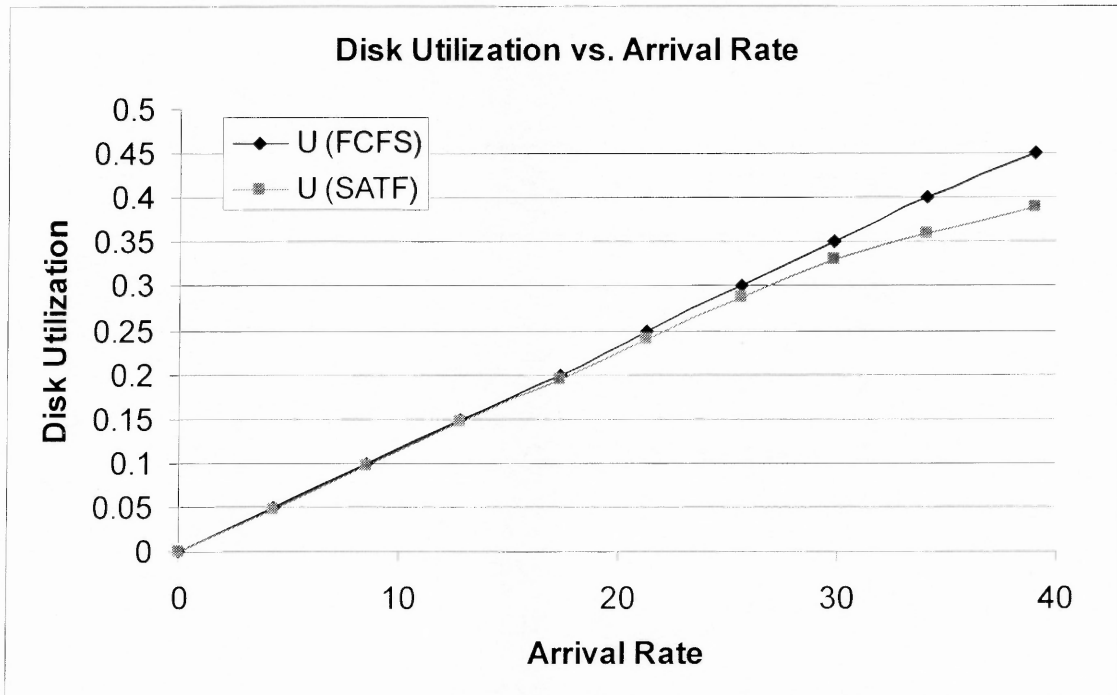
Figure 2.3 Disk utilization for a RAID5 system at different arrival rates with FCFS and SATF (N = 21).
