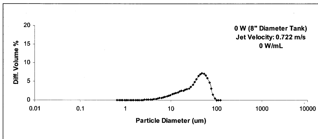
Figure A.1-2 Particle size distribution of experiment without sonication, Exp. 23, LS 5
