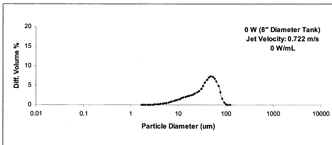
Figure A.1-3 Particle size distribution of experiment without sonication, Exp. 23, LS 7
