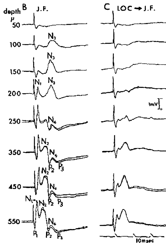
Figure 1.7 The results of Eccles et al experiments showing the mossy fiber field potential at varying depths. The P 1 , N 1 , N 2 , N 2 , P 2 , N 4 , and P 3 waves are marked for each depth. [Eccles, J. C., Sasaki, K., Strata, P., "Interpretation of the potential fields generated in the cerebellar cortex by a mossy fiber volley," Experimental Brain Research , vol. 3, pp. 58-80, 1967]
