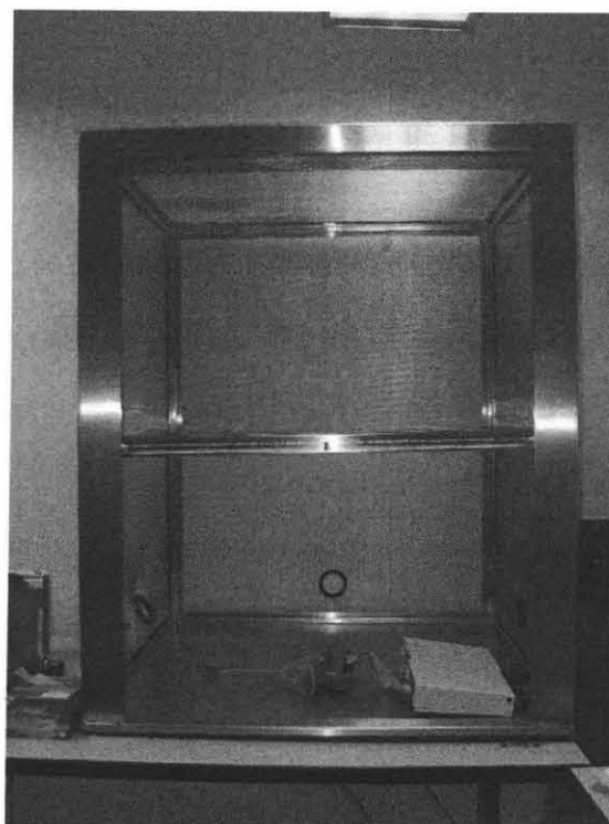
Figure 2.6 Faraday cage used to reduce noise.
