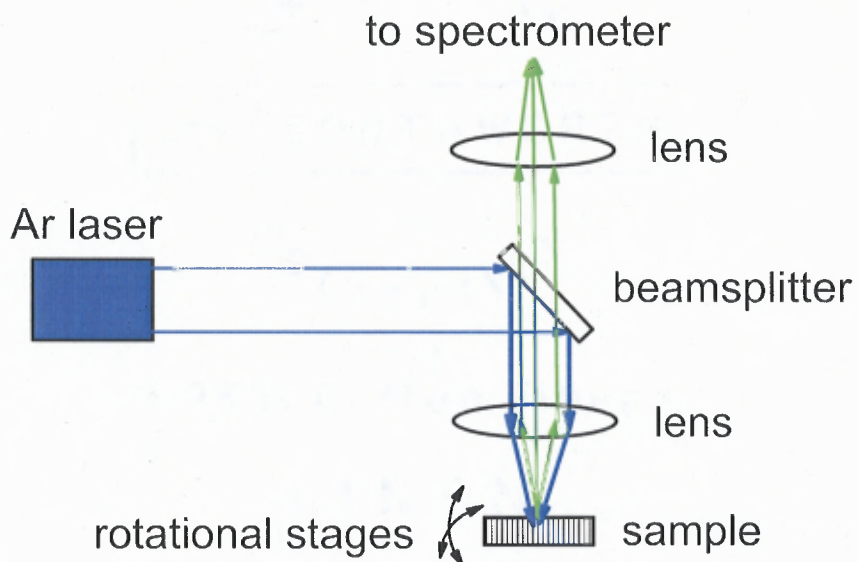
Figure 3.7 System configuration: the pump light (Ar at 488 nm or 514.5nm) is focused onto the sample which is placed on a rotational stage. The fluorescence signal is collimated and focused onto the spectrometer slit. A PMT is used to detect the signal and a cut-off filter is used to eliminate the laser line from the spectra.
