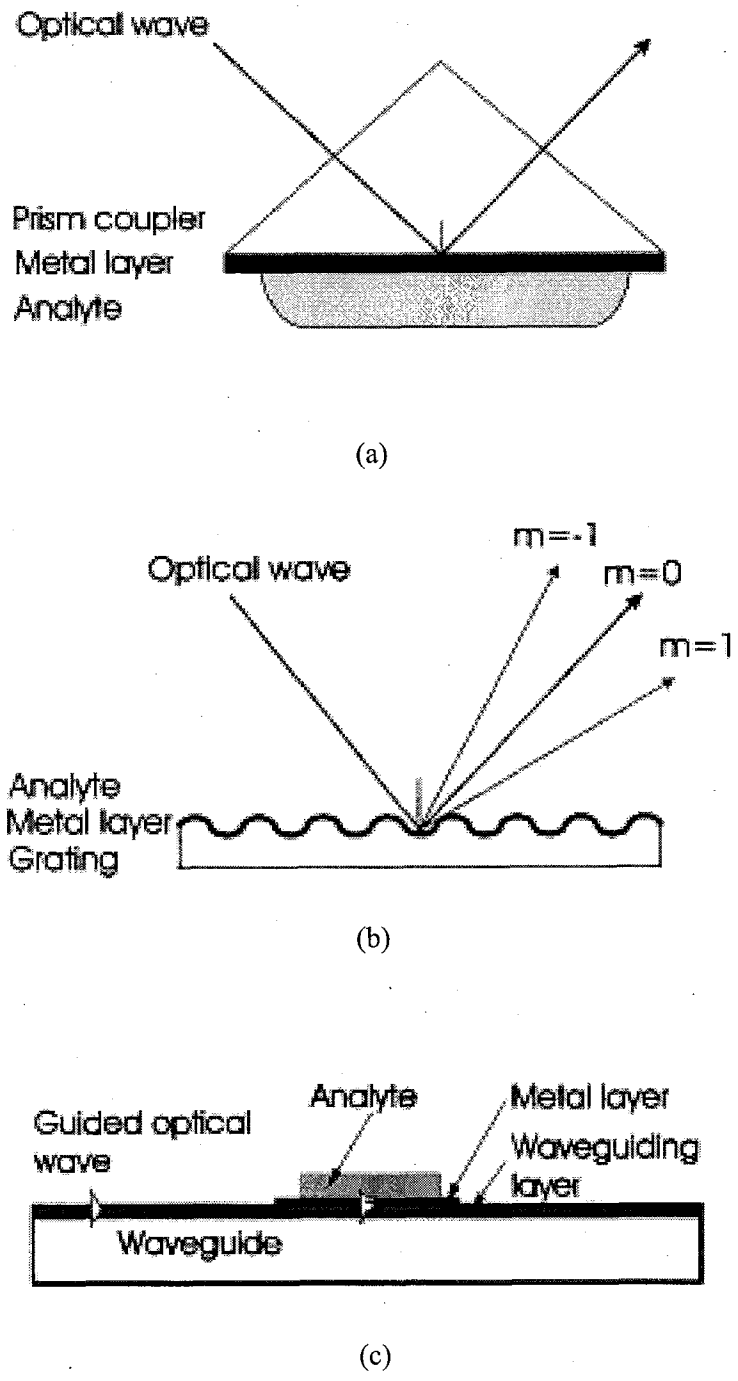
Figure 1.2 Most widely used configurations of SPR sensors: (a) prism coupler-based SPR system; (b) grating coupler-based SPR system; and (c) optical waveguide-based SPR system.
