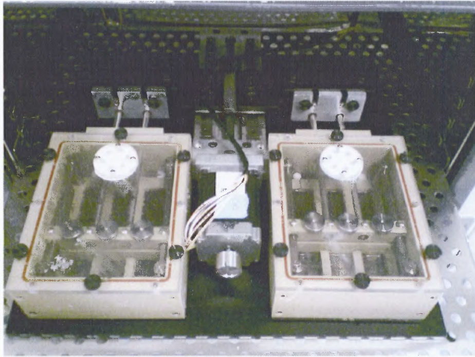
Figure 3.1 Stretch-growth bioreactors developed at the University of Pennsylvania.
