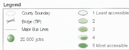
Figure H3. Output of model BD1011SO113
