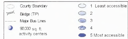
Figure H34. Output of model QL1012
