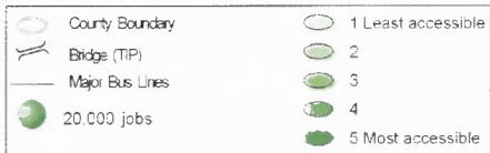
Figure H7. Output of model BD1O12SO121
