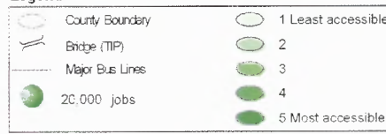
Figure H6. Output of model BD1O11
