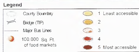
Figure H15. Output of model MA1011SO111
