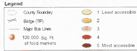
Figure H16. Output of model MA1011SO112
