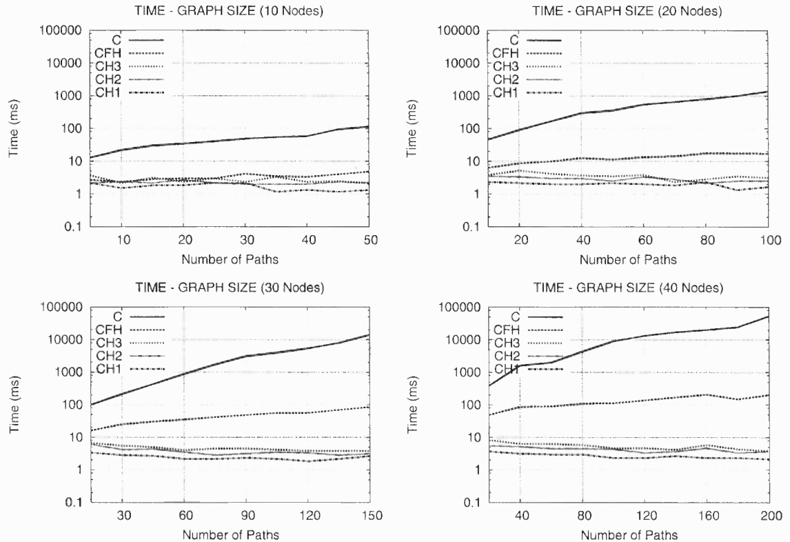
Figure 4.11 Execution time for checking PTPQ containment varying the number of root-to-leaf paths for 10, 20, 30 and 40 nodes in the dimension graph.
