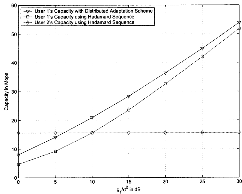
Figure 5.13 Users' individual capacity of 2-user system, when user 1 tries to maximize its capacity and user 2 tries to optimize its MSE.
