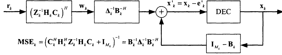
Figure 3.4 Successive interference cancelation structure at mobile k .
