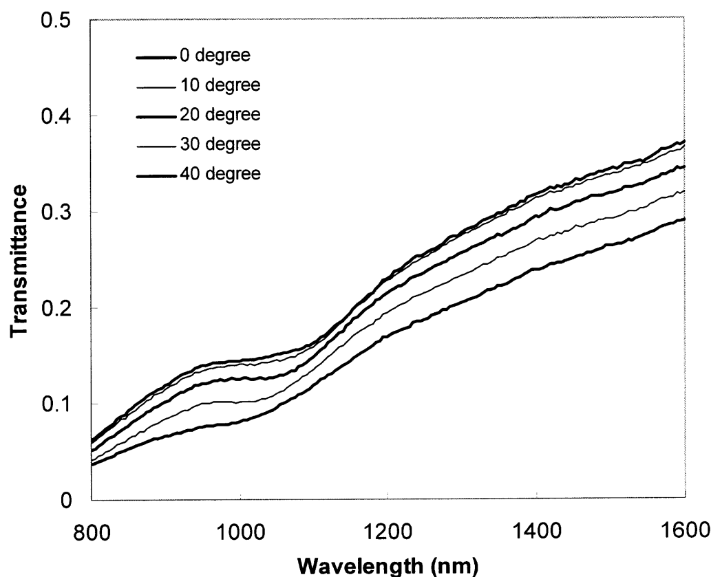
Figure 3.16 Transmission spectra of 503nm opal template embedded with SWCNT measured at different incident angles. From top to bottom, the curves corresponding to incident angle at 0°, 10°, 20°, 30°, and 40°.
