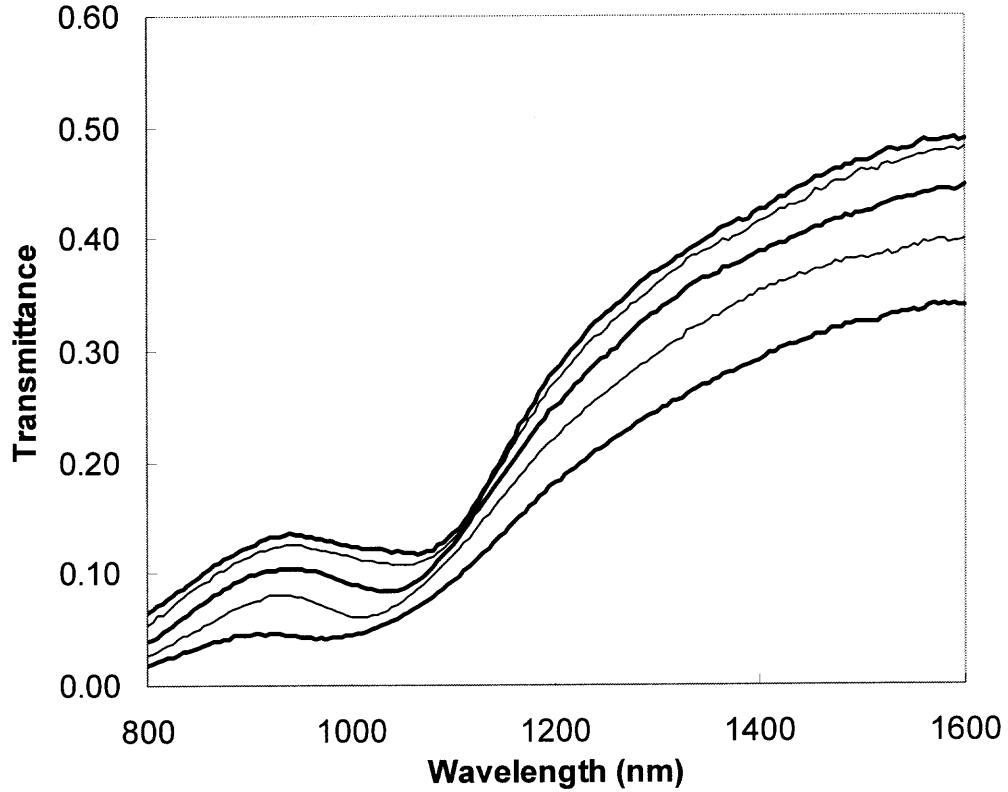
Figure 3.6 Optical transmission spectra recorded at different incident angles from opal with spherical diameter 503 nm. From top to bottom, each curve corresponding to incident angle of 0^\circ , 10^\circ , 20^\circ , 30^\circ , and 40^\circ .
