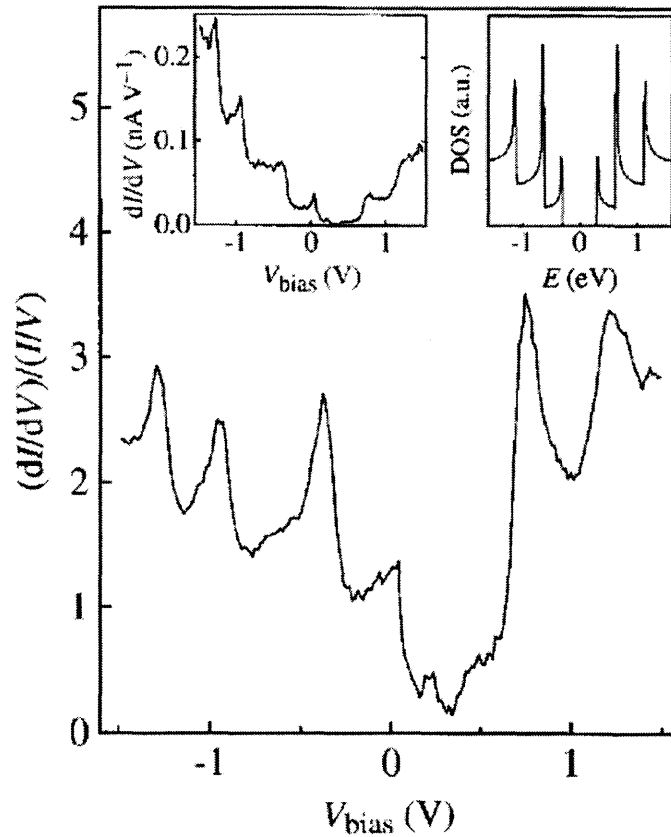
Figure 1.12 (dI/dV)/(I/V) , which is a measure of the DOS, versus V for single-wall carbon nanotubes [68]. The asymmetric peaks correspond to singularities at the onsets of 1-D energy bands of carbon nanotubes. The left inset displays the dI/dV data. The right inset displays a typical example of the spike-like DOS for a semiconducting tube.
