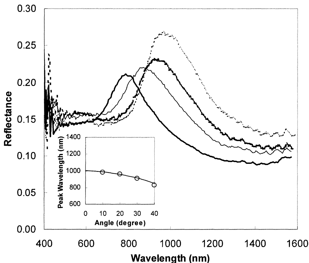
Figure 3.32 Optical reflection spectrum of PMMA–SWCNT inverse opaline structure. From left to right, each curve corresponding to incident angle 40°, 30°, 20°, and 10°. The inset image shows the angular dependency of reflection peak position. Hollow circular marks represent experimental peak wavelength measured at different incident angle; the solid line represents the theoretical function of Bragg law (Equation 2.10).
