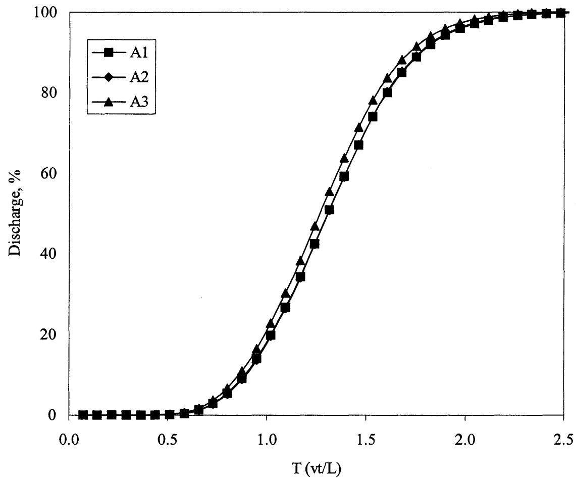
Figure 3.6 Discharge Profile Comparison for Peclet Number P=25 .
