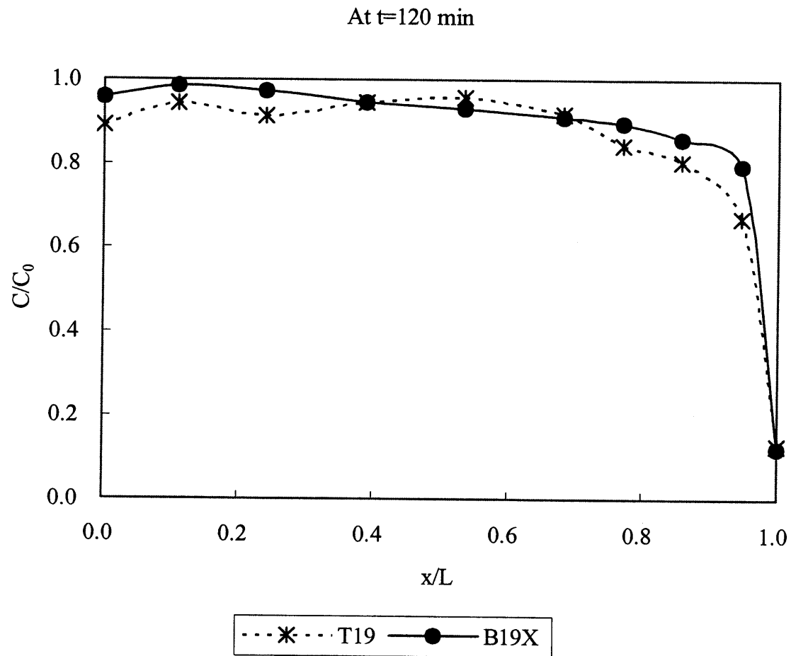
Figure 4.32 Contaminant Distribution for Case T19.
