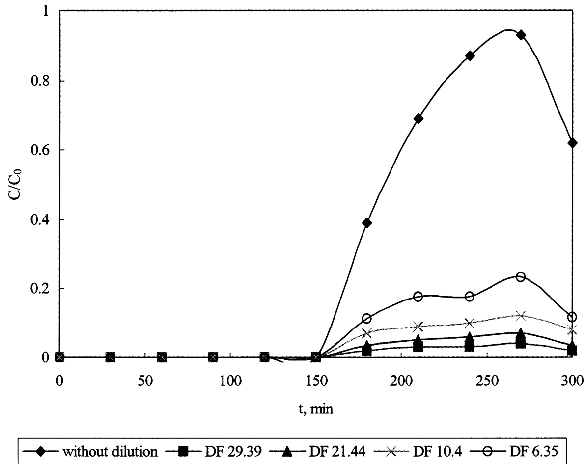
Figure 4.18 Contaminant Concentration Varies over Time in the Discharge Chamber Showing Lower Concentration Resulted from Dilution and Mixing.
