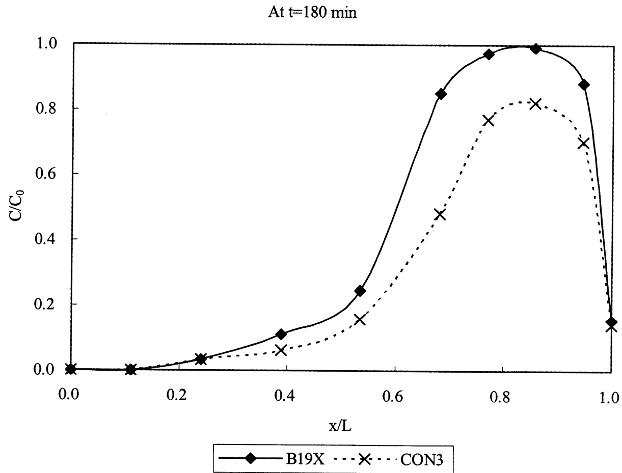
Figure 4.37 Contaminant Distribution for Case CON3 (Continued).
