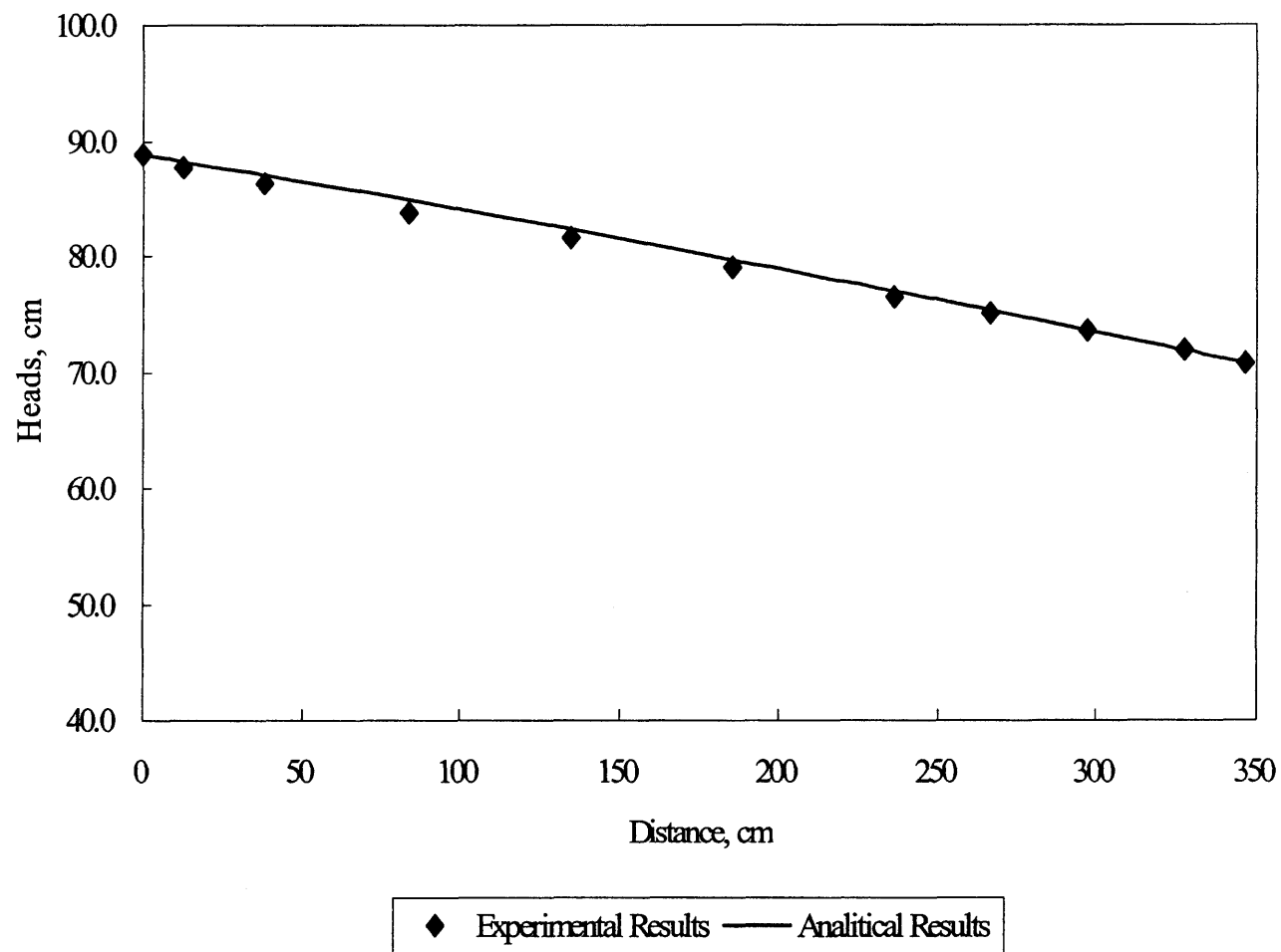
Figure 4.3 Experimental Results in Unconfined Situation-Hydraulic Heads.
