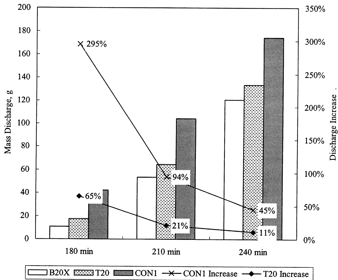
Figure 4.47 Contaminant Discharge Comparison.
