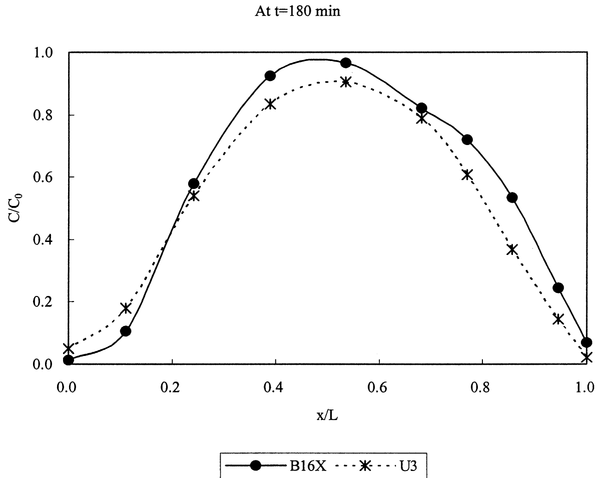
Figure 4.29 Contaminant Distribution for Case U3.
