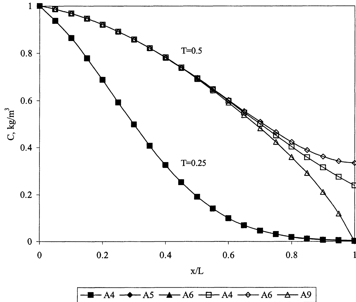
Figure 3.5 Concentration Profile Comparison for Peclet Number P=5 .
