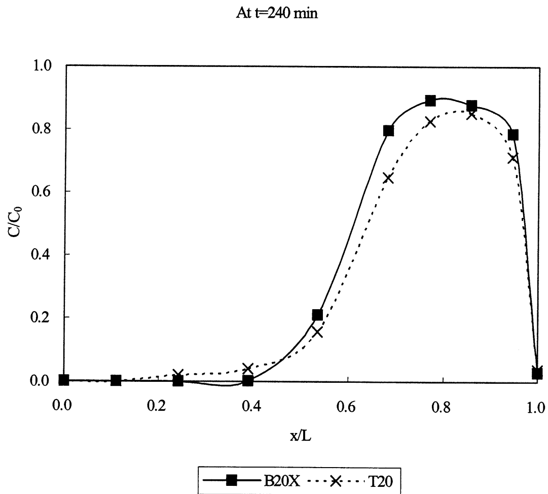
Figure 4.40 Contaminant Distribution for Case T20 (Continued).
