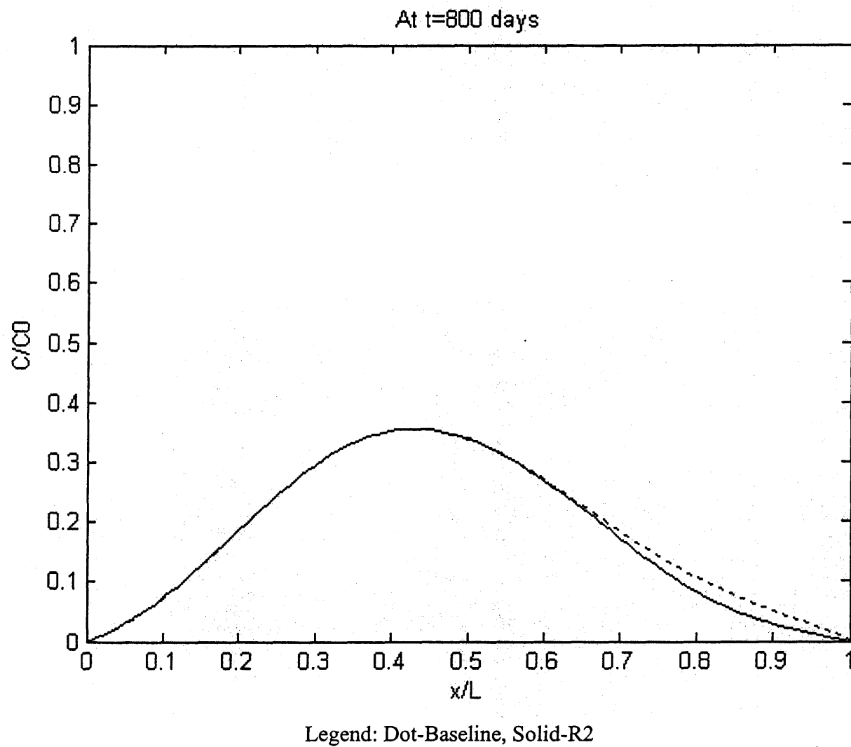
Figure 5.13 Tidal Effect on Contaminant Distribution at Stage I (Continued).
