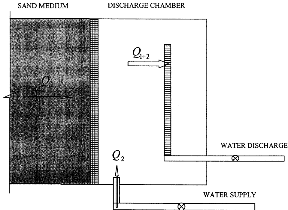
Figure 4.17 Dilution and Mixing in the Effluent Chamber Simulating Coastal Boundary Condition.
