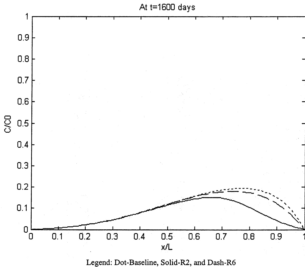
Figure 5.31 Tidal Effect on Contaminant Distribution (Continued).
