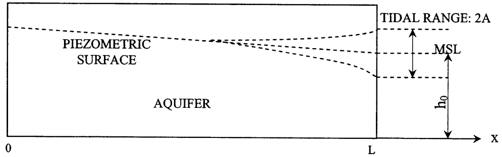
Figure 3.2 Groundwater Level Fluctuations Induced by Tides.
