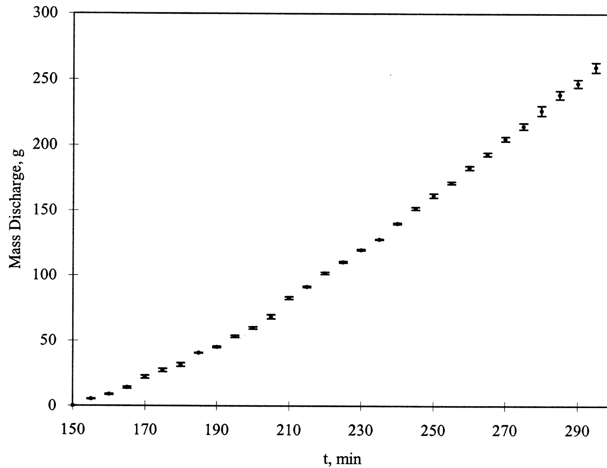
Figure 4.8 Experimental Repeating Tests for Case T16.
