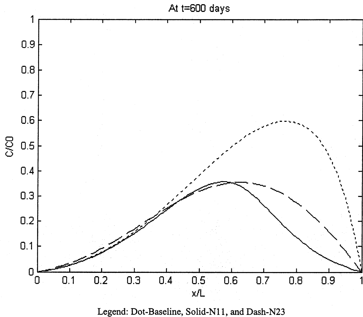
Figure 5.28 Tidal Effect on Contaminant Distribution (Continued).
