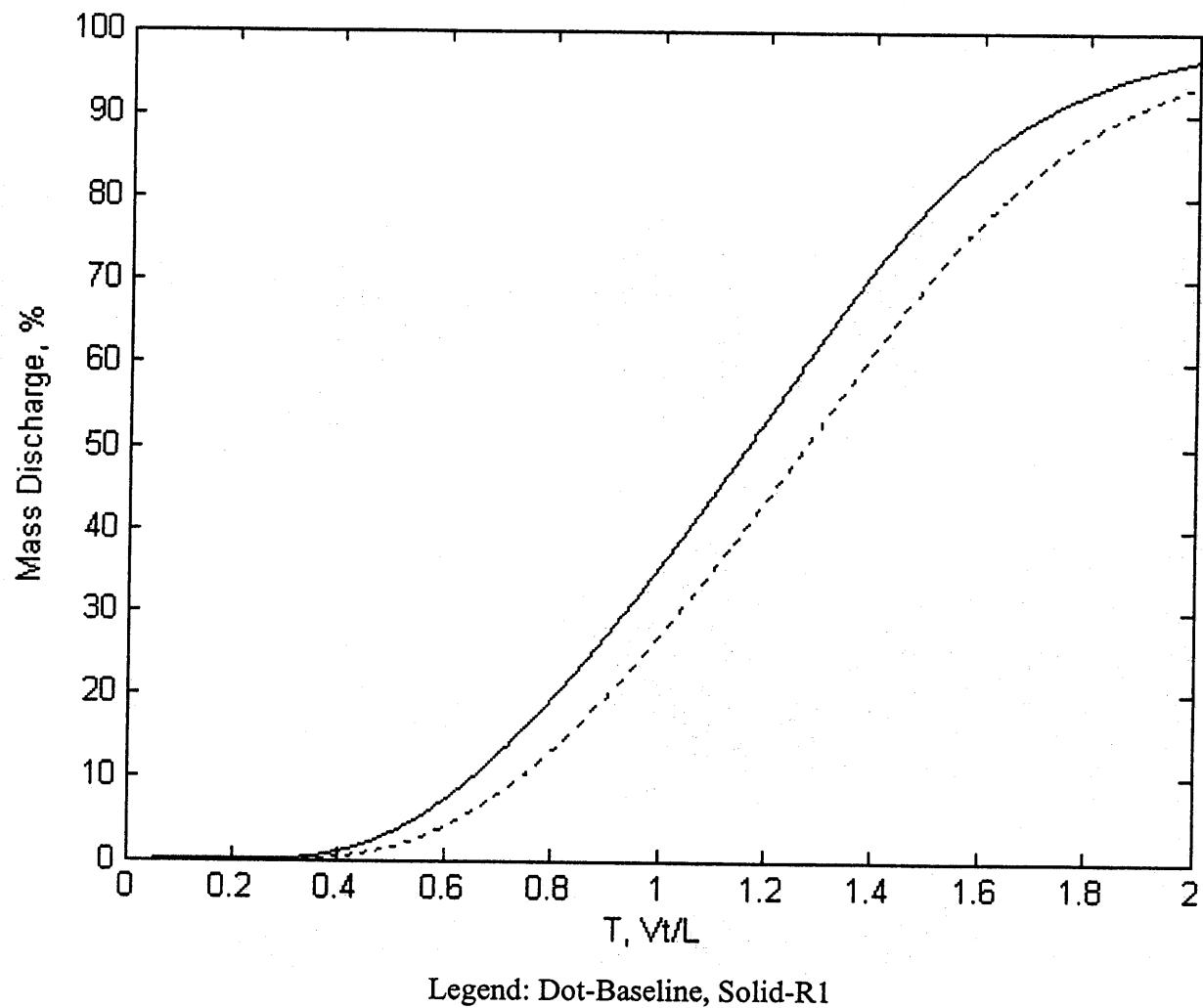
Figure 5.14 Tidal Effect on Contaminant Discharge subject to Different Retardation Factors.
