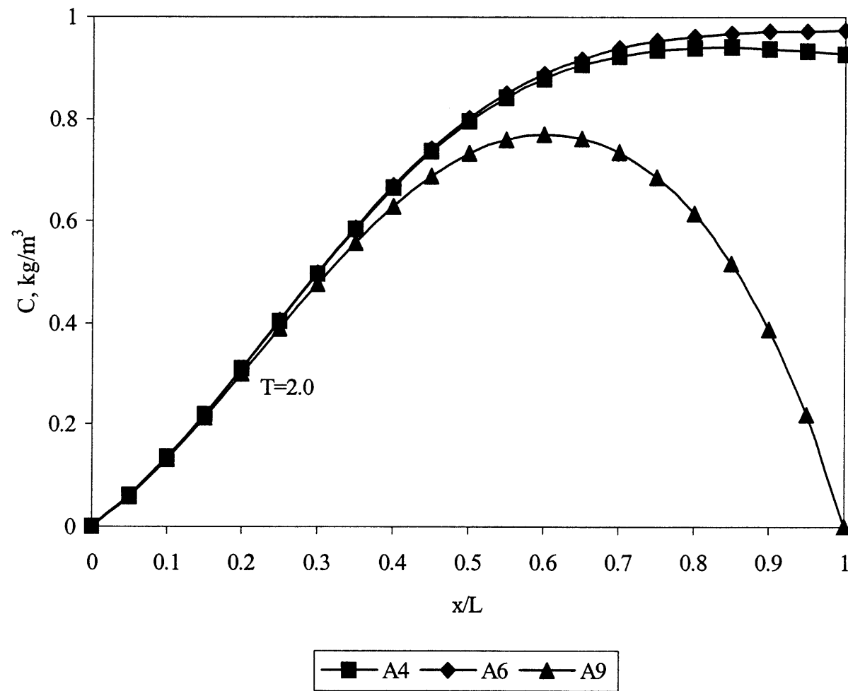
Figure 3.5 Concentration Profile Comparison for Peclet Number P=5 (Continued).
