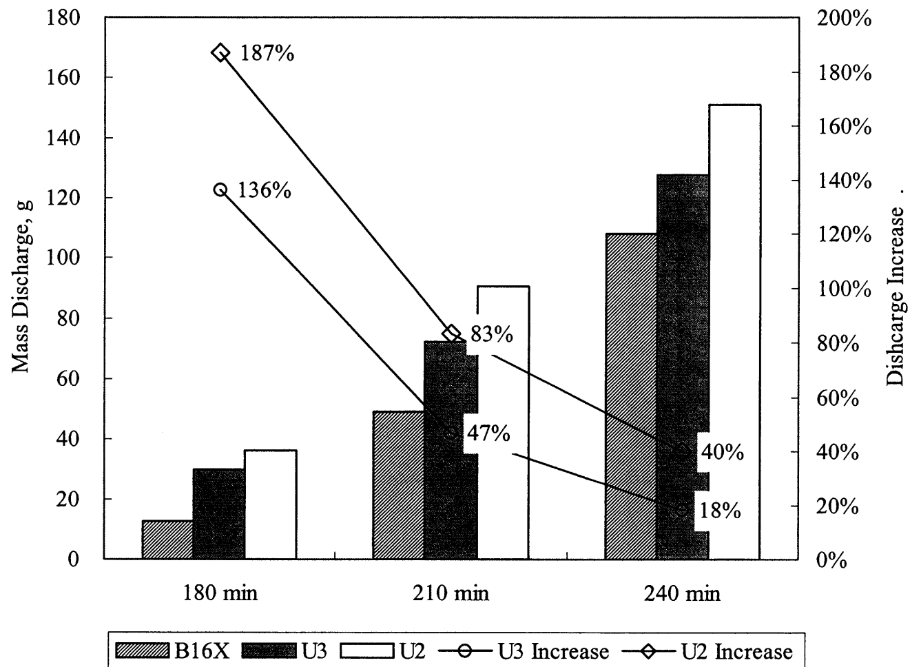
Figure 4.28 Contaminant Discharge Comparison.
