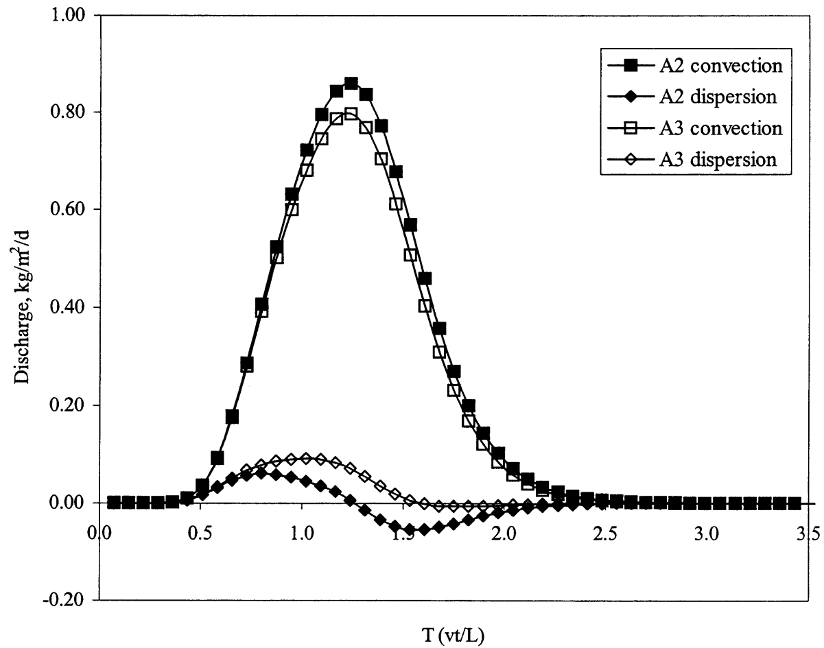
Figure 3.8 Convection vs. Dispersion: 0.1L away from the Boundary (Continued).
