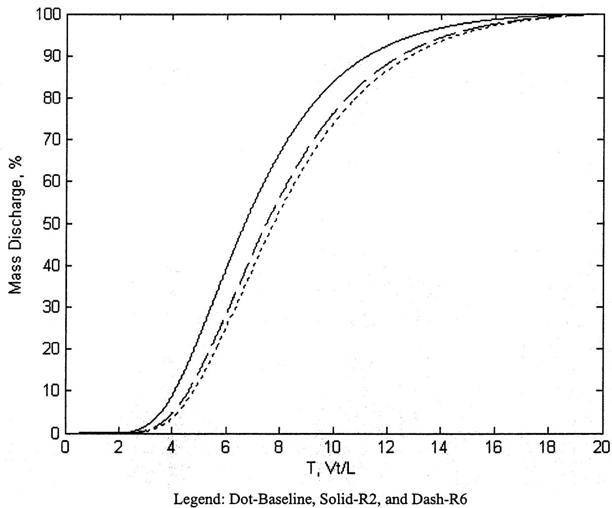
Figure 5.32 Tidal Effect on Contaminant Discharge subject to Different Confining Status.
