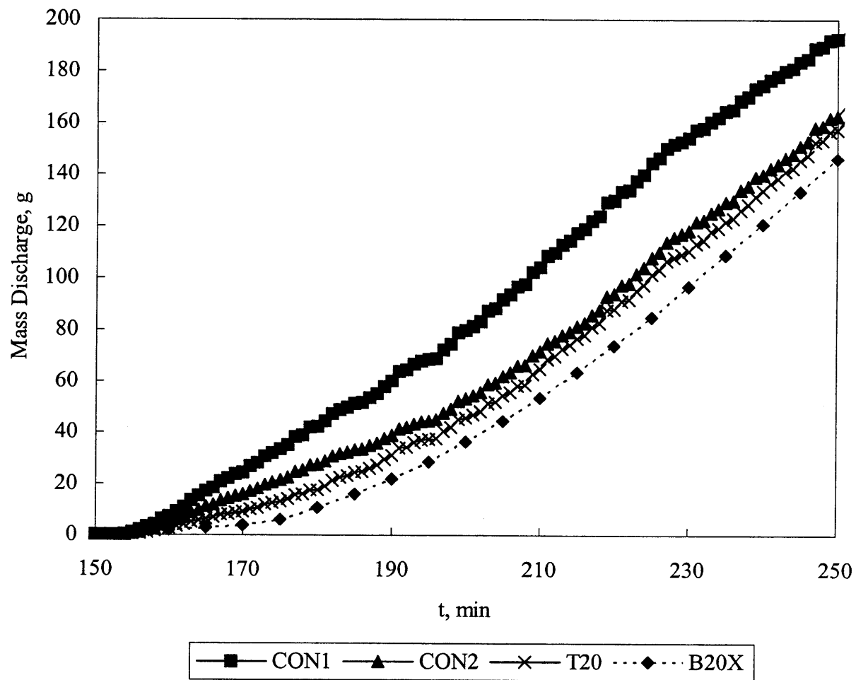
Figure 4.46 Contaminant Discharge Comparison.
