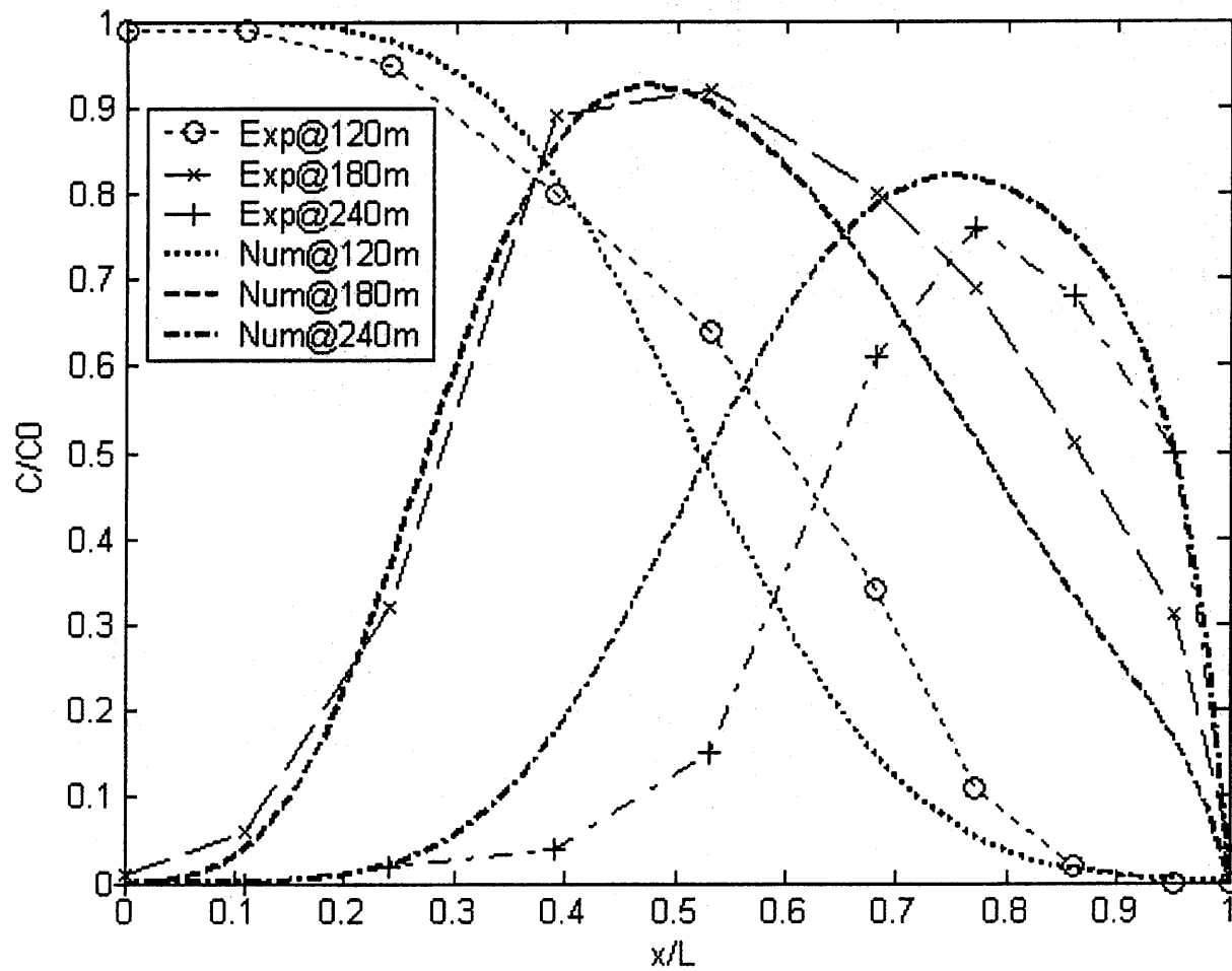
Figure 4.13 Comparison of Experimental and Numerical Results for Case CON1.
