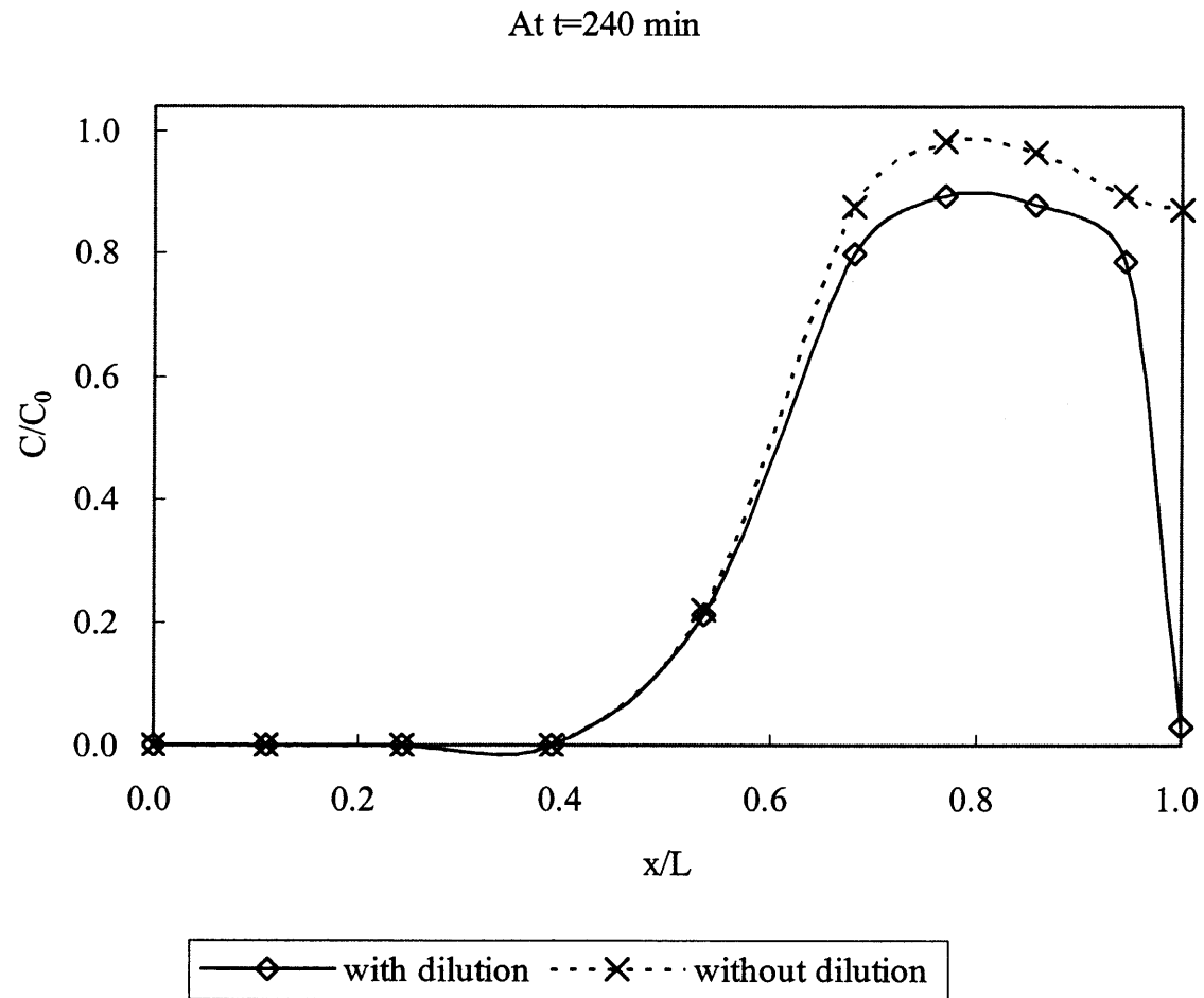
Figure 4.19 Contaminant Distribution subject to Dilution and Mixing (DF=29.39) (Continued).
