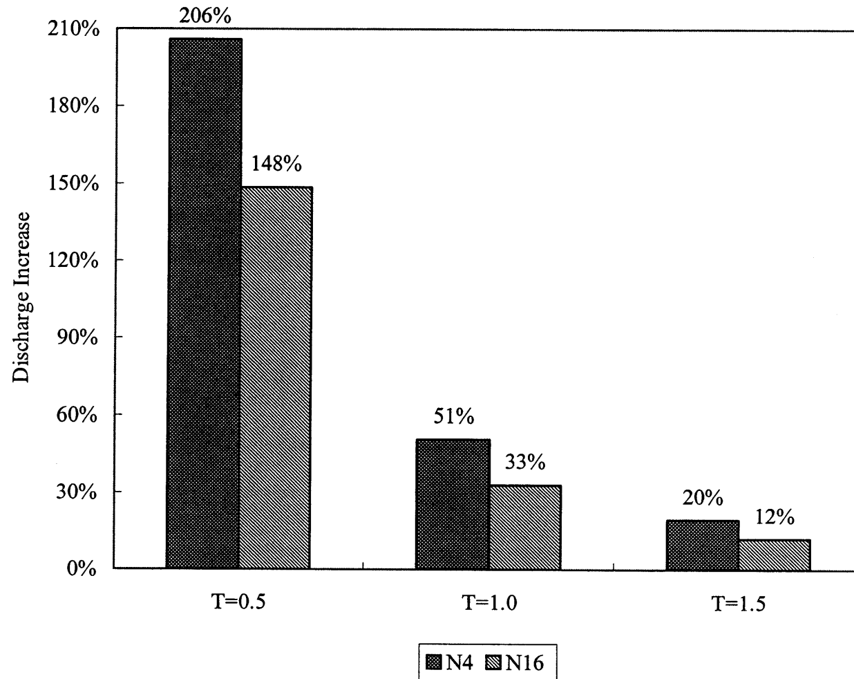
Figure 5.27 Tidal Effect on Contaminant Discharge subject to Different Confining Status.
