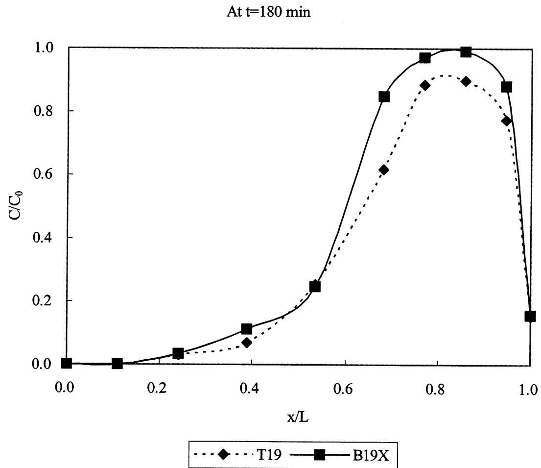
Figure 4.32 Contaminant Distribution for Case T19 (Continued).
