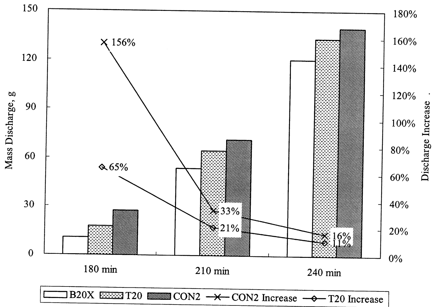
Figure 4.44 Contaminant Discharge Comparison.
