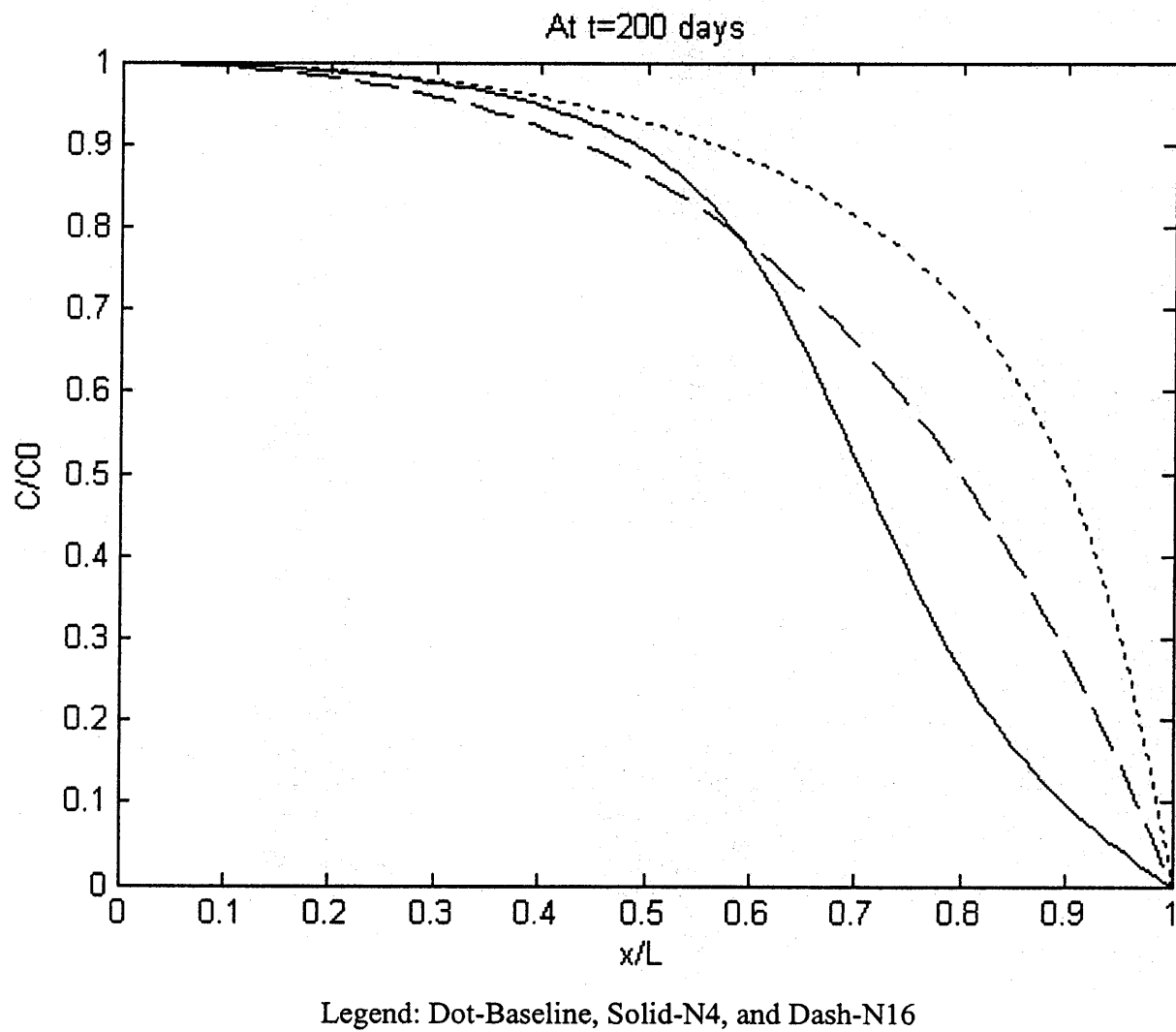
Figure 5.25 Tidal Effect on Contaminant Distribution.
