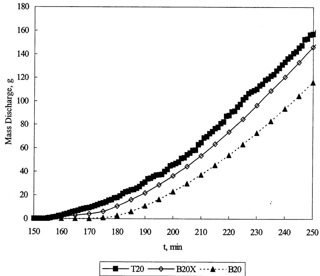
Figure 4.41 Contaminant Discharge Comparison.
