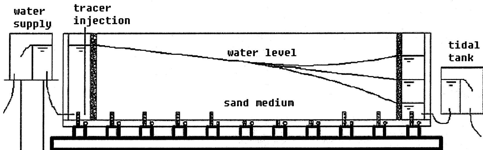
Figure 4.21 Unconfined-Condition Experiments.
