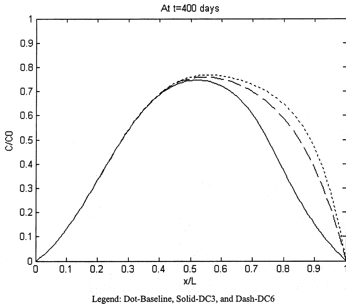
Figure 5.34 Tidal Effect on Contaminant Distribution (Continued).
