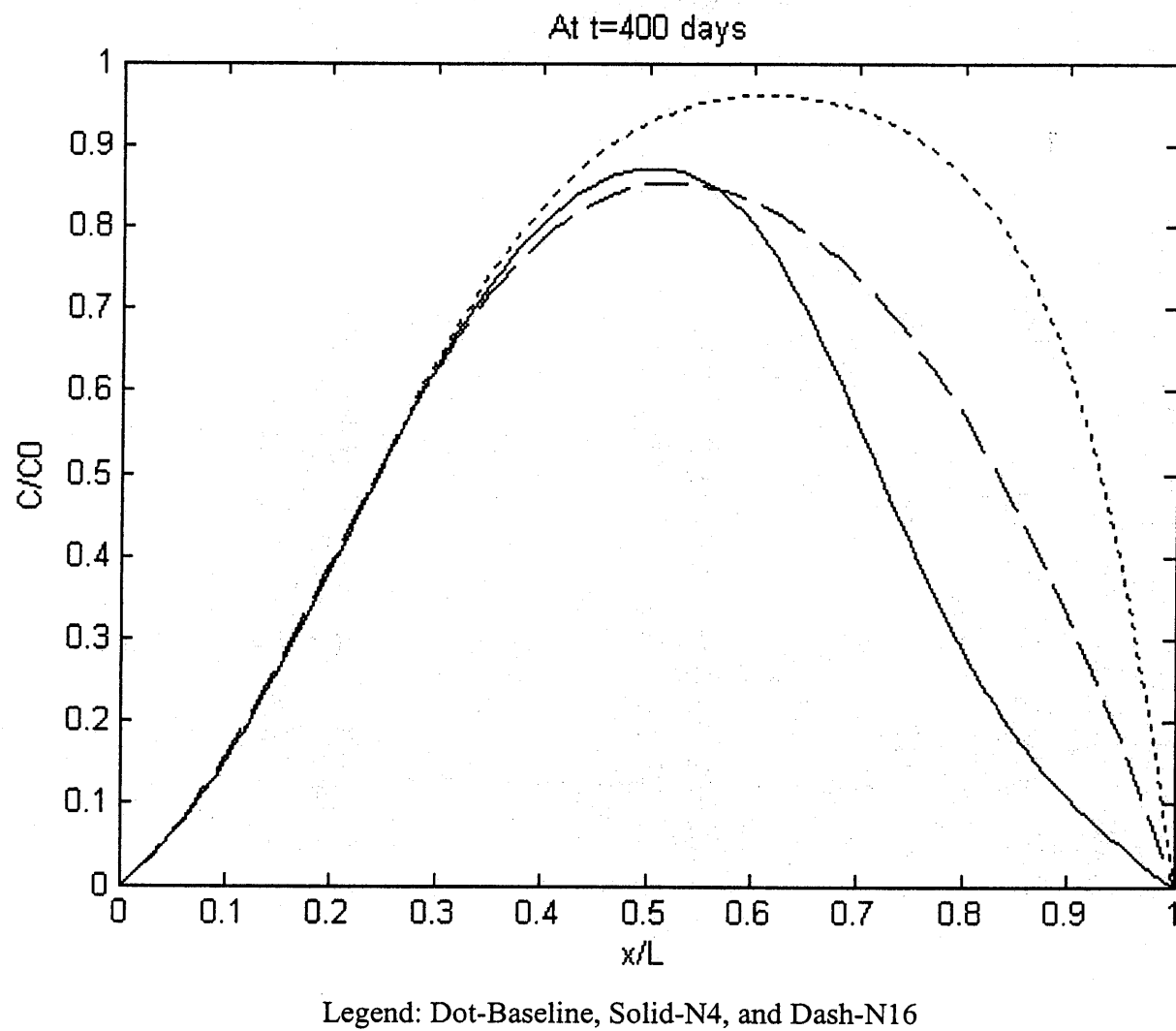
Figure 5.25 Tidal Effect on Contaminant Distribution (Continued).
