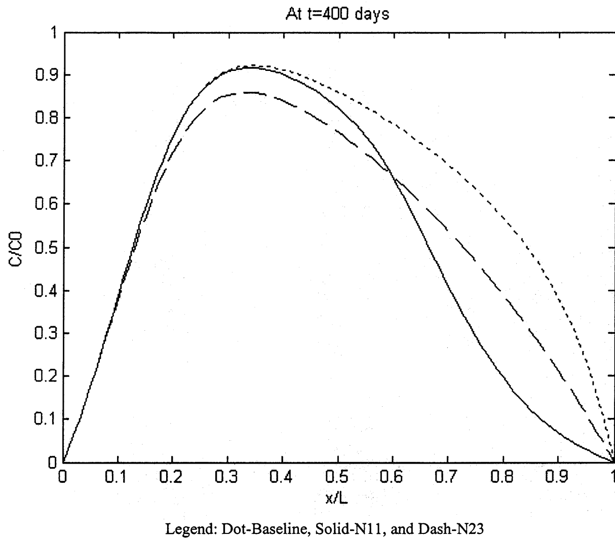
Figure 5.28 Tidal Effect on Contaminant Distribution.
