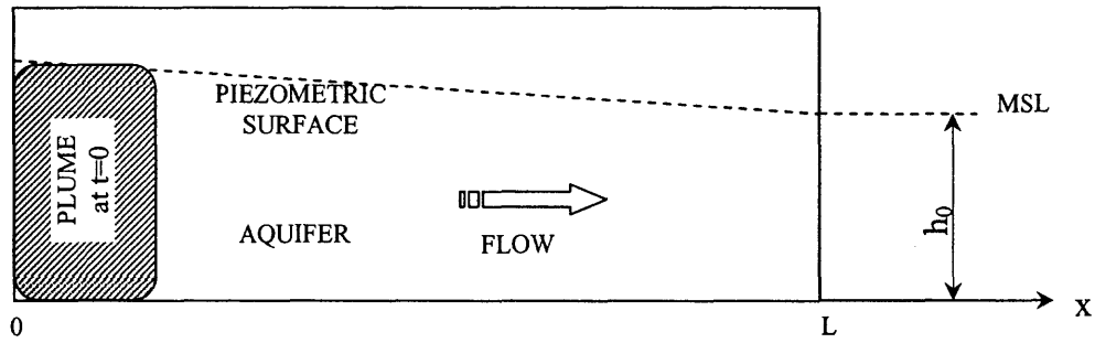
Figure 3.3 Illustration of the Baseline Problem without Tides.
