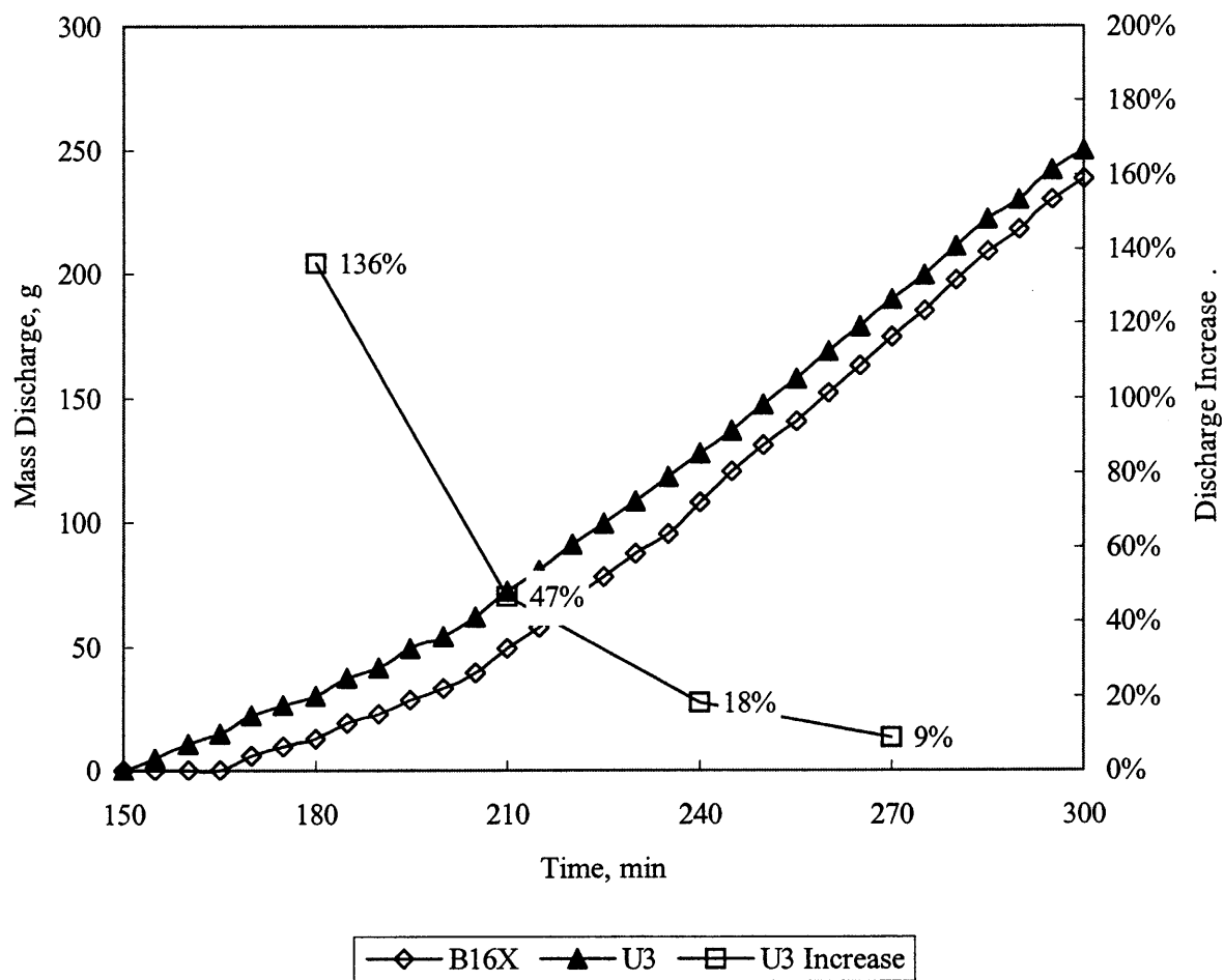
Figure 4.30 Contaminant Discharge Comparison.
