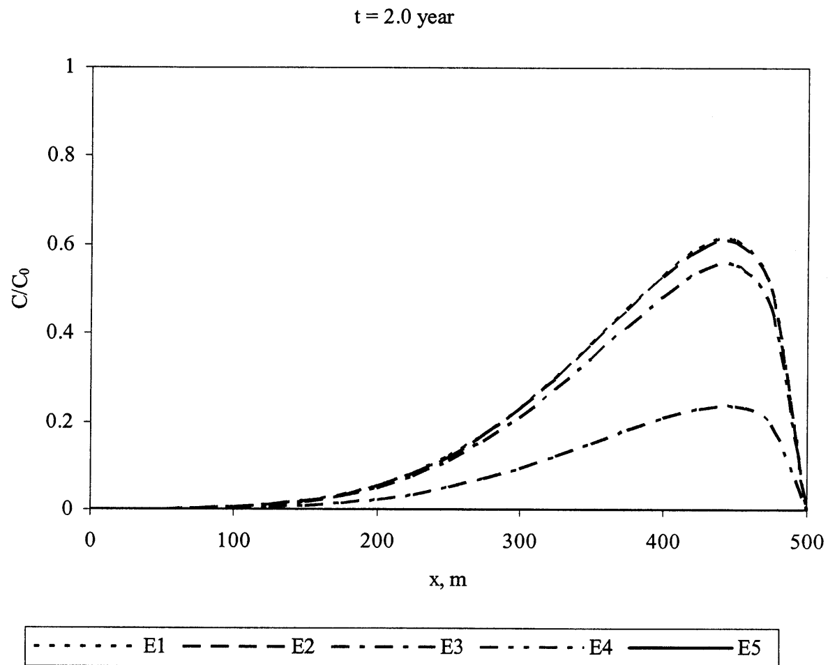
Figure 5.16 Evaluation of Decay-Concentration Distribution Relation (Continued).
