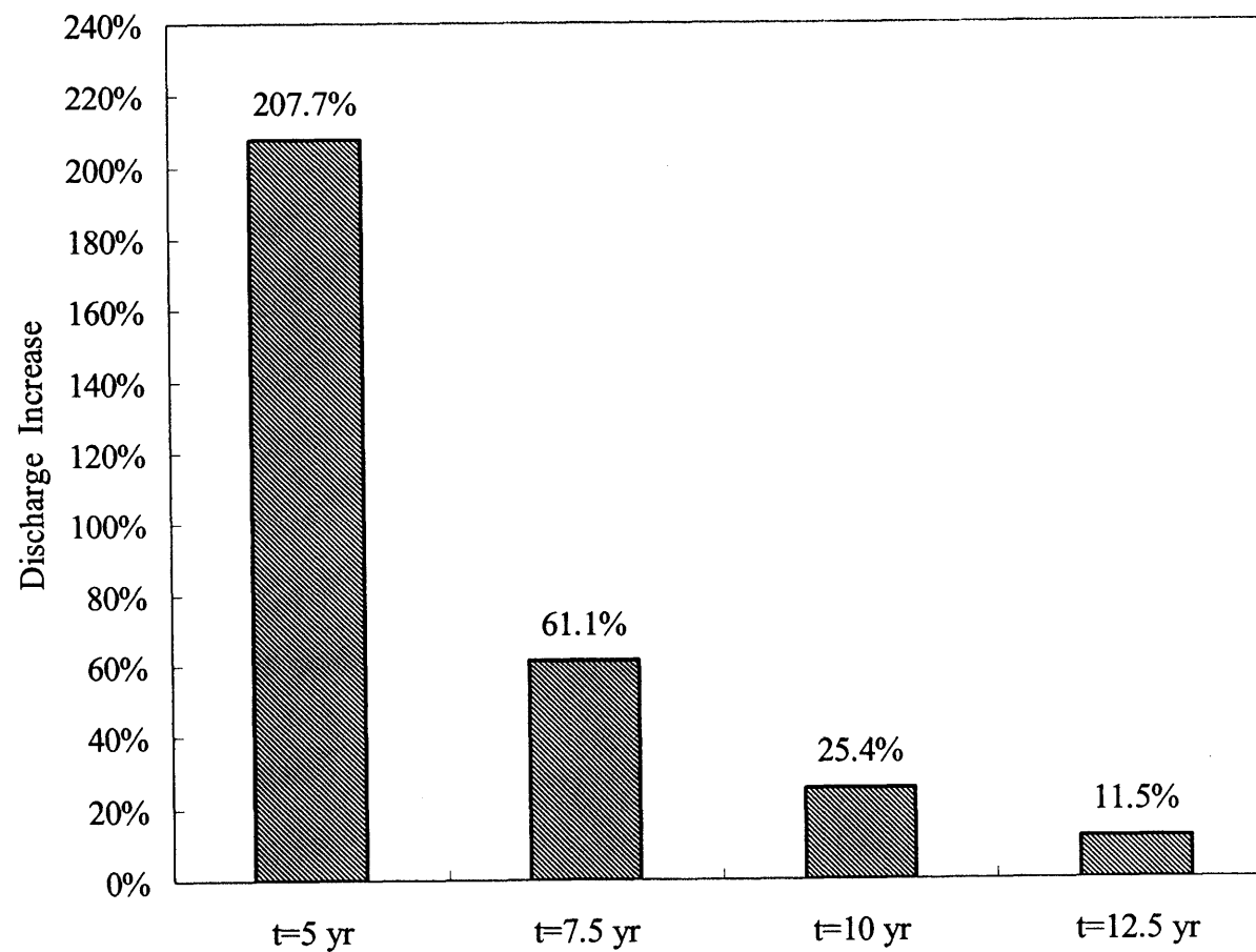
Figure B.3 Contaminant Discharge Increase in the Field Application Study.
