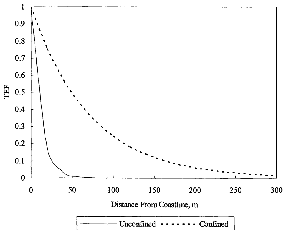
Figure 5.1 Tidal Efficiency Factor under Confined and Unconfined Conditions.
