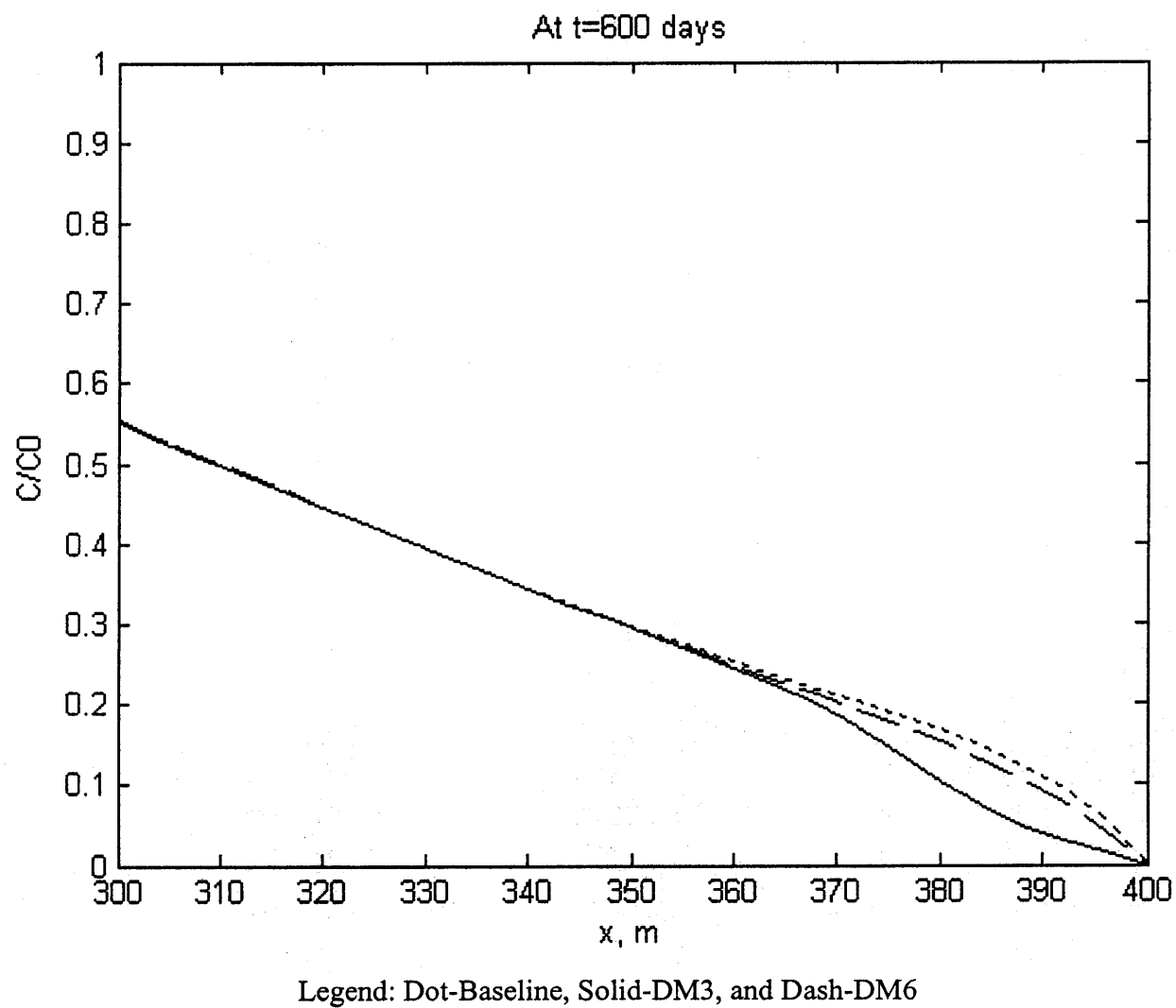
Figure 5.37 Tidal Effect on Contaminant Distribution.
