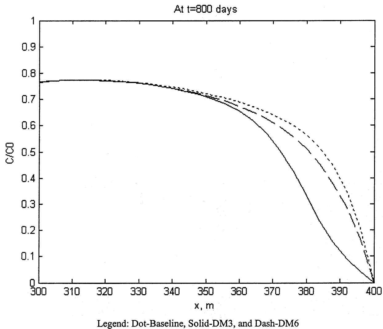
Figure 5.37 Tidal Effect on Contaminant Distribution (Continued).
