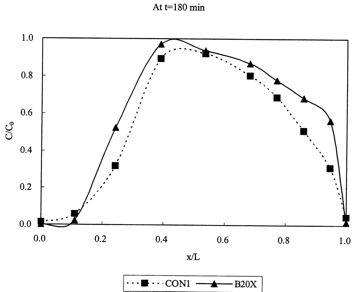
Figure 4.45 Contaminant Distribution for Case CON1.
