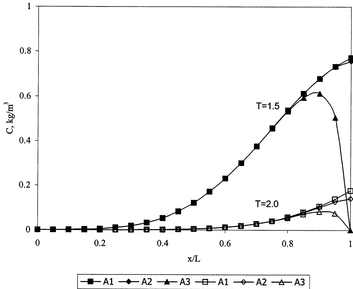
Figure 3.4 Concentration Profile Comparison for Peclet Number P=25 (Continued).
