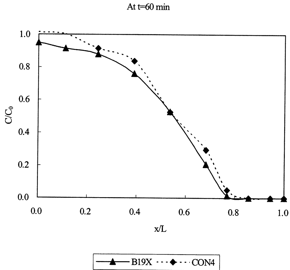
Figure 4.34 Contaminant Distribution for Case CON4.
