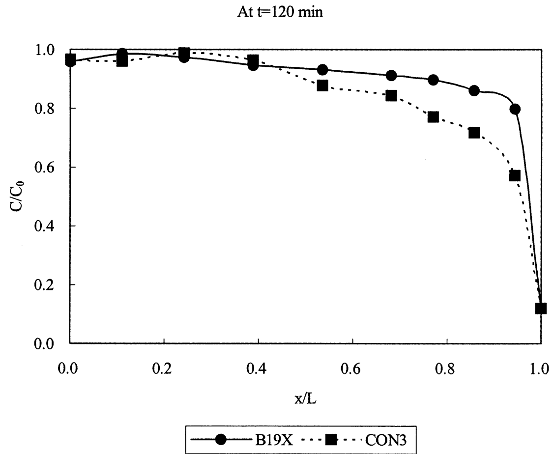
Figure 4.37 Contaminant Distribution for Case CON3.
