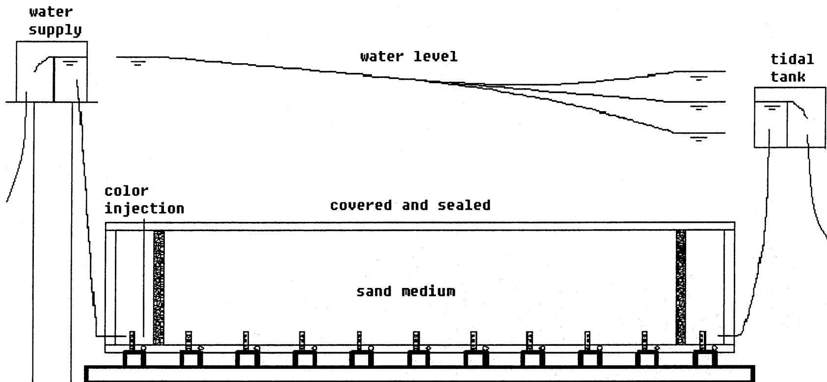
Figure 4.31 Confined-Condition Experiments.
