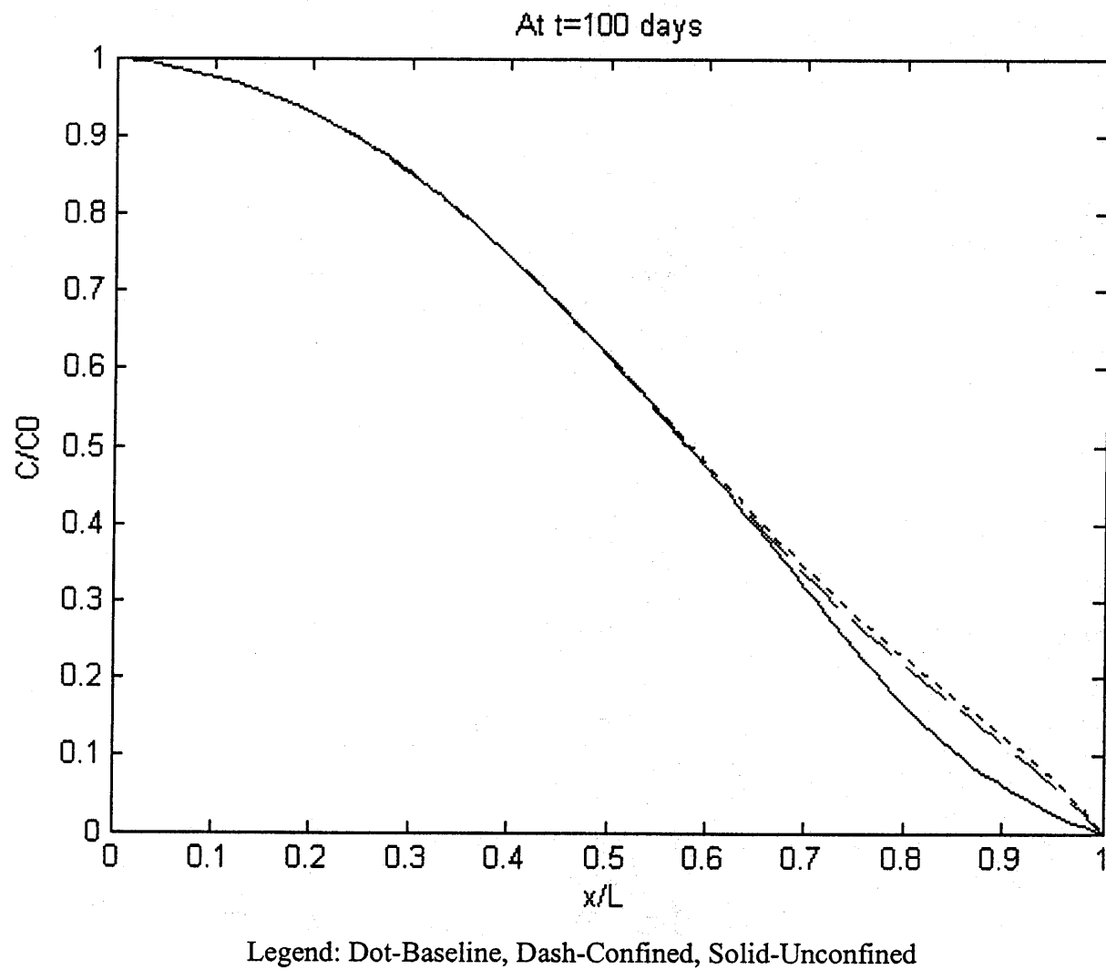
Figure 5.2 Tidal Effect on Contaminant Distribution in Confined versus Unconfined Aquifers.
