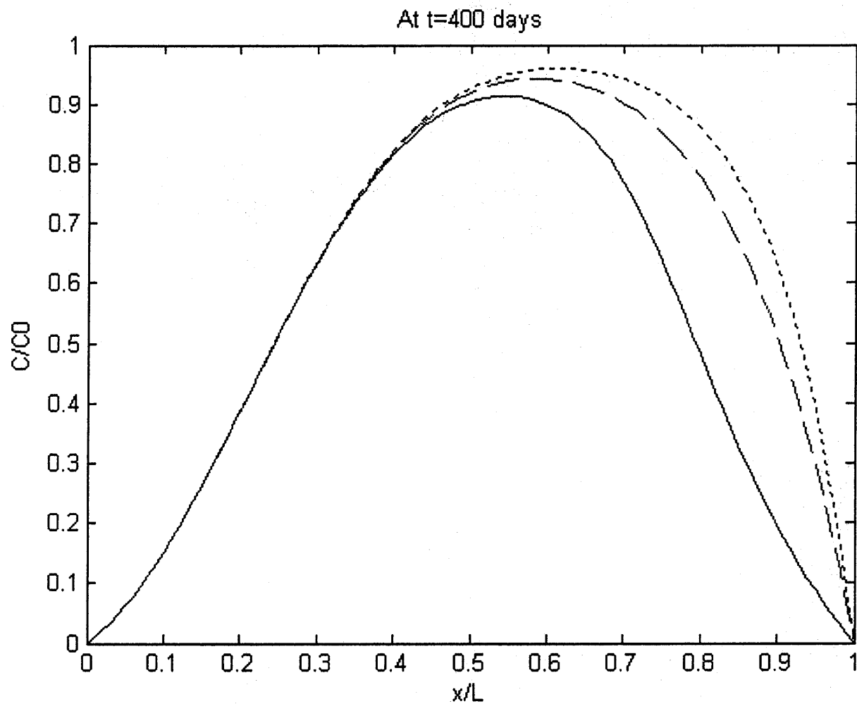
Figure 5.2 Tidal Effect on Contaminant Distribution in Confined versus Unconfined Aquifers (Continued).
