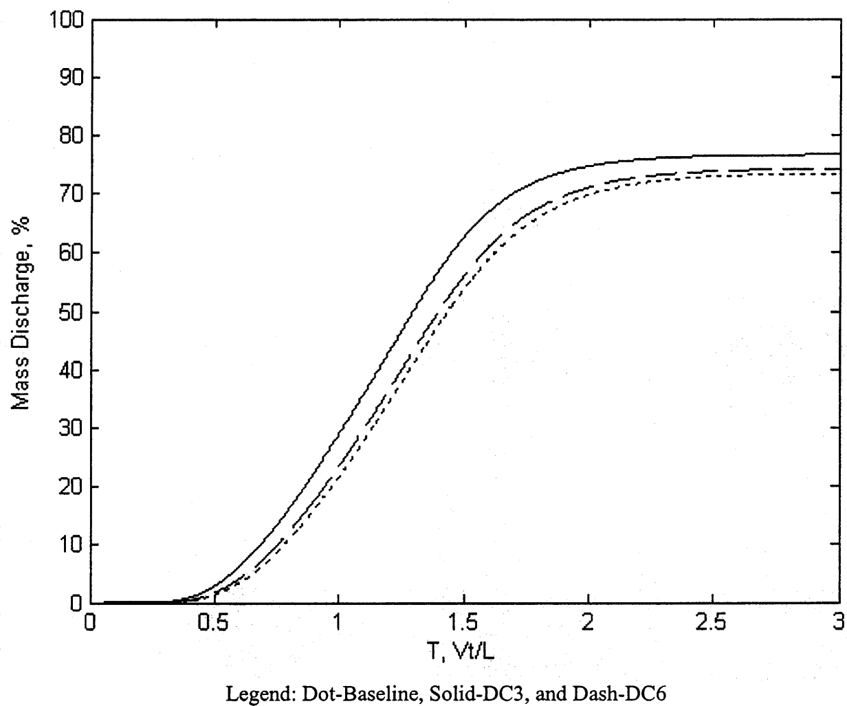
Figure 5.35 Tidal Effect on Contaminant Discharge subject to Different Confining Status.
