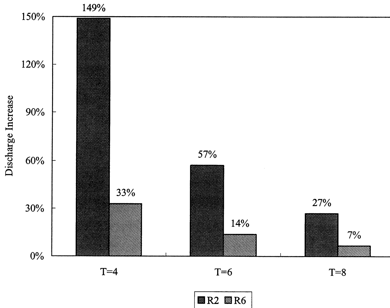
Figure 5.33 Tidal Effect on Contaminant Discharge subject to Different Confining Status.
