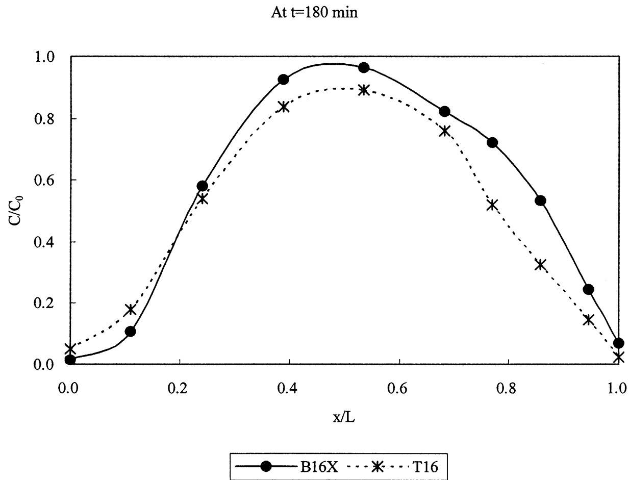
Figure 4.22 Contaminant Distribution for Case T16.
