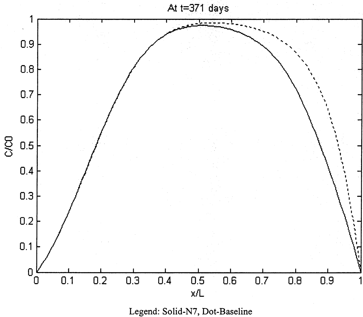
Figure 5.8 Comparison of Tidal Effect on Contaminant Distribution at Stage I.
