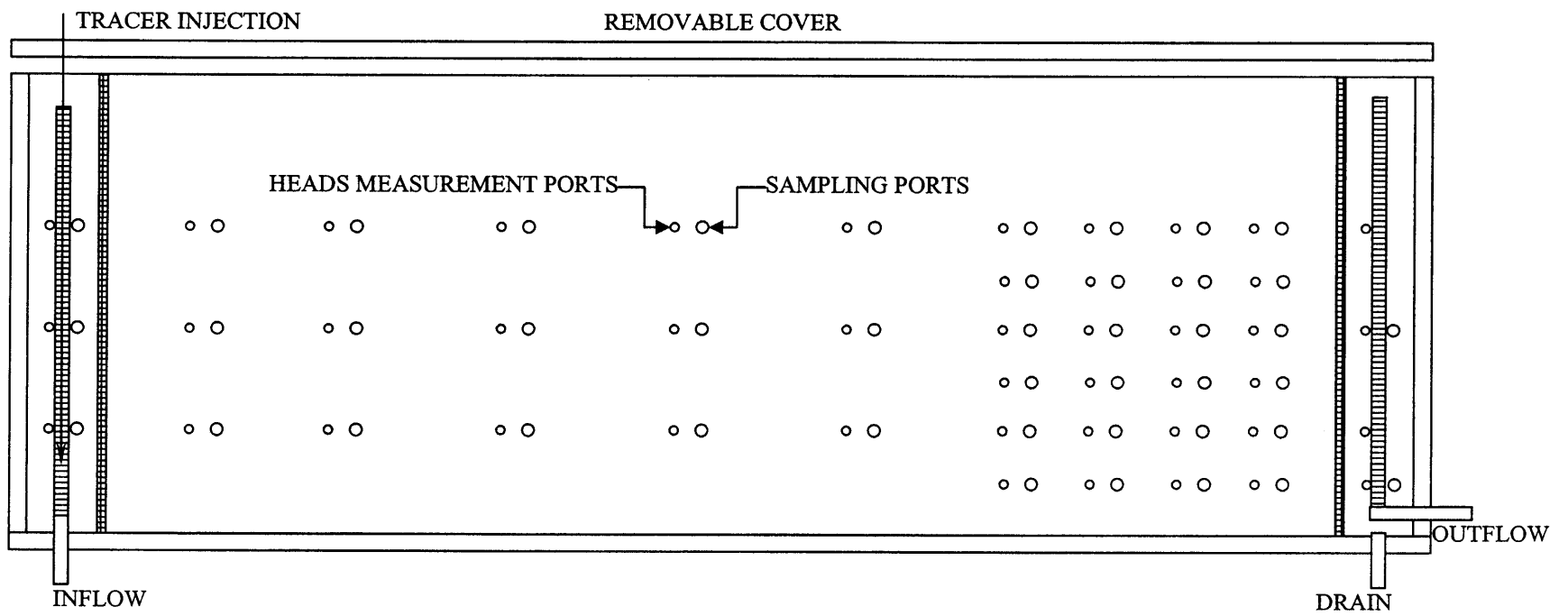
Figure 4.2 Positions of Tracer Sampling and Heads Measurement Ports.
