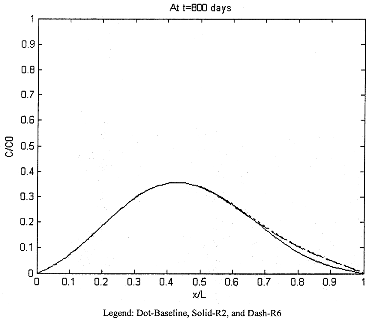
Figure 5.31 Tidal Effect on Contaminant Distribution.
