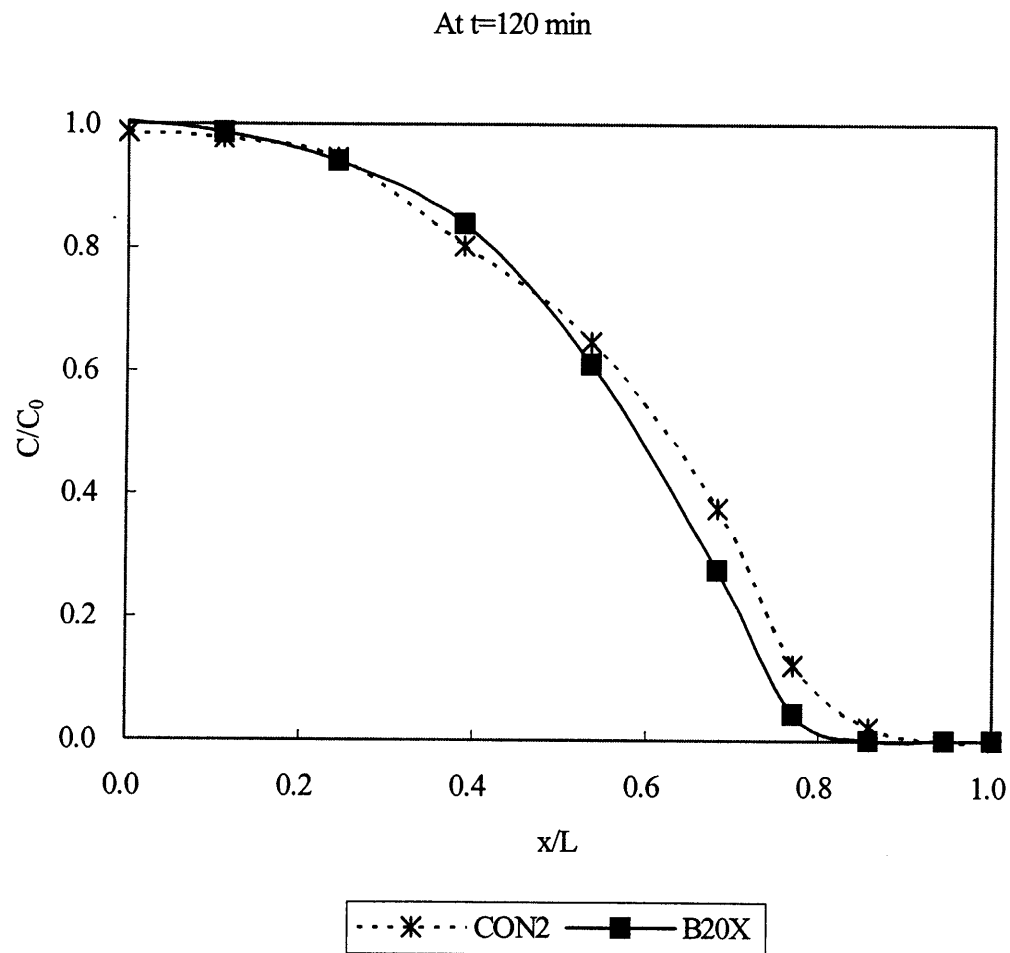
Figure 4.42 Contaminant Distribution for Case CON2.
