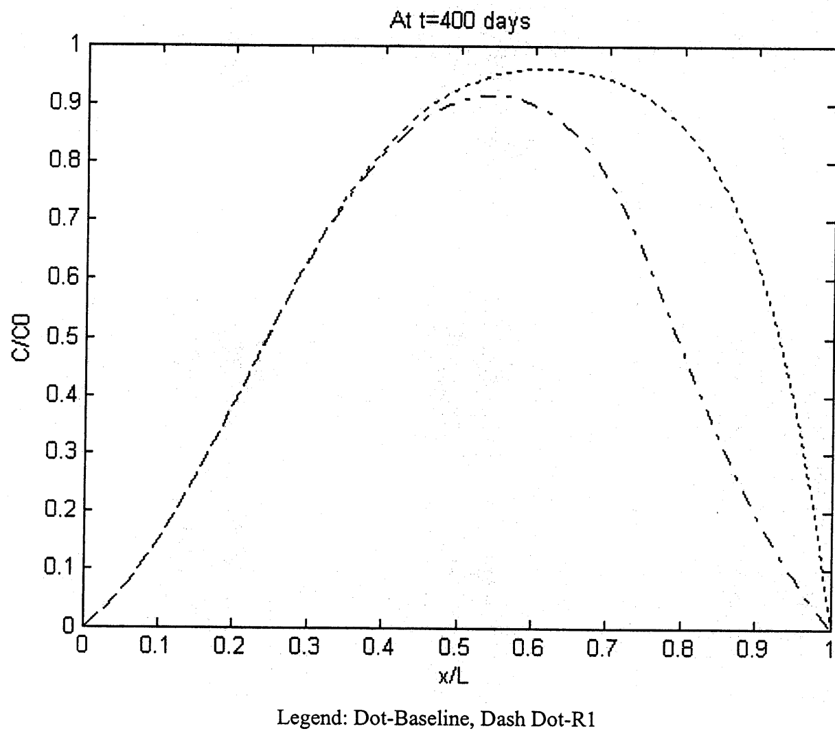
Figure 5.13 Tidal Effect on Contaminant Distribution at Stage I.
