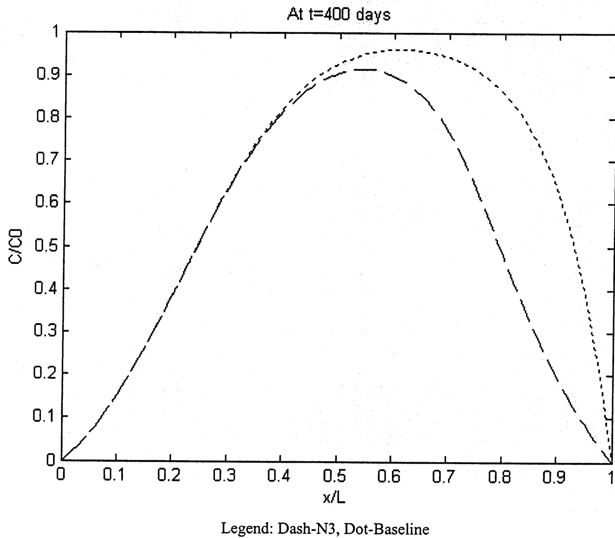
Figure 5.8 Comparison of Tidal Effect on Contaminant Distribution at Stage I (Continued).
