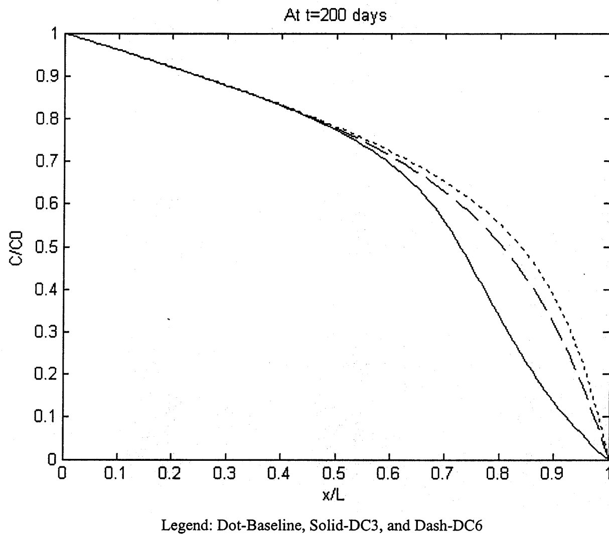
Figure 5.34 Tidal Effect on Contaminant Distribution.
