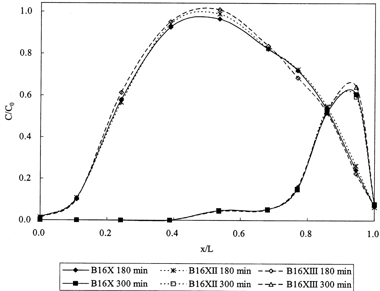
Figure 4.5 Experimental Repeating Tests for Case B16X.
