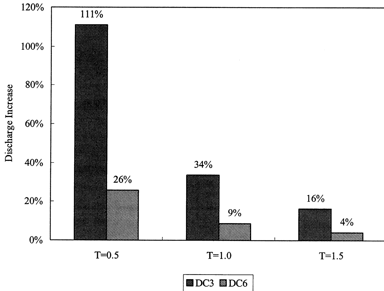
Figure 5.36 Tidal Effect on Contaminant Discharge subject to Different Confining Status.
