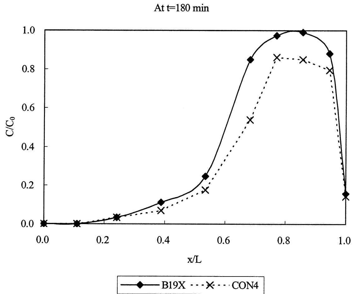
Figure 4.34 Contaminant Distribution for Case CON4 (Continued).
