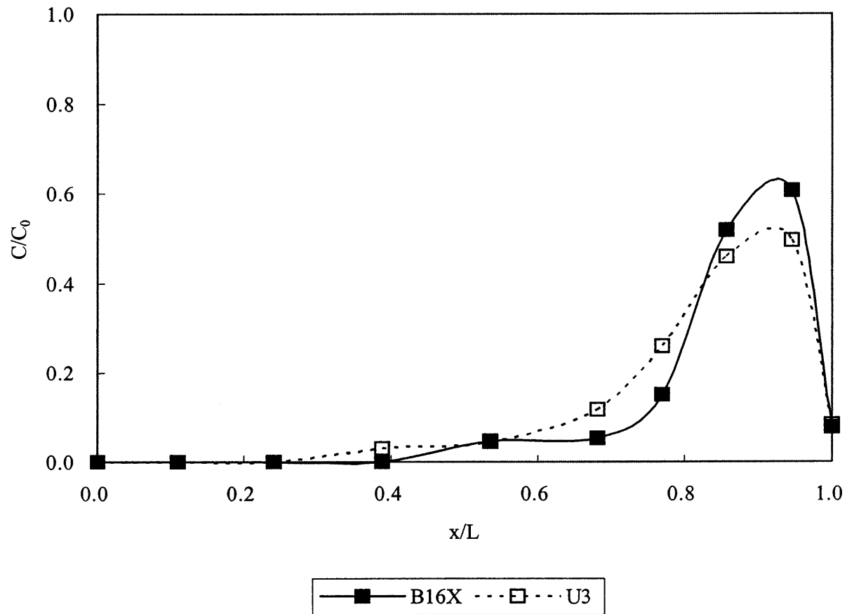
Figure 4.29 Contaminant Distribution for Case U3 (Continued).
