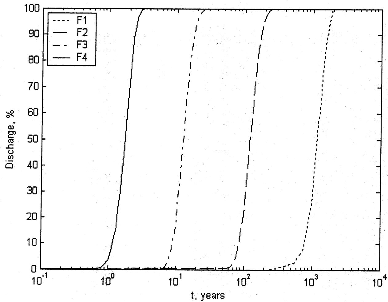
Figure 5.12 Retardation-Discharge Relation.
