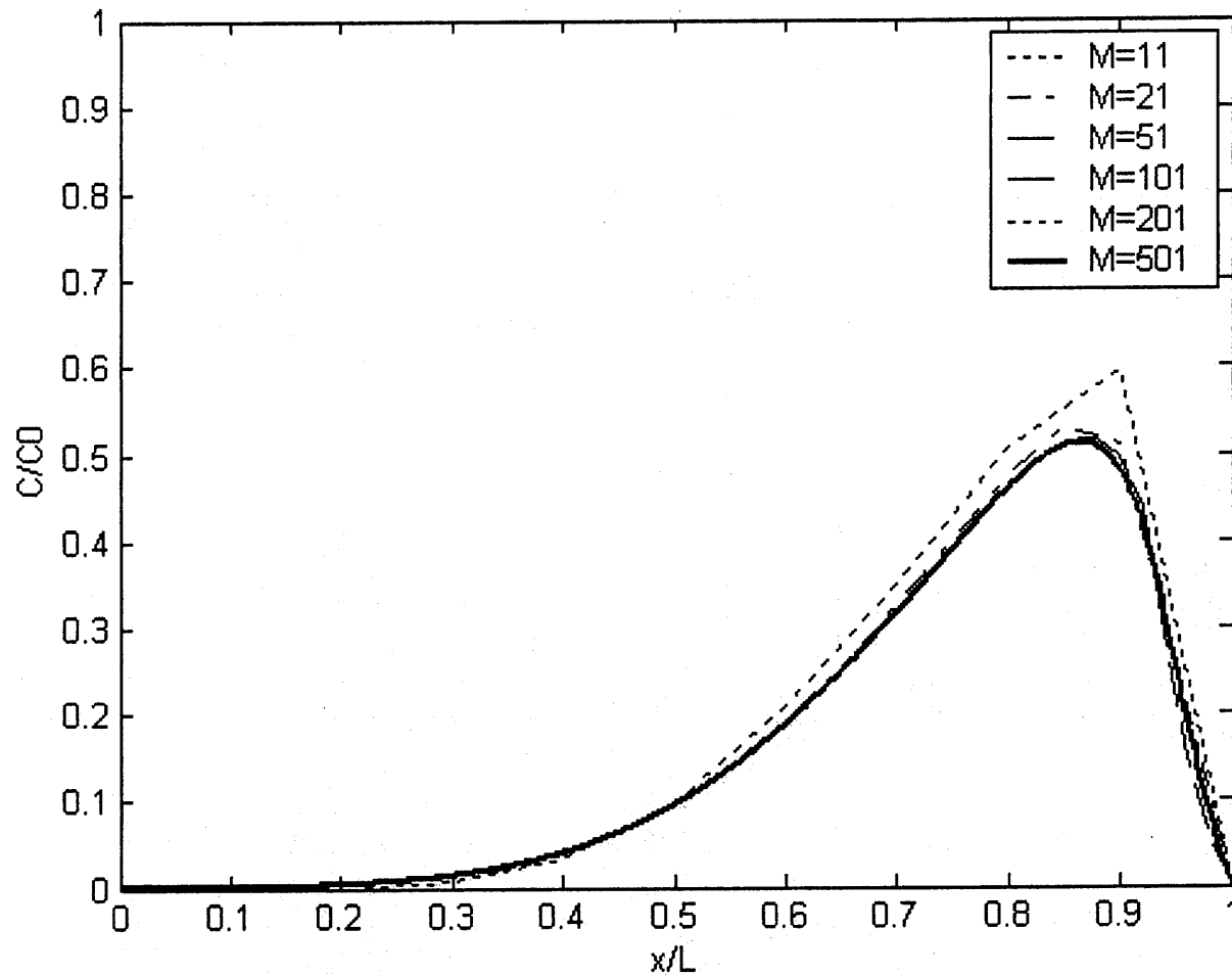
Figure 3.10 Numerical Solution Convergence Test with \Delta t = 0.2v_{\max}\Delta x .
