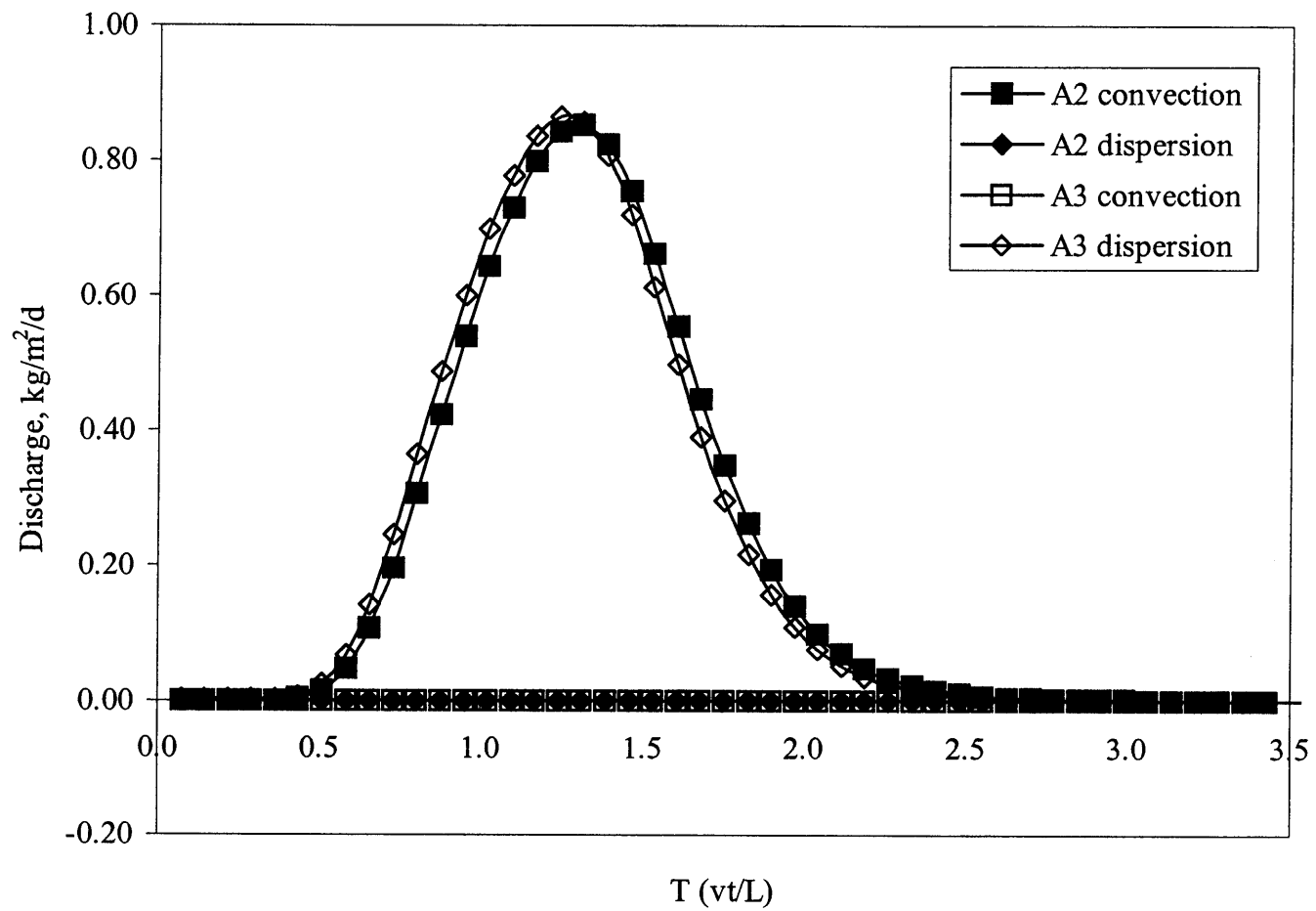
Figure 3.8 Convection vs. Dispersion: At the Coastal Boundary.
