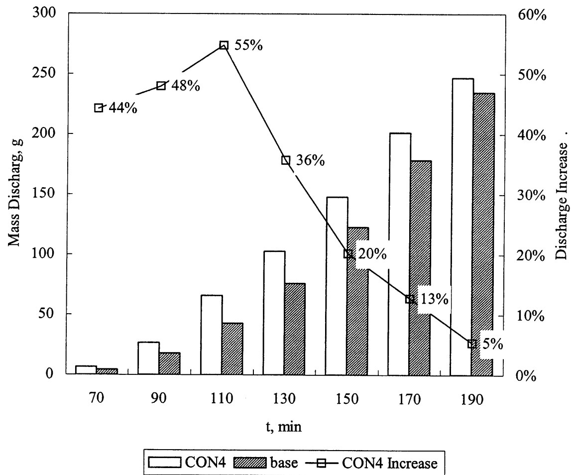
Figure 4.36 Contaminant Discharge Comparison.
