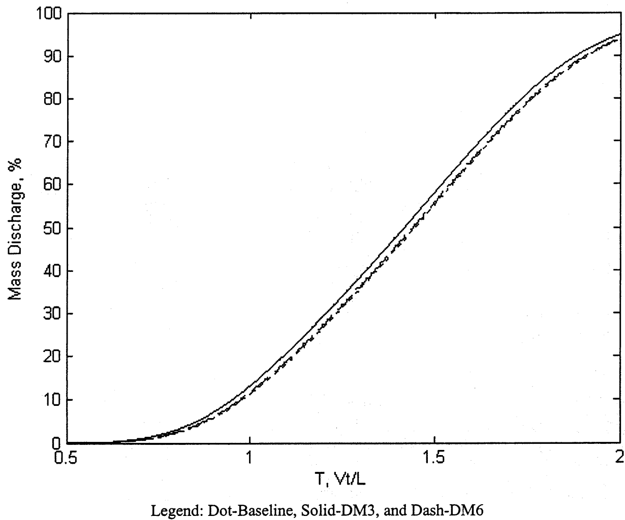
Figure 5.38 Tidal Effect on Contaminant Discharge subject to Different Confining Status.
