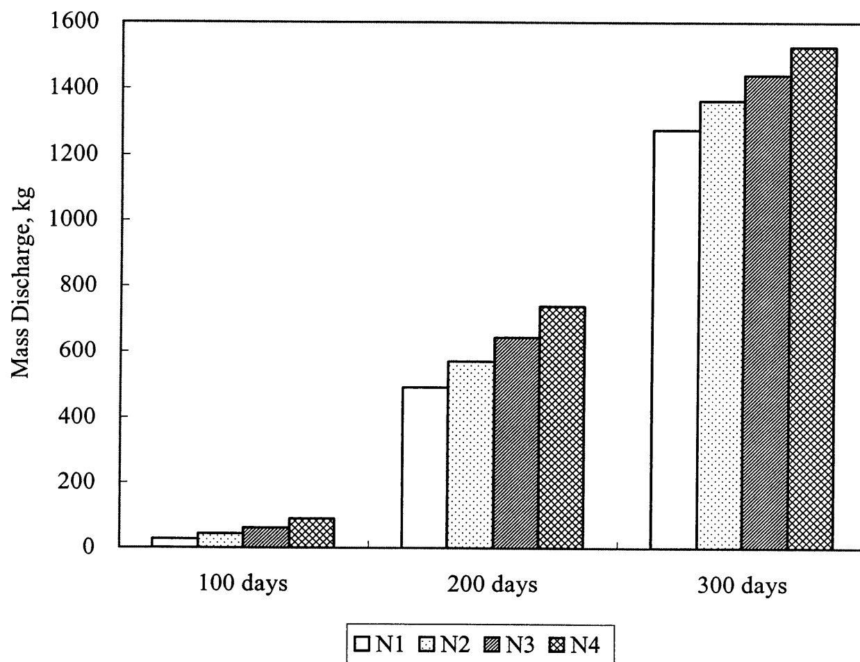
Figure 5.5 Contaminant Discharge subject to Different Tidal Amplitudes.
