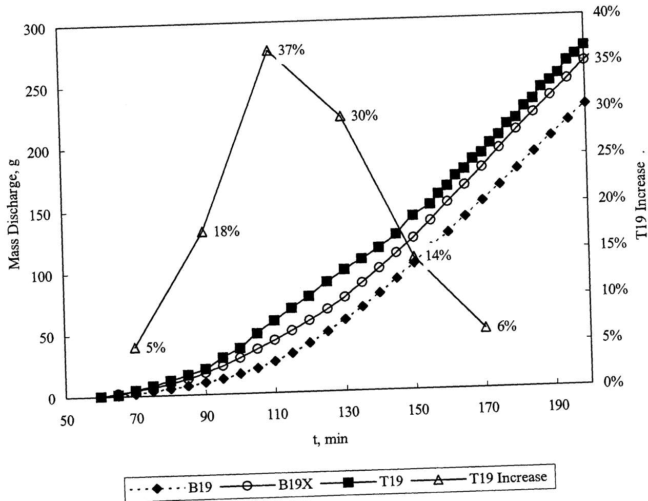
Figure 4.33 Contaminant Discharge Comparison.
