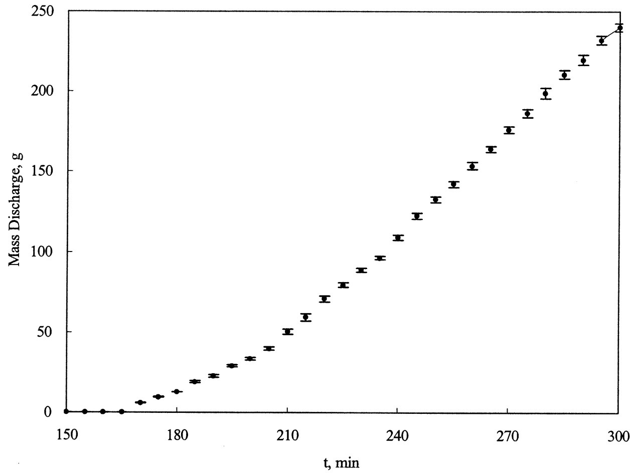
Figure 4.6 Experimental Repeating Tests for Case B16X.
