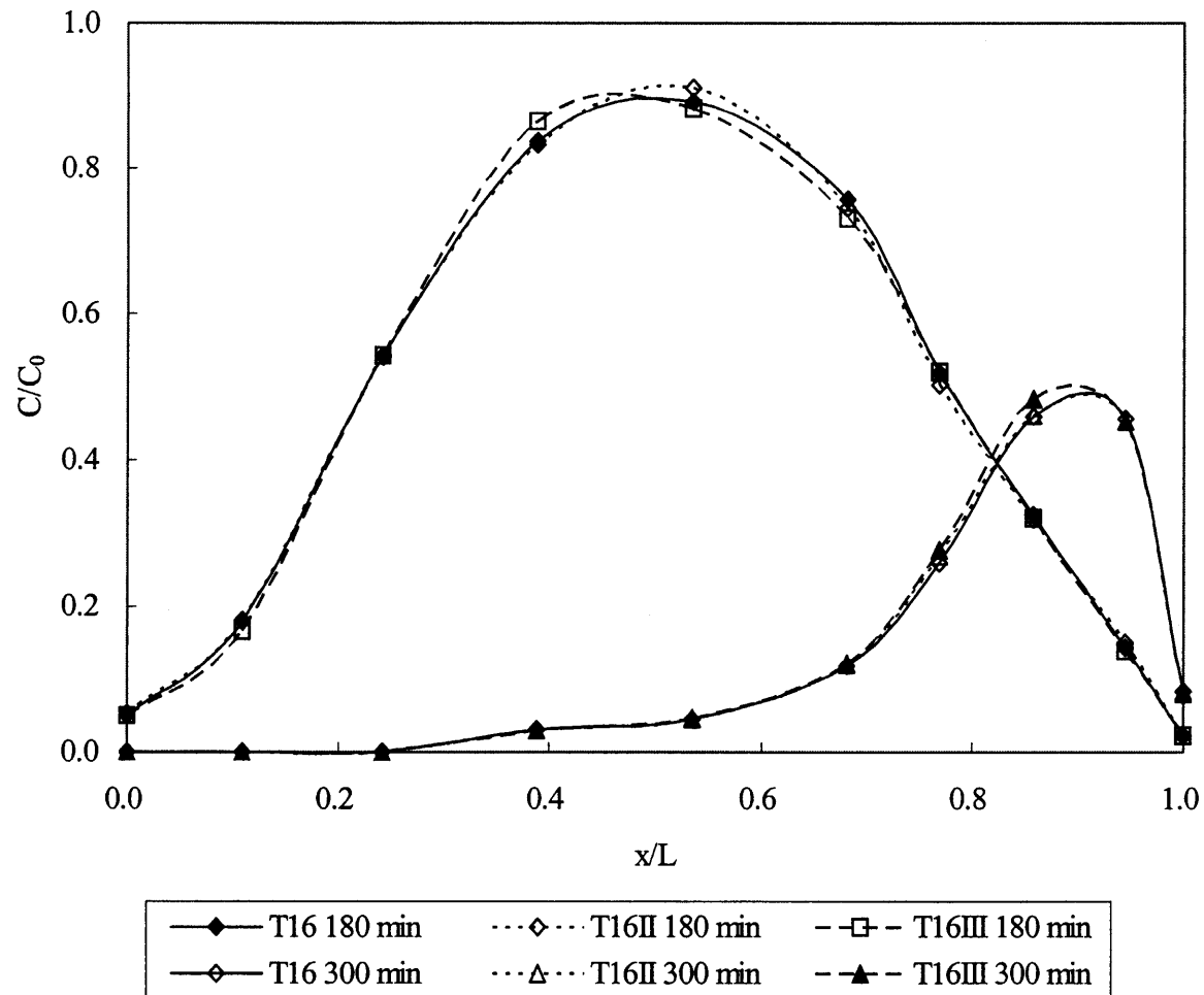
Figure 4.7 Experimental Repeating Tests for Case T16.
