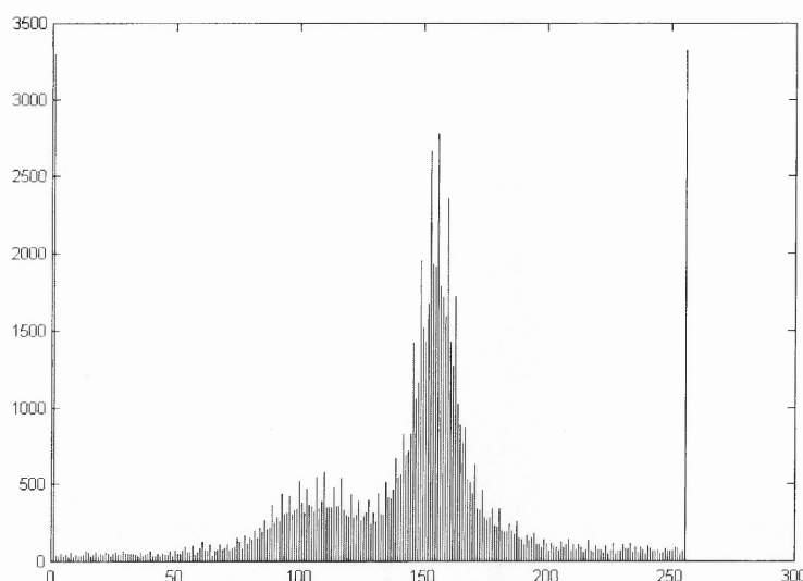
Figure 4.4 Histogram of one medical image. (Note that there are two huge peaks, 164,683 and 20,739, in the histogram, located at gray levels 0 and 255, respectively. They have been scaled down on purpose in order to show more details for the vast majority of other gray levels.)
