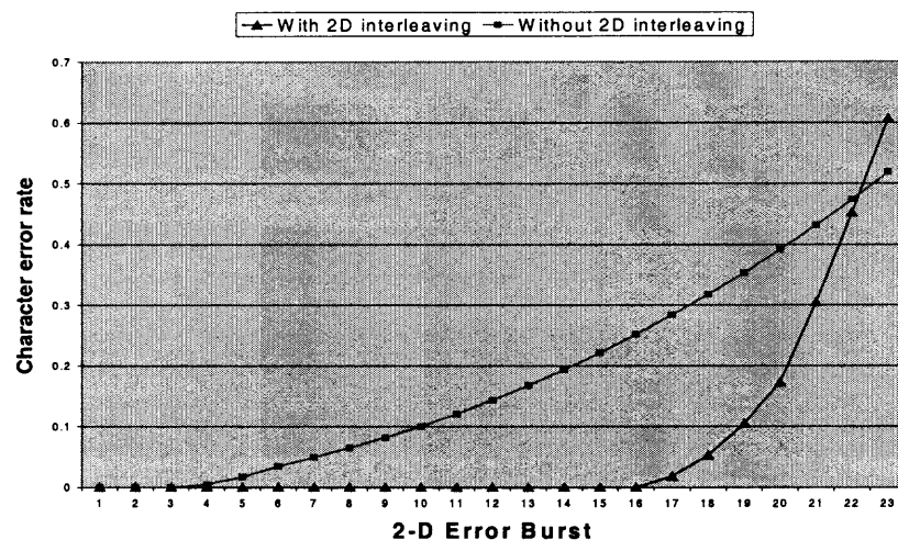
Figure 3.1 Results for block burst error attack.
