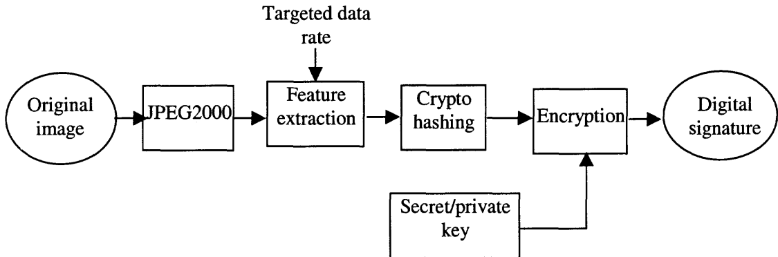
Figure 5.25 Block diagram of content signing.
