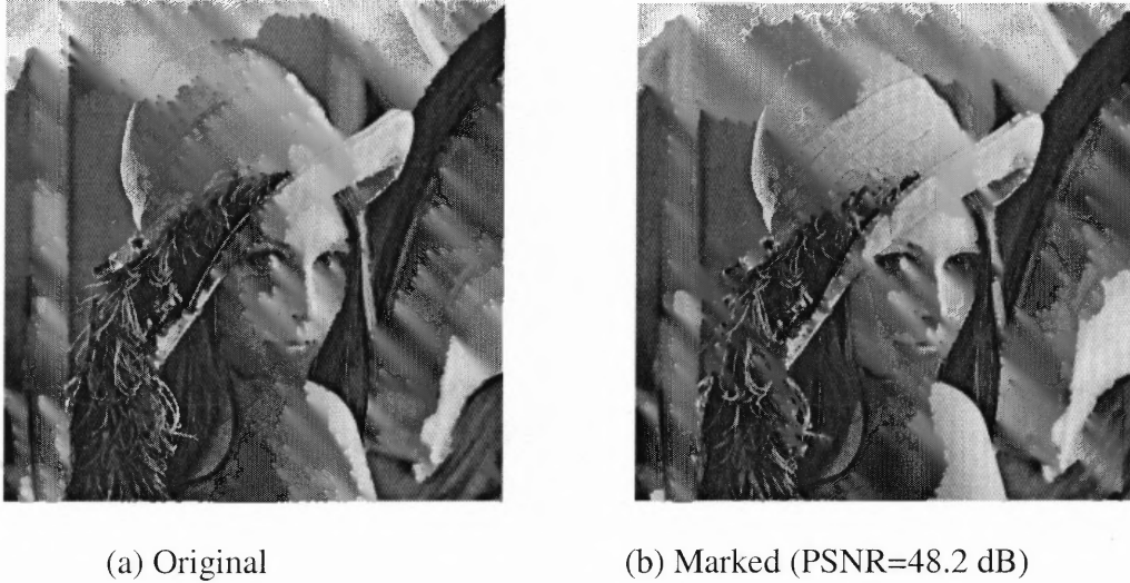
Figure 4.2 Lena image.
