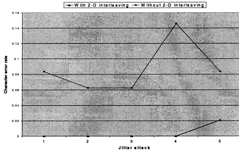
Figure 3.3 Results for “StirMark” jitter attack.
