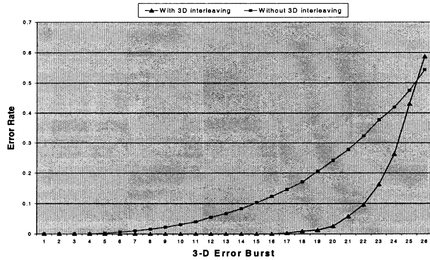
Figure 3.5 Results for 3-D error burst attack.
