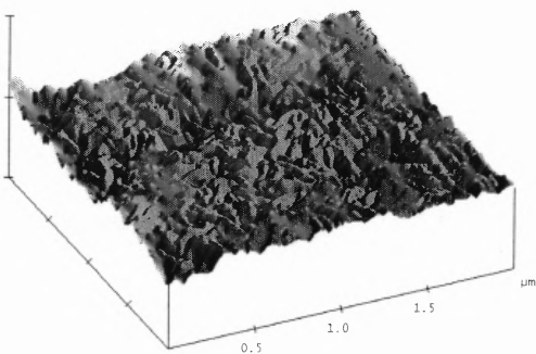
(e) \beta -Ta 5 \mu\text{m} , R_{\text{rms}} = 7.2 nm
