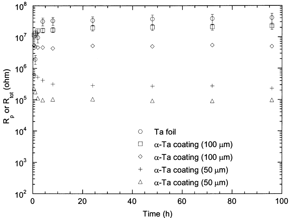
Figure 6.12 R_p of Ta foil and R_{tot} of the 50 and 100 \mu m \alpha -Ta coatings as a function of time. Error bars not visible are present within symbol.
