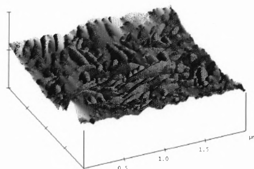
(b) \alpha -Ta 10 \mu\text{m} , R_{\text{rms}} = 9.8 nm
