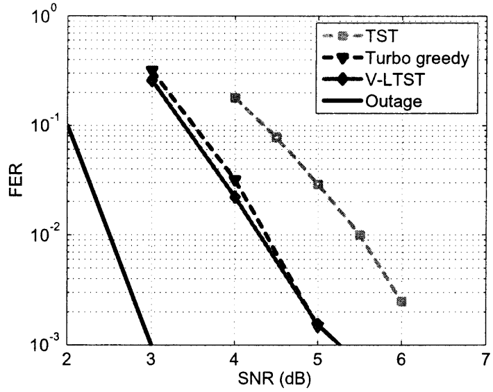
Figure 5.4 FER comparison of V-LTST and other schemes, 8 \times 8 , 8b/s/Hz.
