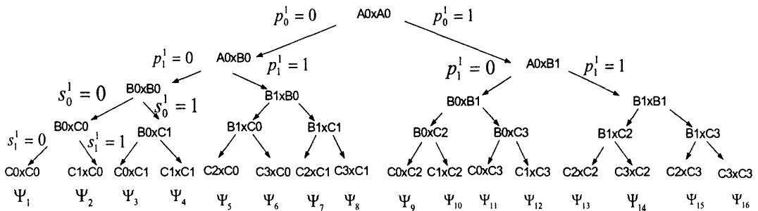
Figure 4.3 Partition of a 2 \times 16 QAM constellation based on the 16 QAM set partition.
