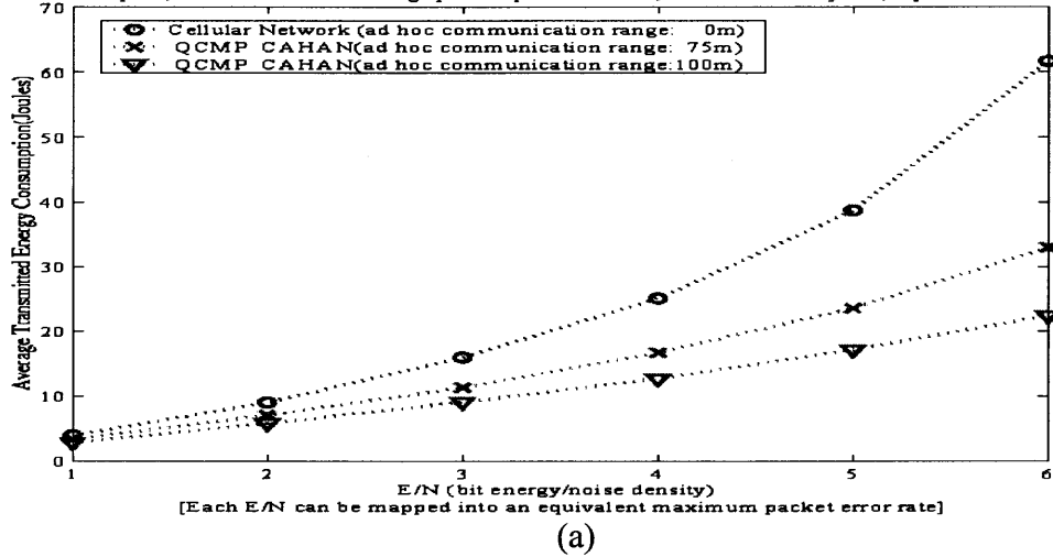
Total Data Packet & Control Packet Energy Consumption of Cellular Networks/QCMP CAHAN(Link- cost limitation downlink shortest path, Maximum MT moving speed: up to 30 m/sec, Network density: 28, Update Interval: 1 sec)
