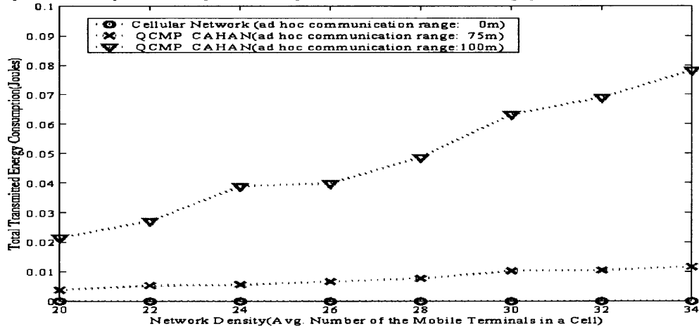
Figure 2.8 Energy consumption of RTS/CTS/ESR/ESA control packets for peer-to-peer data transmission in QCMP CAHAN: (a) uplink traffic simulation, (b) downlink traffic simulation.
