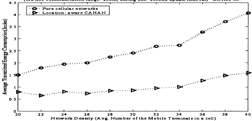
Figure 4.5 Average transmitted energy of GA CAHAN and pure cellular networks on the three different districts of service (a) Service I (the smallest target area) (b) Service II (c) Service III (the largest target area).
