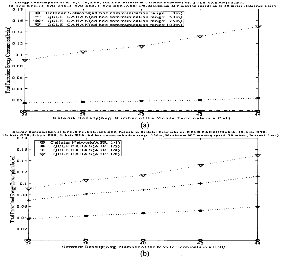
Figure 3.10 Energy consumption of RTS/CTS/ESR/ESA control packets for peer-to-peer data transmission in QCLE CAHAN: (a) Various ad hoc communication range, (b) Various ASR.
