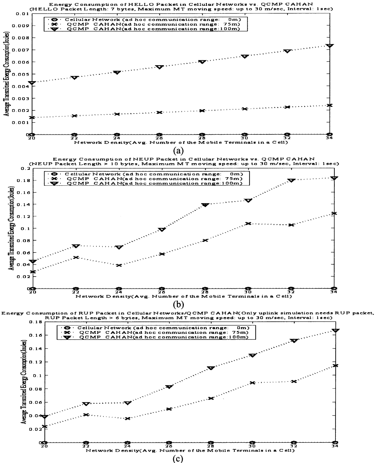
Figure 2.7 Energy consumption of HELLO/NEUP/RUP control packets for system maintenance in QCMP CAHAN: (a) HELLO packets, (b) NEUP packets, (c) RUP packets (RUP packets are needed only if there are source MTs in networks, i.e., RUP packets are needed only in uplink simulation, not downlink simulation).
