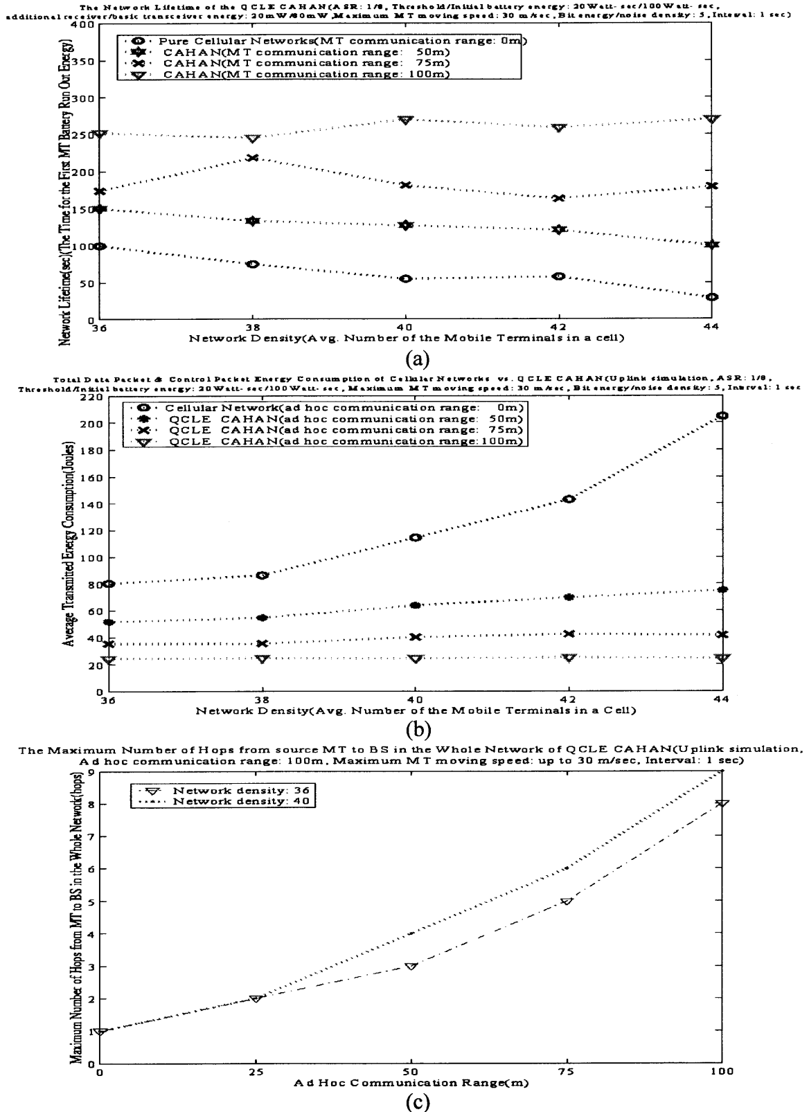
Figure 3.6 QCLE CAHAN with various ad hoc communication range in uplink traffic simulation (a) Network lifetime of QCLE CAHAN, (b) Total data packet and control packet energy consumption, (c) Maximum number of hops from MT to BS in CAHAN.
