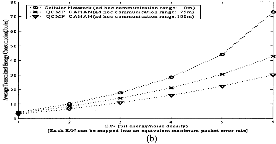
Figure 2.6 Total data packet and control packet energy consumption of cellular networks/QCMP CAHAN with link-cost limitation shortest path: (a) uplink traffic simulation, (b) downlink traffic simulation ( \frac{E}{N} = \gamma , \gamma denote minimum SIR requirement).
