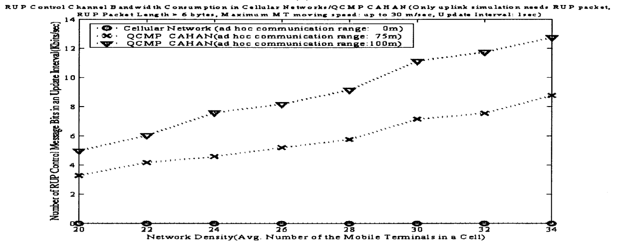
Figure 2.9 HELLO/NEUP/RUP control channel bandwidth consumption for system maintenance in QCMP CAHAN: (a) HELLO packets, (b) NEUP packets, (c) RUP packets (RUP packets are needed only if there are source MTs in networks, i.e., RUP packets are needed only in uplink simulation, not downlink simulation).
