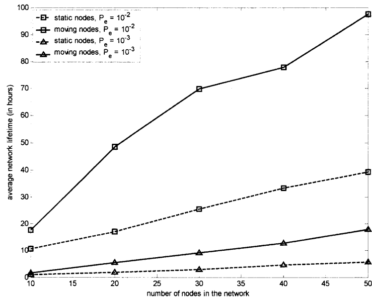
Figure 1.4 Average network lifetime for network with static and moving nodes.
