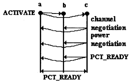
Figure 4.3 PCT initiation procedure.
