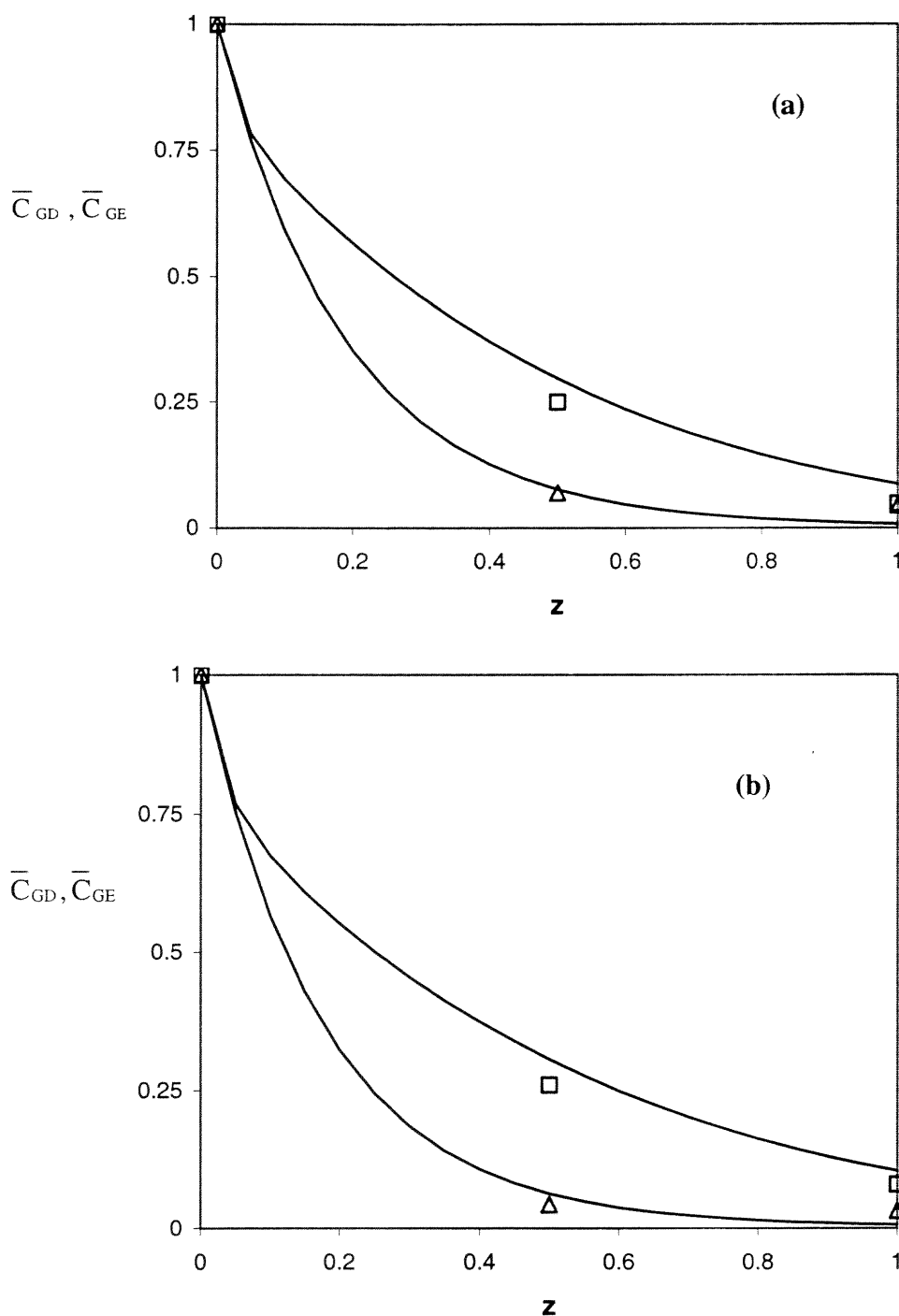
Figure 7.23 Model-predicted dimensionless concentration profiles of o-DCB (curves 1) and ethanol (curves 2) in BTF-II in the air along BTF-II when reaction in the liquid phase is neglected. Symbols represent experimental data. The values for C_{GD_i} ( \text{gm}^{-3} ), C_{GE_i} ( \text{gm}^{-3} ), Q_L ( \text{Lh}^{-1} ), and \tau (min) are correspondingly, 3.14, 1.9, 7.8, and 5.5 in (a), and 0.87, 2.23, 8.35, and 4.2 in (b).
