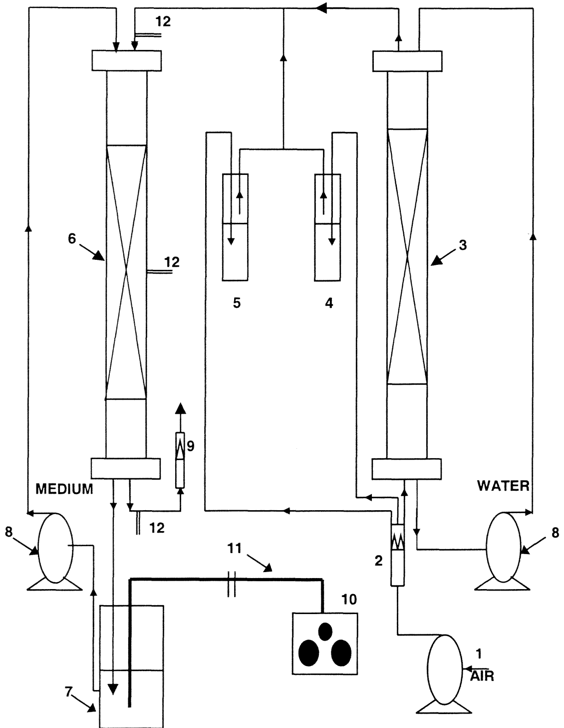
Figure 4.1: Schematic representation of the BTF unit
