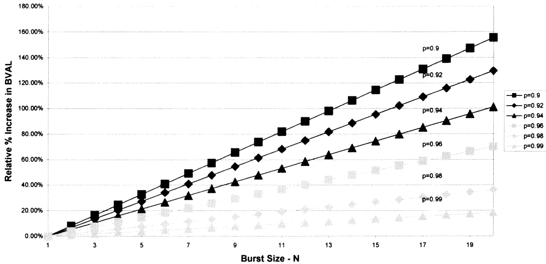
Figure 3.3 Relative % Increase in BVAL as a Function of Burst Size (N) and Packet Completion Rate (p)
