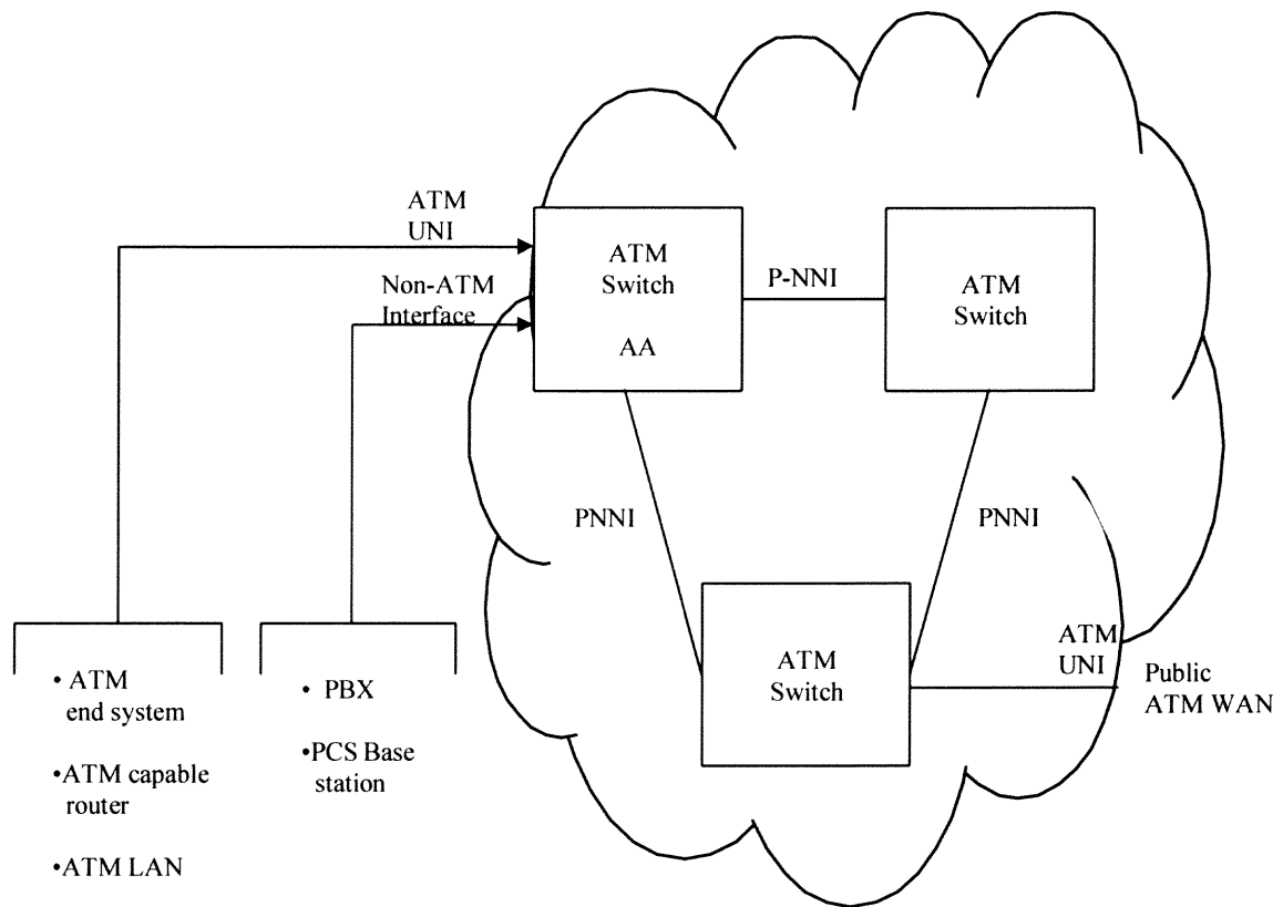
Figure 1.4 ATM Networks
