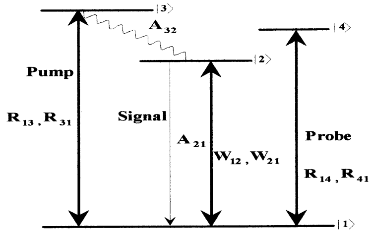
Figure 2.2 Energy State in the quasi-three level system for the study of the nonlinear susceptibility \chi^{(3)} when there is a pump laser present in the system.
