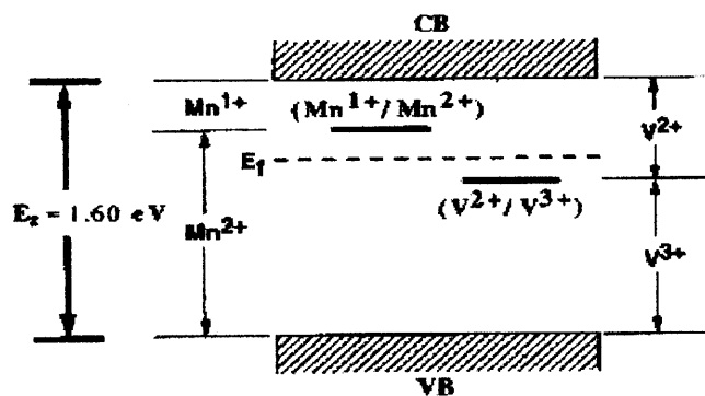
Figure 4.11 Energy level diagram depicting the positions of the ionization levels. For vanadium and Manganese [66].
