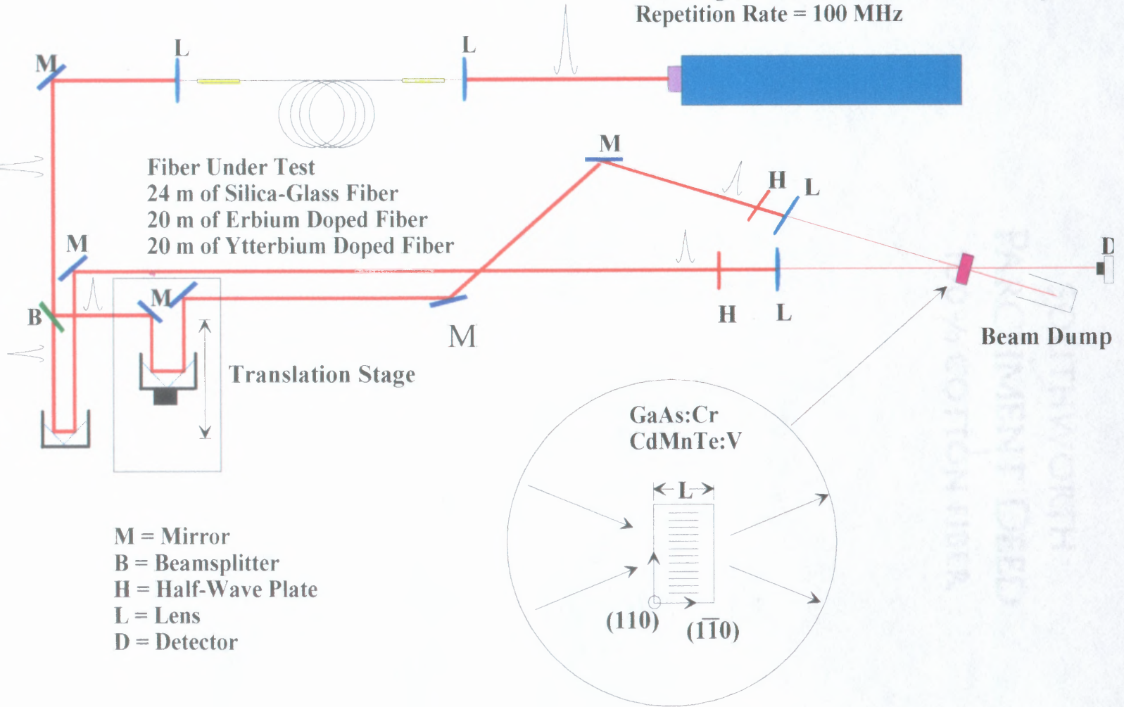
Figure. 5.9 Experimental Setup for TBC-IGA.
