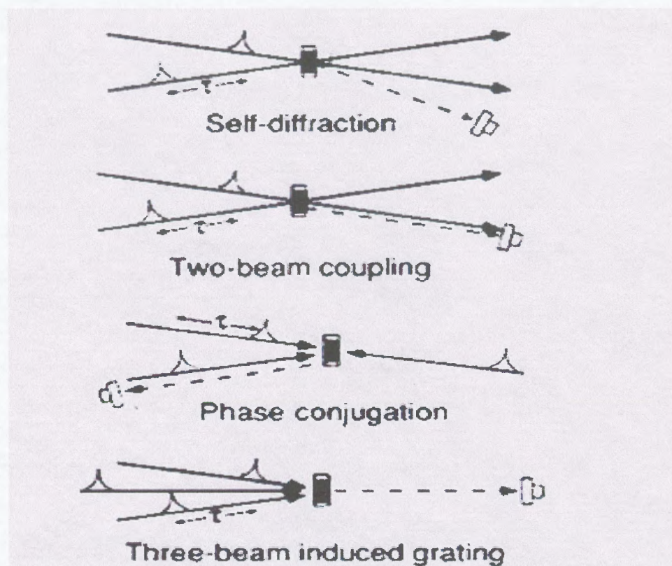
Figure 4.2 Several Geometries for performing IGA experiments [50].
