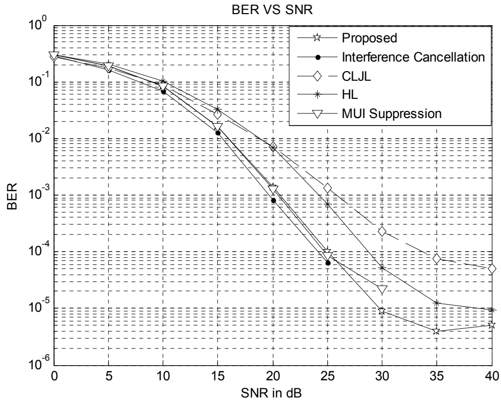
Figure 5.9 BER Vs. SNR for different methods of CFO compensation at uplink of OFDMA.
