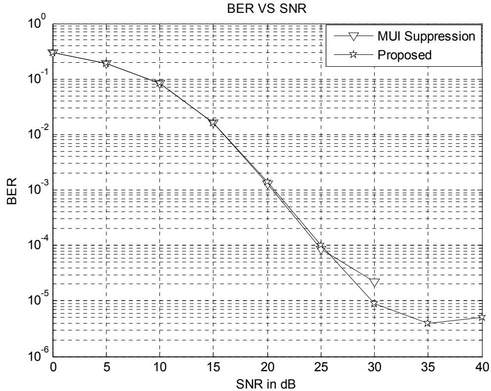
Figure 5.8 BER vs. SNR of MUI suppression by MMSE equalization & proposed method.
