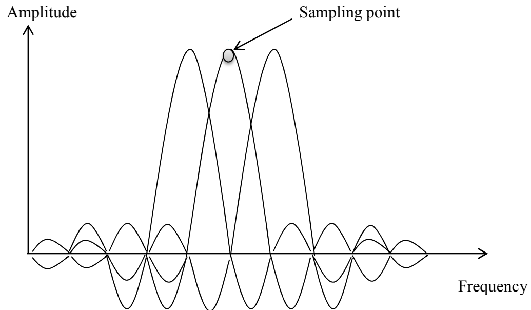
Figure 1.6 OFDM symbol representation using Sinc function.
