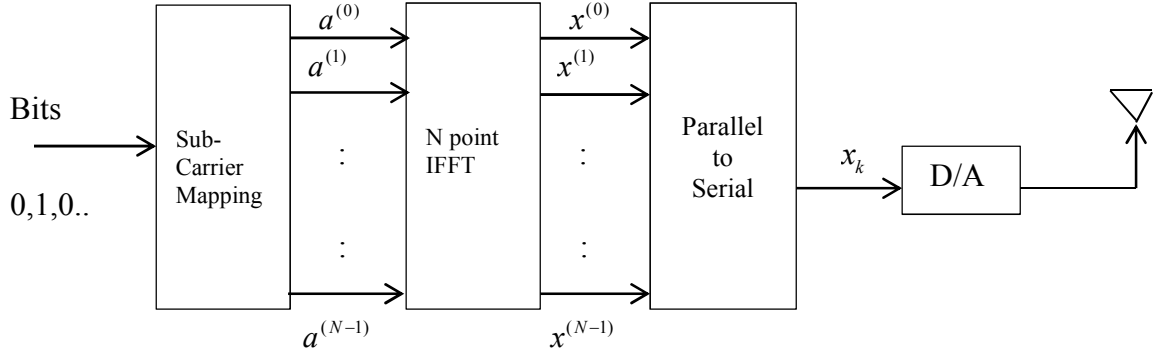
Figure 1.2 OFDM transmitter.
