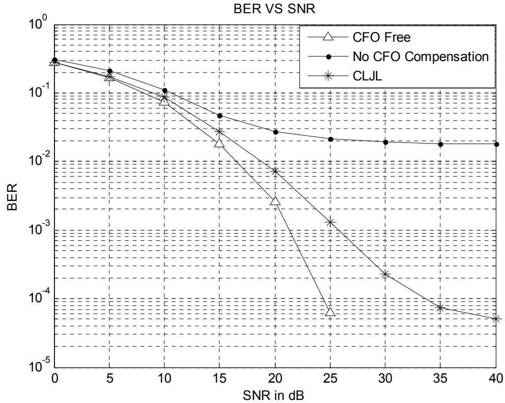
Figure 5.4 BER vs. SNR at Uplink of ODMA by CLJL method.
