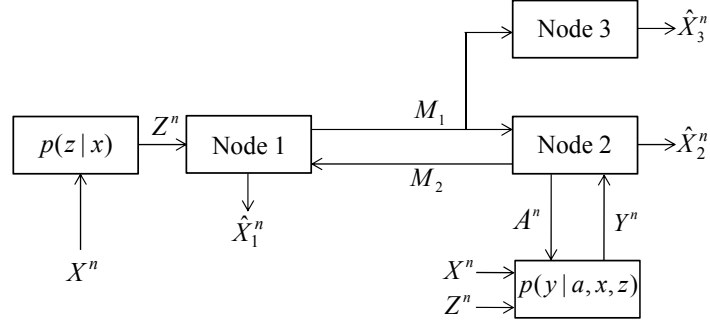
Figure 6.5 Indirect two-way source coding when the side information vending machine may be absent at the recipient of the message from Node 1.
