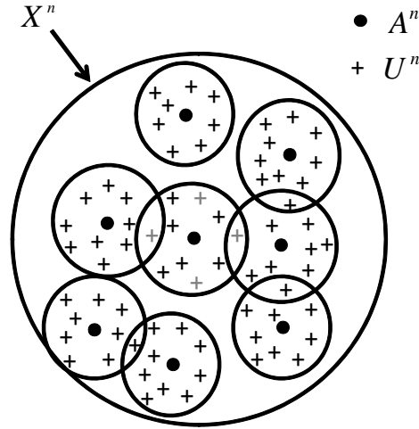
Figure 2.5 Illustration of the optimal strategy for the set-up of Figure 2.4. The picture assumes for simplicity that \mathcal{X} = \mathcal{A} = \mathcal{U} .
