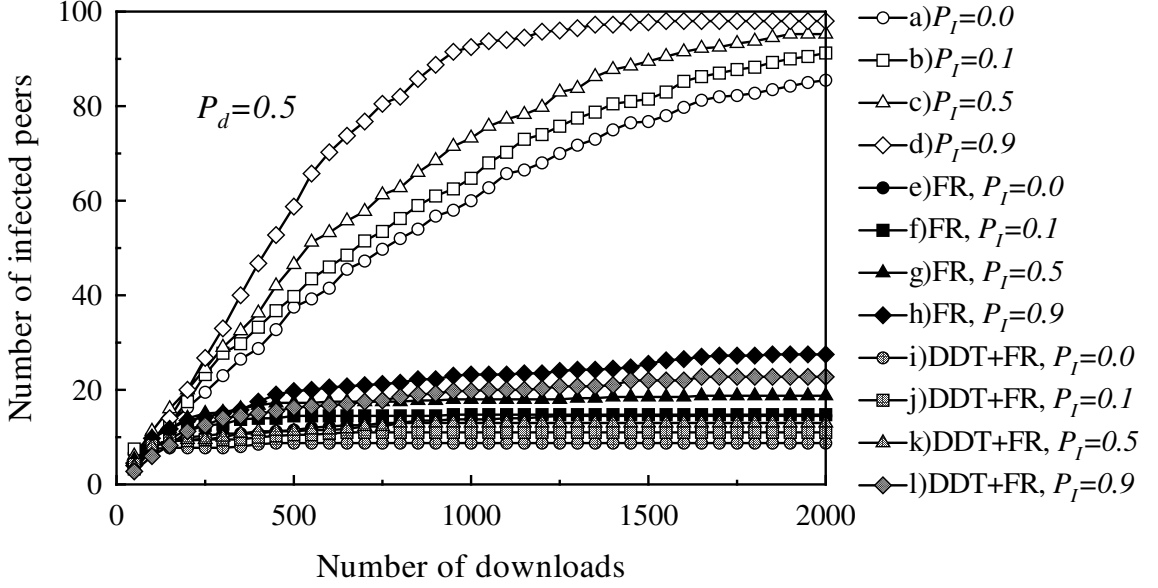
Figure 2.10 Comparison of proliferation of viruses using T_v only and with the proposed scheme.
