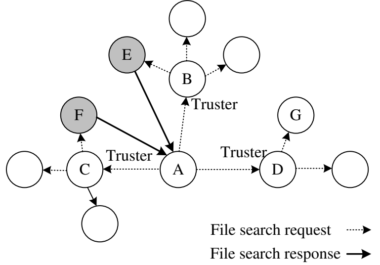
Figure 2.2 File search mechanism, from a peer to its trusters. Trusters forward the search request to their own trustees.
