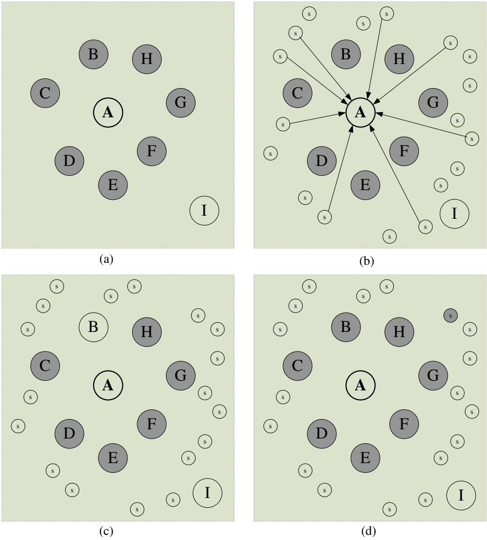
Figure 4.1 Sybil attack.
