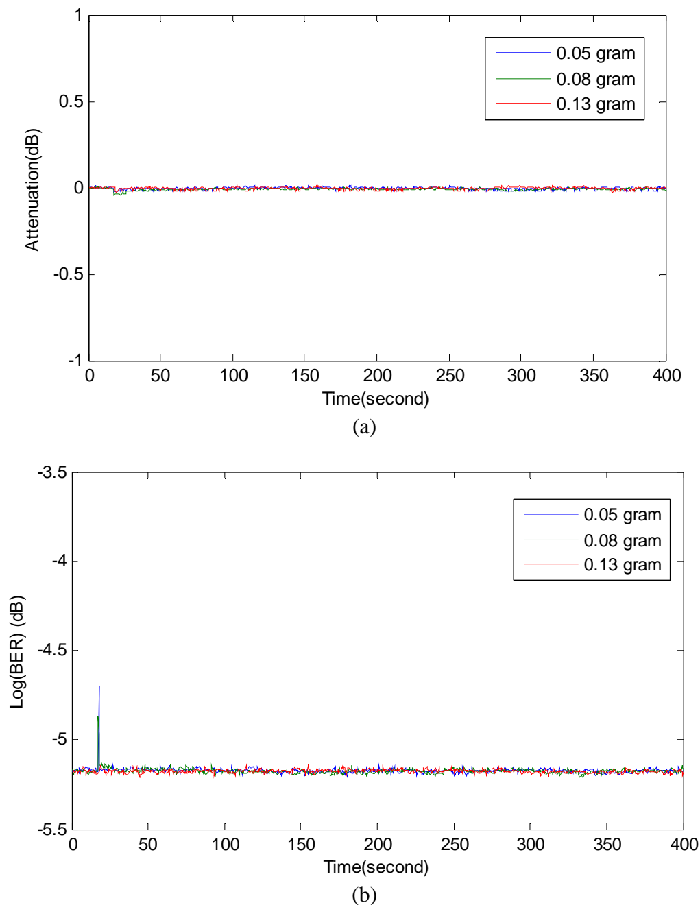
Figure 5.14 (a) Attenuation for different amount of the dust (b) Log(BER) of THz for different amounts of dust.
