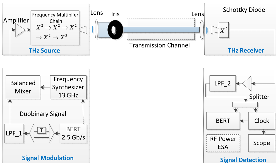
Figure 2.6 Schematic of up converting frequency multiplier chain based 625 GHz transmission link.
