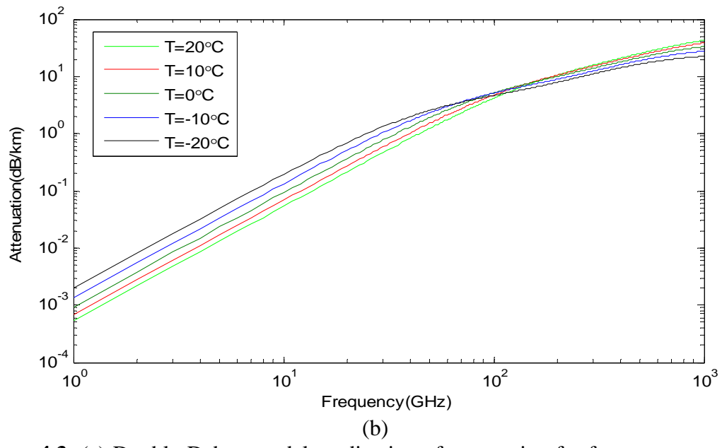
Figure 4.3 (a) Double-Debye model prediction of attenuation for frequency up to 1000 GHz, water content: w=1\text{g/m}^3 and temperature from -20\text{ }^\circ\text{C} to +20\text{ }^\circ\text{C} (b) Logarithmic scale.
