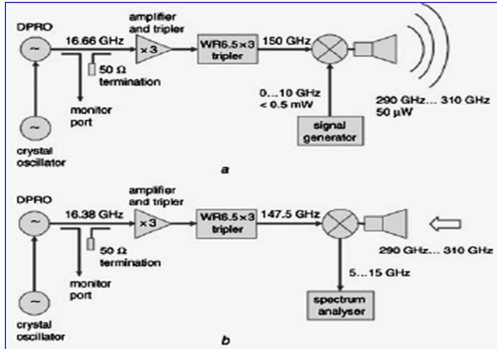
Figure 1.5 Microwave frequency multiplier (a) THz source (b) THz receiver.
