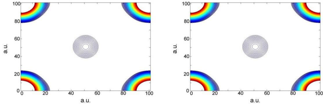
Figure 4.9 Reconstructed electron density on (100) (left) and (110) (right) plane of PZN-PT unit cell from solved \rho(\vec{h}) picture.
