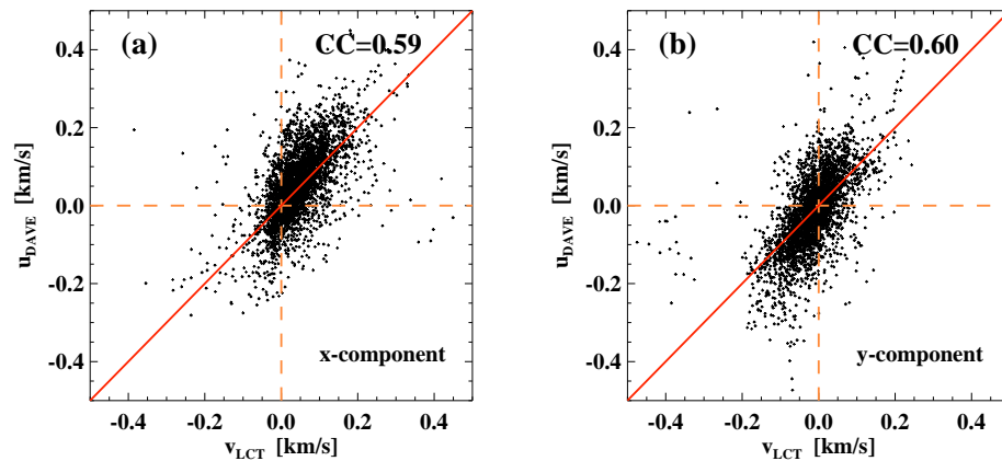
Figure 2.5 u_{\text{DAVE}} vs. v_{\text{LCT}} for their (a) x-components and (b) y-components. The linear CC is specified in each panel. The red line with a slope of 1 is plotted in each panel for purpose of displaying the discrepancy between v_{\text{LCT}} and u_{\text{DAVE}} .
