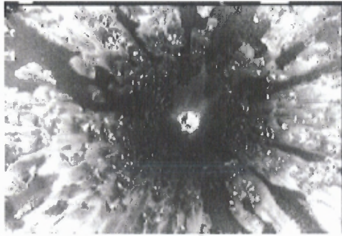
Figure 1.3 Typical M829E3 M256 macro-photo; 360 0 view of 0.9-to 2.0-m erosion band.
