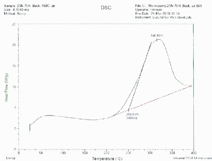
Figure B.14 DSC for annealed CHEAP SWNT substrate from 25% Nitrogen/75% Hydrogen PE-CVD process. Location at Back quartz boat.
