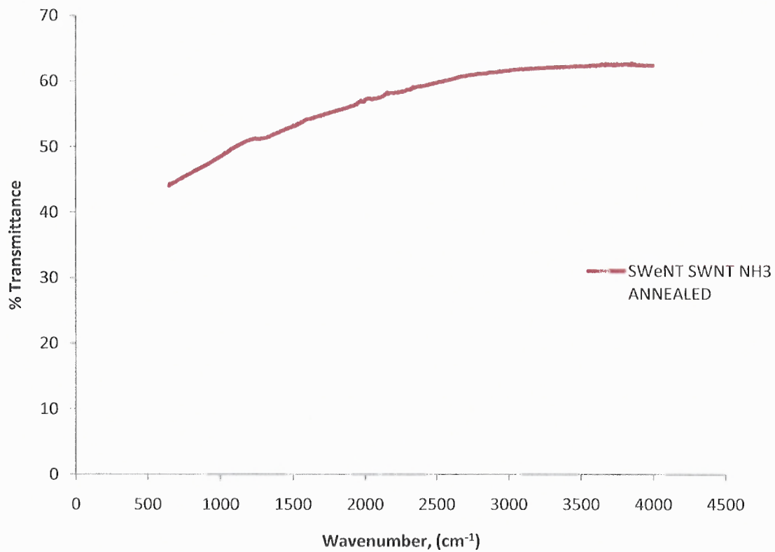
Figure C.2 Sample number 2-SWeNT ammonia annealed, no electrochem.
