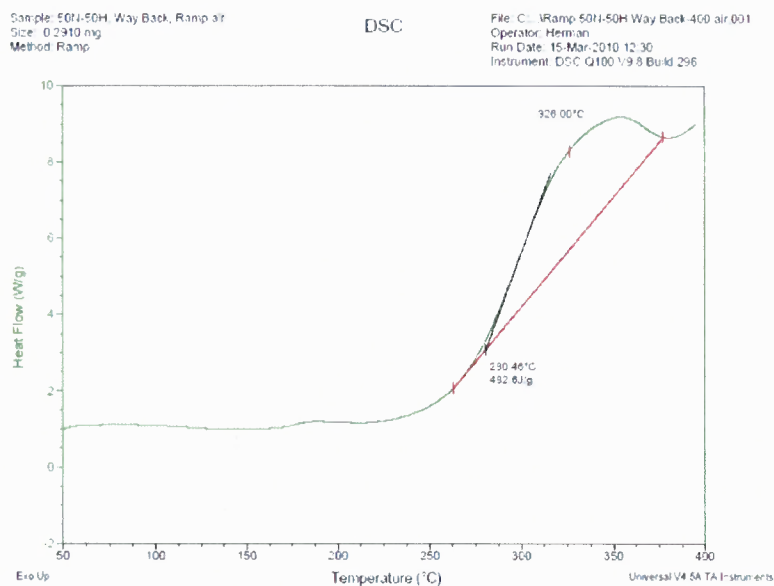
Figure B.11 DSC for not annealed CHEAP SWNT substrate from 50%Nitrogen50% Hydrogen PE-CVD process, Location at Wayback quartz boat.
