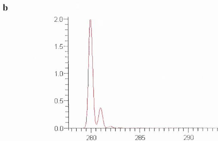
Figure 5.9 Laser desorption time of flight mass spectrum in the (a) 100 to 300 amu and (b) 280 amu region region from the electrochemically functionalized SWNT nanopaper made from Cheap SWNTs.
