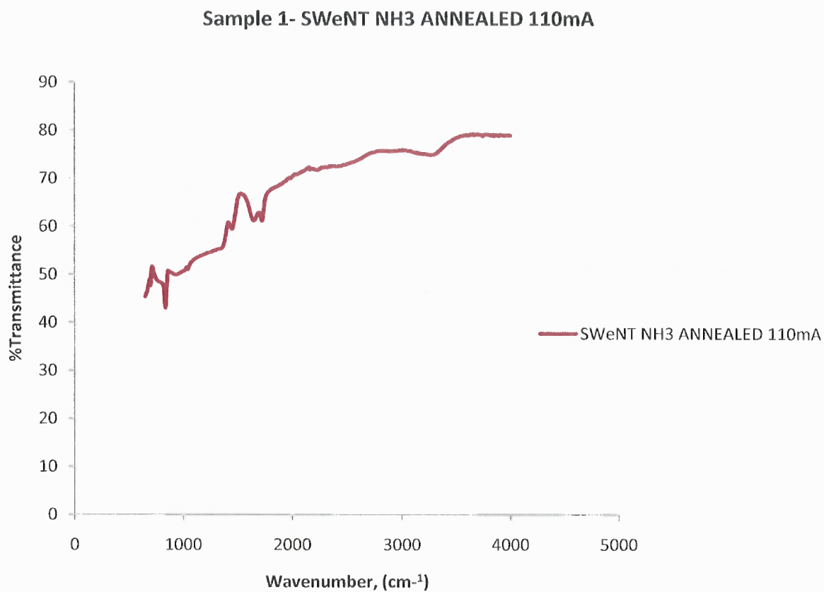
Figure C.1 Sample number 1-SWeNT ammonia annealed , electrochem with 110mA.
