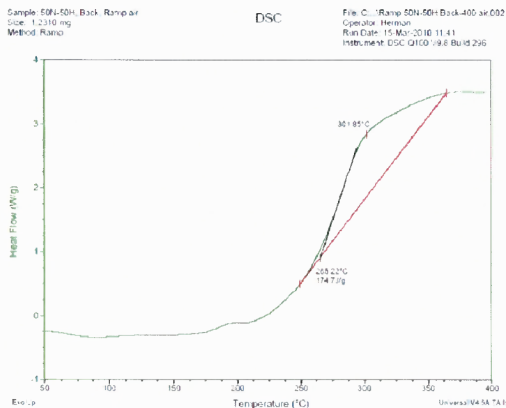
Figure B.10 DSC for not annealed CHEAP SWNT substrate from 50% Nitrogen 50% Hydrogen PE-CVD process. Location at Back quartz boat
