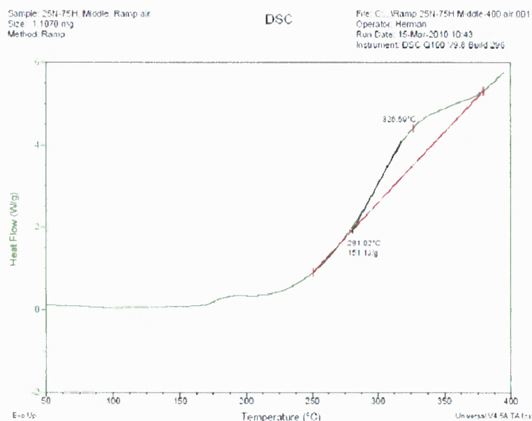
Figure B.9 DSC for not annealed CHEAP SWNT substrate from 25% Nitrogen 75% Hydrogen PE-CVD process. Location at Middle quartz boat.
