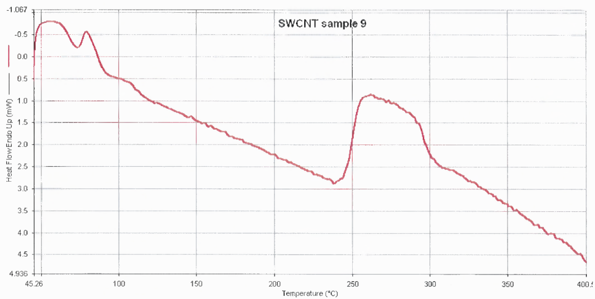
Figure A.9 DSC of CHEAP SWNT, 5%PS, 1Ma, 1,495V, NH 3 Annealed.
