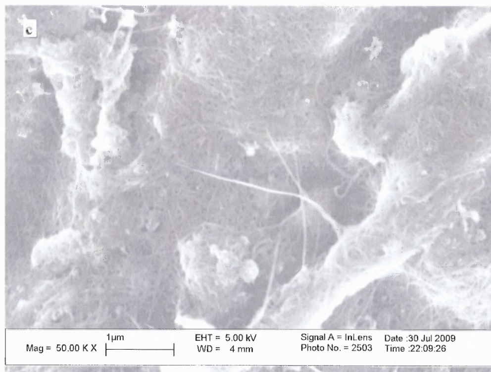
Figure 4.4 SEM images of some of the CHEAP SWNT bundles from sample obtained from Cheap Tubes Inc used in this study. (a) Surface of pristine nanotube sheet. Prepared from these SWNT, (b) Surface of polystyrene infiltrated nanotube sheet (c) Surface of nanotube sheet, showing a thin coating of PS polymer indicating sizable infiltration had occurred.
