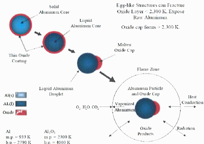
Figure 2.2 Aluminum combustion mechanism.
