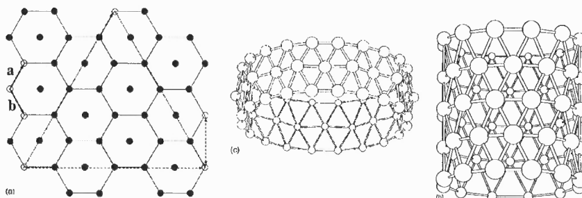
Figure 2.9 (a) Construction of boron tubes from 2D hexagonal boron layers. The fat dashed lines mark the direction of the finite horizontal cut, as well as the direction of the infinite vertical cuts. (b) tubular B 60 cluster composed of five 12 membered rings. (c) B 60 cluster composed of three 20 membered rings and characterized by a buckled surface.
