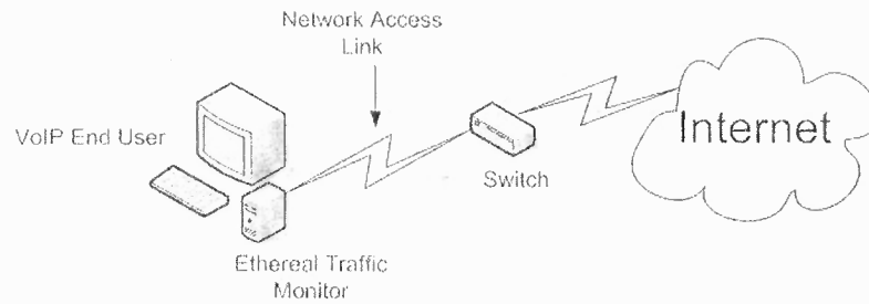
Figure 3.1 Traffic Monitoring System.
