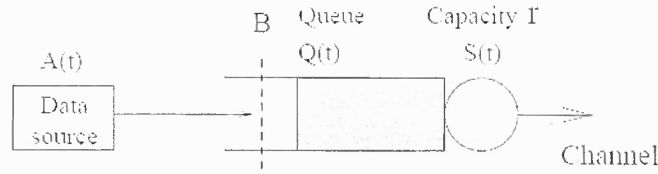
Figure 9.1 A general queueing system.
