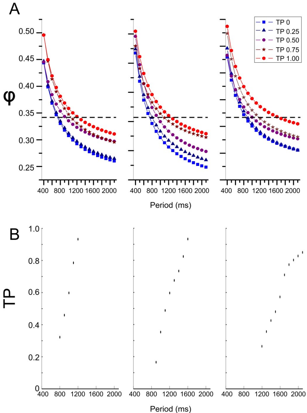
Figure 5.11 Predicting TP value required to maintain a specific (0.34) \phi constancy at constant duty cycle and fixed G_{max} . A. Using the sampled data, the LP \phi constancy was fixed to 0.34 (grey dotted line) and fixed G_{max} , and plotted each of the five different TP values: 0 (royal blue), 0.25 (dark blue), 0.50 (purple), 0.75 (burgundy) and 1.00 (red). B. Using the data plotted in A, the values of TP were predicted (black dots) at each period required to maintain a LP \phi constancy of 0.34. At each of the different values of G_{max} , across certain periods it would be impossible given the range of TP value to maintain a LP \phi constancy to 0.34.
