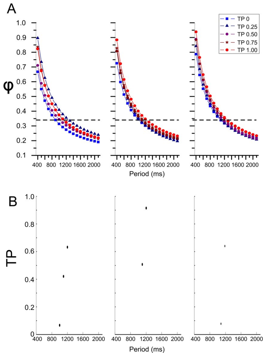
Figure 5.12 Predicting TP value required to maintain a specific (0.34) \phi constancy at duration of 300ms and fixed G_{max} . A. The sampled data was plotted, and the LP \phi constancy was fixed to 0.34 (grey dotted line) and fixed G_{max} , and plotted each of the five different TP values: 0 (royal blue), 0.25 (dark blue), 0.50 (purple), 0.75 (burgundy) and 1.00 (red). B. Using the data plotted in A, the values of TP predicted (black dots) at each period to maintain a LP \phi constancy of 0.34. With a constant duration of 300ms across all periods, it is very difficult at each period with a fixed a LP \phi constancy to 0.34. At each of the different values of G_{max} , across certain periods it would be impossible given the range of TP value to maintain a LP \phi constancy to 0.34.
