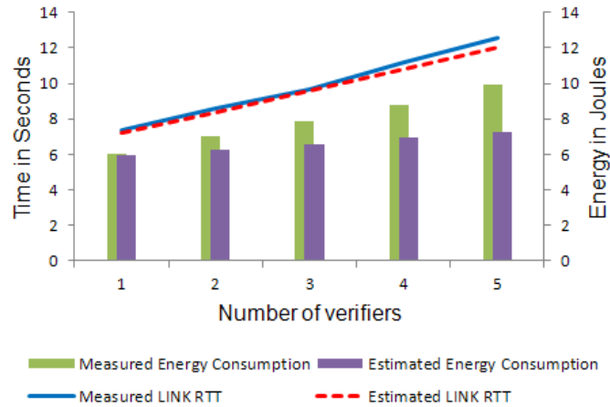
Figure 5.11 LINK RTT and total energy consumed by claimer per claim function of the number of verifiers.
