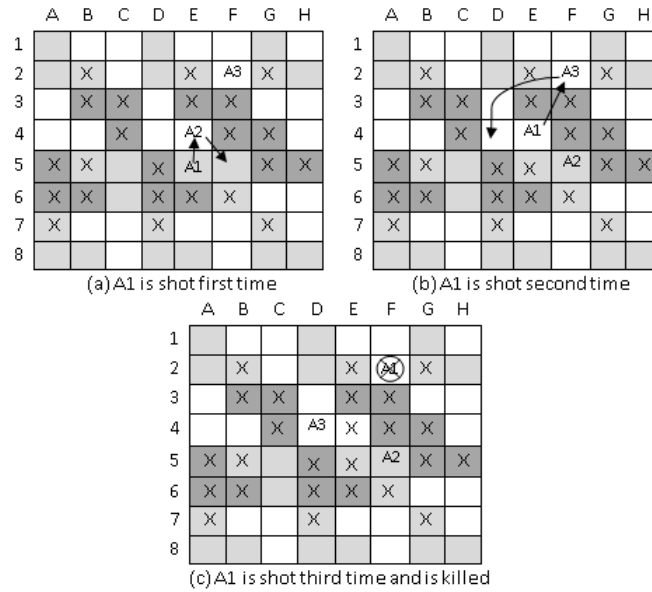
Figure 6.5 Progressive Movement strategy: Example of CGS moving the alien to the closest unpopular region.
