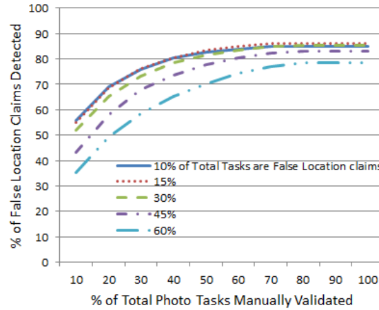
Figure 4.3 ILR performance as function of the percentage of photos manually validated in phase 1. Each curve represents a different percentage of photos with fake locations.
