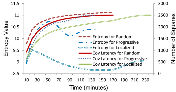
Figure 6.8 The entropy and latency over time for the three alien movement strategies in BH3 scenario.
