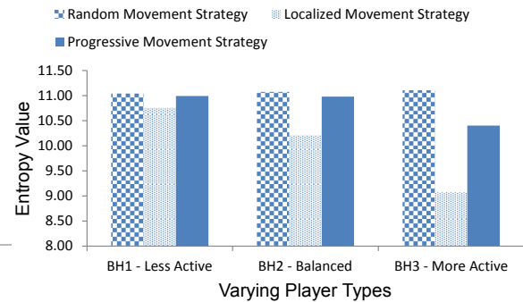
Figure 6.7 Entropy of the area coverage for the three alien movement strategies.
