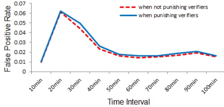
Figure 5.9 False positive rate over time when punishing and not punishing colluding verifiers. All parameters are the same as in Figure 5.8.
