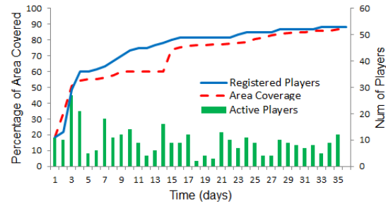
Figure 6.12 Impact of the number of registered players and the number of active players on area coverage over time in the game.
