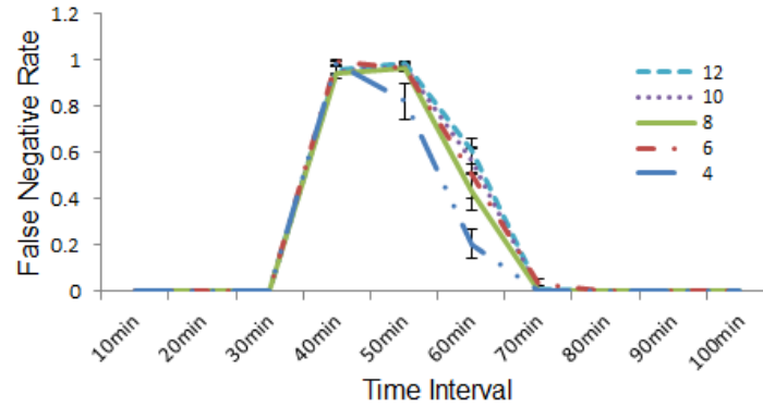
Figure 5.7 False negative rate over time for colluding users. Each curve is for a different colluding group size. Only 50% of the colluding users participate in each verification, thus maximizing their chances to remain undetected. The claim generation rate is 1 per minute and the average speed is 1m/s. Error bars for 95% confidence intervals are plotted.
