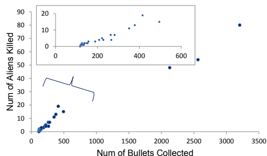
Figure 6.17 Correlation between number of bullets and aliens killed. The calculated correlation value is 0.98 (high positive correlation).
