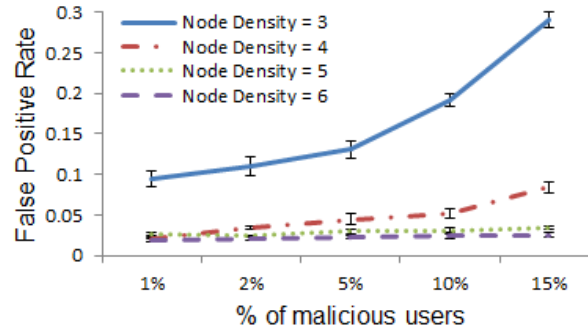
Figure 5.4 False positive rate as a function of the percentage of malicious verifiers for different node densities. The claim generation rate is 1 per minute and average speed is 1m/s. Error bars for 95% confidence intervals are plotted.
