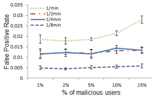
Figure 5.5 False positive rate as a function of the percentage of malicious verifiers for different claim generation rates. The average speed is 1m/s. Error bars for 95% confidence intervals are plotted.
