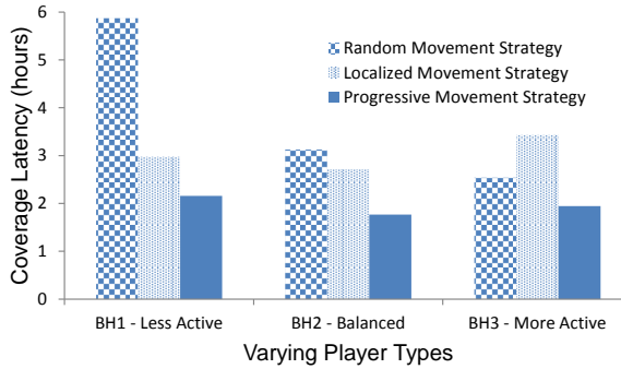
Figure 6.6 The area coverage latency of the three alien movement strategies.
