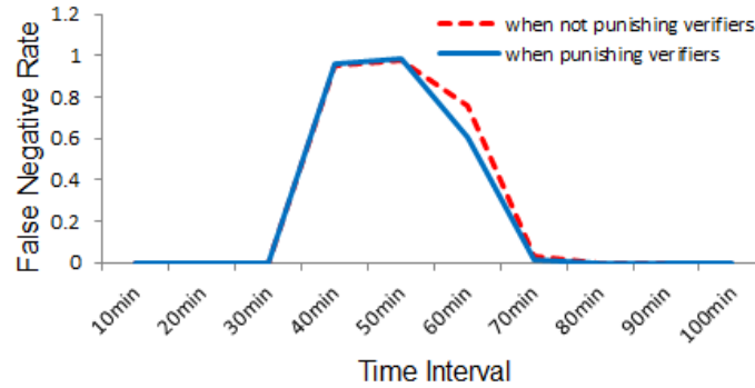
Figure 5.8 False negative rate over time when punishing and not punishing colluding verifiers. The size of the colluding group is 12, and 50% of these users participate in each verification. The claim generation rate is 1 per minute and the average speed is 1m/s.
