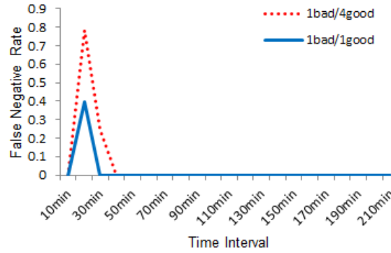
Figure 5.2 False negative rate over time for individual malicious claimers with mixed behavior. The claim generation rate is 1 per minute, 15% of the users are malicious, and average speed is 1m/s.
