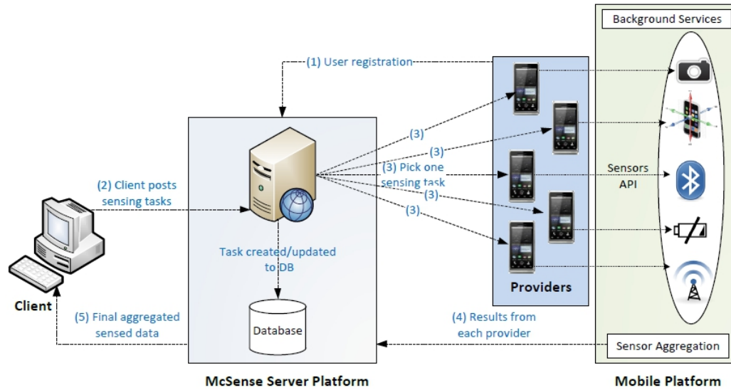
Figure 3.1 McSense Architecture.
