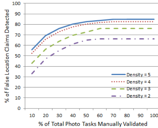
Figure 4.4 ILR performance as function of the percentage of photos manually validated in phase 1. Each curve represents a different network density represented as average number of neighbors per node.
