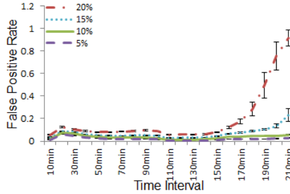
Figure 5.6 False positive rate over time for different percentages of malicious verifiers. The claim generation rate is 1 per minute and the average speed is 1m/s. Error bars for 95% confidence intervals are plotted.
