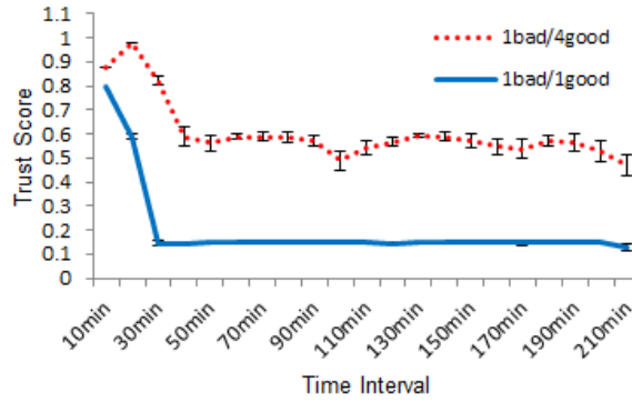
Figure 5.3 Trust score of malicious users with mixed behavior over time. The claim generation rate is 1 per minute, 15% of the users are malicious, and average speed is 1m/s. Error bars for 95% confidence intervals are plotted.
