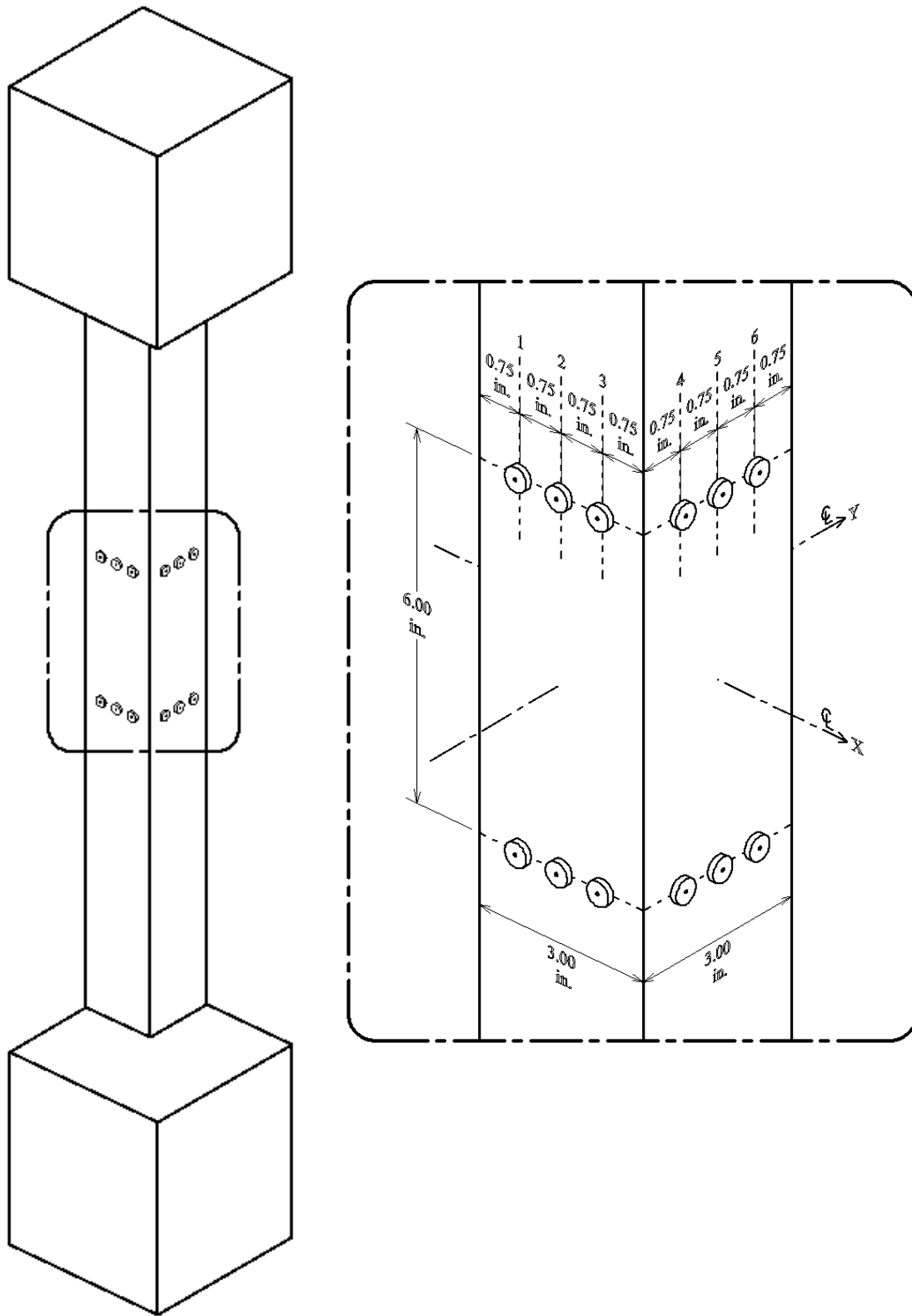
Figure 3.5 Arrangement of mechanical strain gauges.
