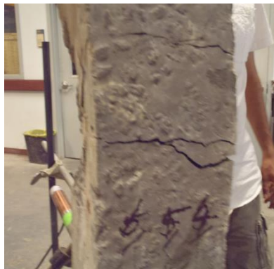
Tension face
