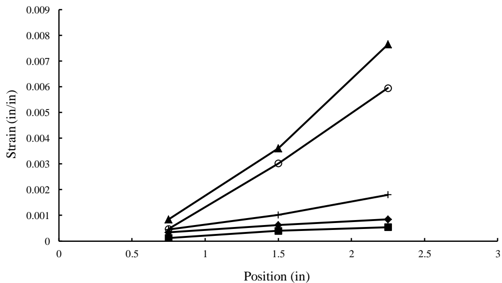
Figure 3.15 Typical strain-position curve for column C5 in X direction.
