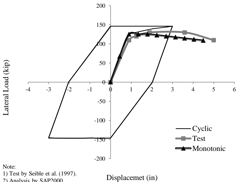
Figure 2.20 Load-displacement response of column #2 without CFRP.
